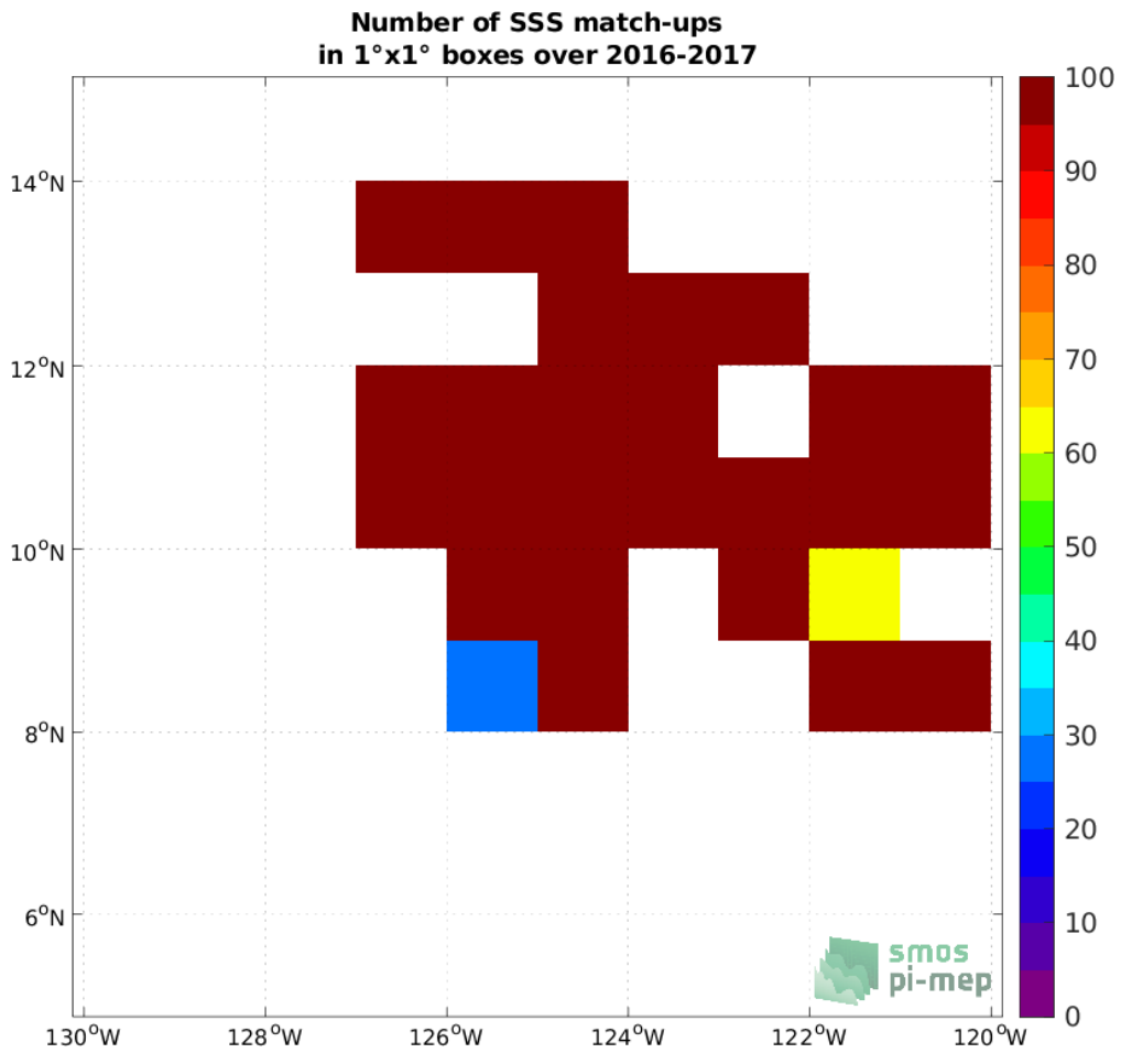
Figure 4: Number of SSS match-ups between Waveglider (SPURS 2) SSS and the SMAP SSS L2 v5 (RSS) SSS product for the SPURS 2 Pi-MEP region over 1°x1° boxes and for the full satellite product period.
