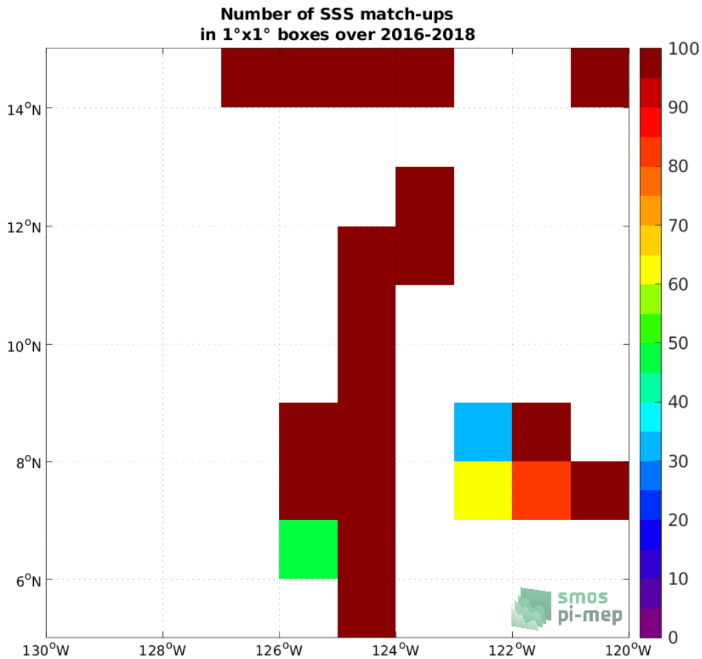
Figure 4: Number of SSS match-ups between TSG (SAMOS) SSS and the SMAP SSS L2 v5 (RSS) SSS product for the SPURS 2 Pi-MEP region over 1°x1° boxes and for the full satellite product period.
