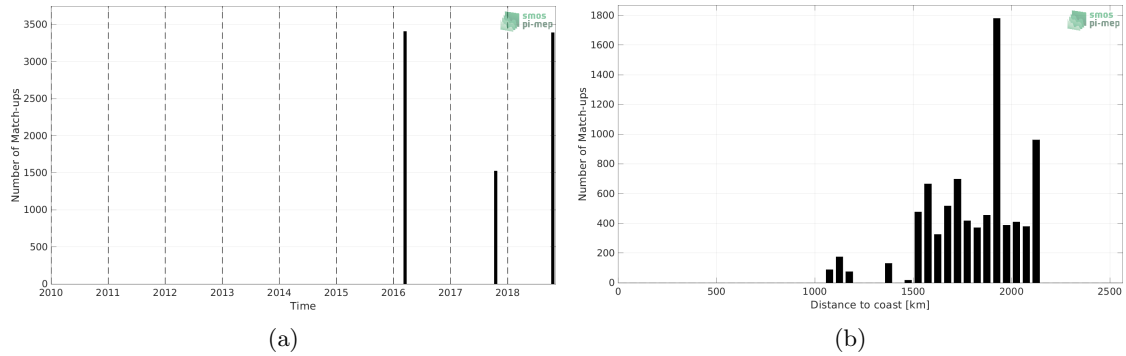
Figure 1: Number of match-ups between TSG (SAMOS) and SMAP SSS L2 v5 (RSS) SSS as a function of time (a) and as function of the distance to coast (b) over the SPURS 2 Pi-MEP region and for the full satellite product period.
