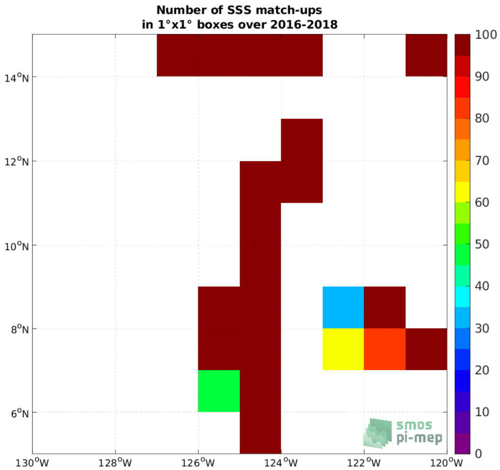
Figure 4: Number of SSS match-ups between TSG (SAMOS) SSS and the SMAP SSS L2 v5 (RSS) SSS product for the SPURS 2 Pi-MEP region over 1^\circ \times 1^\circ boxes and for the full satellite product period.
