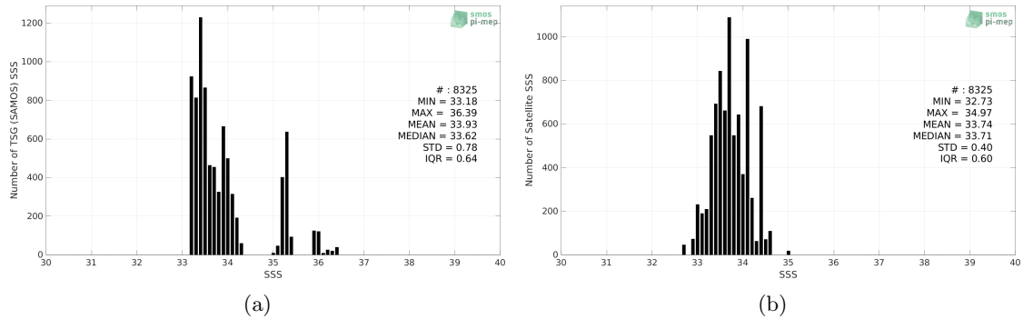
Figure 2: Histograms of SSS from TSG (SAMOS) (a) and SMAP SSS L2 v5 (RSS) (b) considering all match-up pairs per bins of 0.1 over the SPURS 2 Pi-MEP region and for the full satellite product period.
