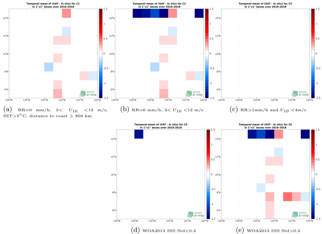
Figure 12: Temporal mean gridded over spatial boxes of size 1^\circ \times 1^\circ of \Delta SSS (SMAP SSS L2 v5 (RSS) - TSG (SAMOS)) for 5 different subdatasets corresponding to:RR=0 mm/h, 3 < U_{10} < 12 m/s, SST >5^\circ C, distance to coast > 800 km (a), RR=0 mm/h, 3 < U_{10} < 12 m/s (b), RR >1 mm/h and U_{10} < 4 m/s (c), WOA2013 SSS Std <0.2 (d), WOA2013 SSS Std >0.2 (e).
