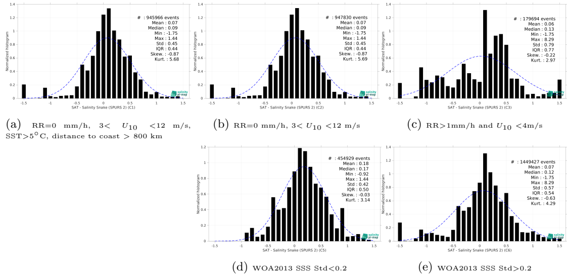
Figure 13: Normalized histogram of \Delta SSS (SMAP SSS L2 v5 (RSS) - Salinity Snake (SPURS 2)) for 5 different subdatasets corresponding to: RR=0 mm/h, 3 < U_{10} < 12 m/s, SST>5°C, distance to coast > 800 km (a), RR=0 mm/h, 3 < U_{10} < 12 m/s (b), RR>1mm/h and U_{10} < 4 m/s (c), WOA2013 SSS Std<0.2 (d), WOA2013 SSS Std>0.2 (e).
