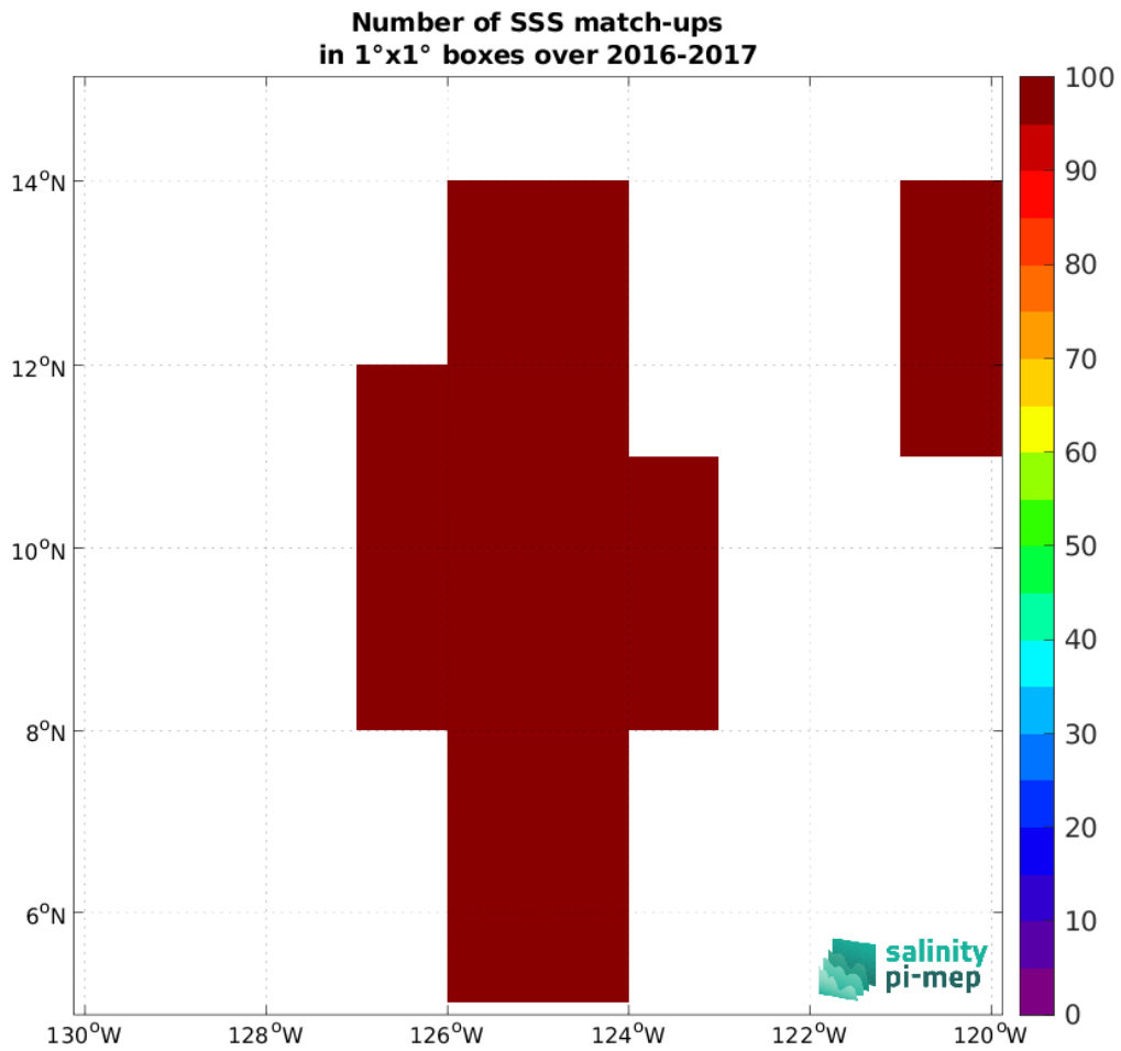
Figure 4: Number of SSS match-ups between Salinity Snake (SPURS 2) SSS and the SMAP SSS L2 v5 (RSS) SSS product for the SPURS 2 Pi-MEP region over 1^\circ \times 1^\circ boxes and for the full satellite product period.
