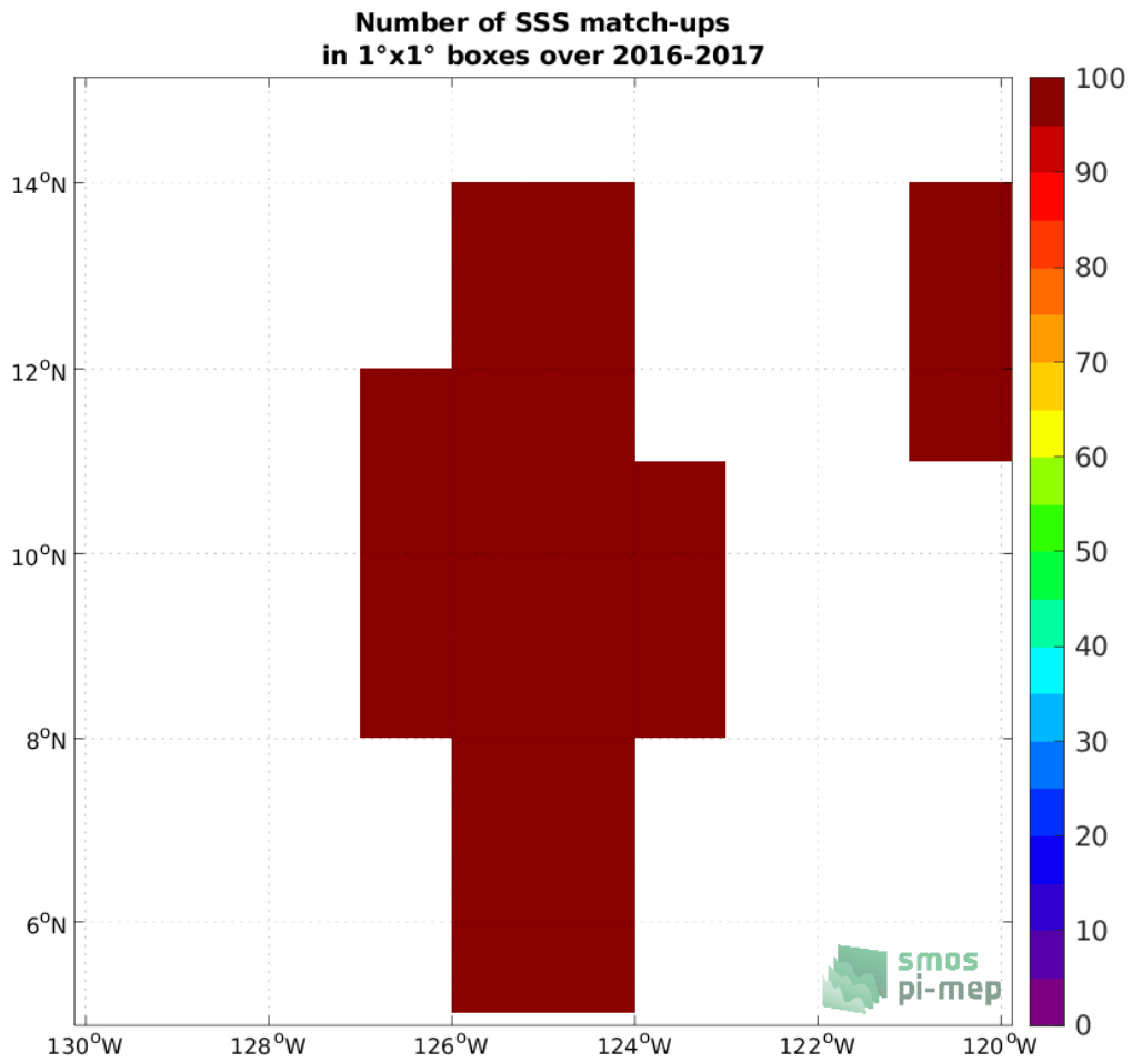
Figure 4: Number of SSS match-ups between Salinity Snake (SPURS 2) SSS and the SMAP SSS L2 v5 (RSS) SSS product for the SPURS 2 Pi-MEP region over 1°x1° boxes and for the full satellite product period.
