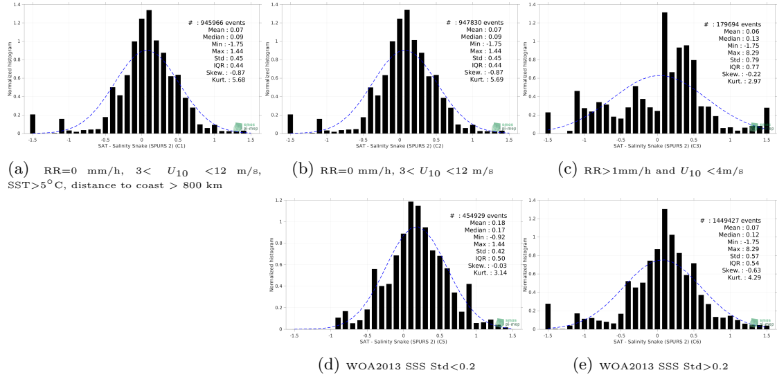
Figure 13: Normalized histogram of \Delta SSS (SMAP SSS L2 v5 (RSS) - Salinity Snake (SPURS 2)) for 5 different subdatasets corresponding to: RR=0 mm/h, 3 < U_{10} < 12 m/s, SST > 5°C, distance to coast > 800 km (a), RR=0 mm/h, 3 < U_{10} < 12 m/s (b), RR > 1mm/h and U_{10} < 4 m/s (c), WOA2013 SSS Std < 0.2 (d), WOA2013 SSS Std > 0.2 (e).
