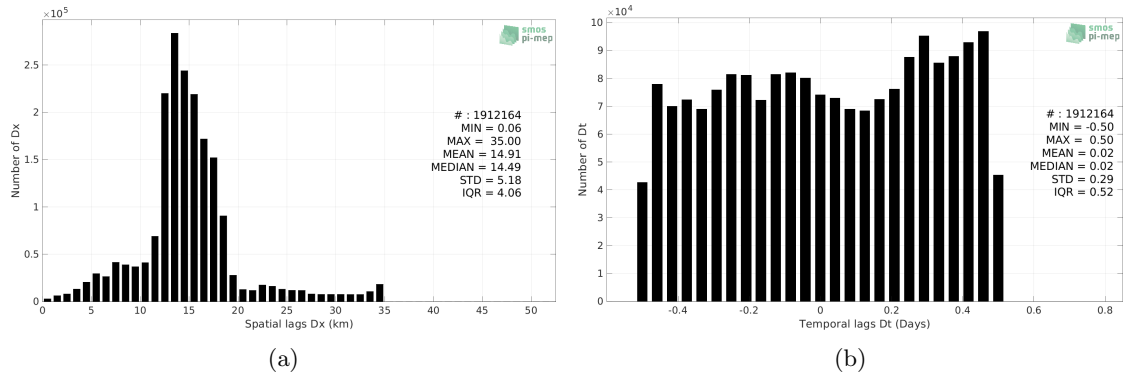
Figure 5: Histograms of the spatial (a) and temporal (b) lags between the location/time of the Salinity Snake (SPURS 2) measurement and the date of the corresponding SMAP SSS L2 v5 (RSS) SSS pixel.
