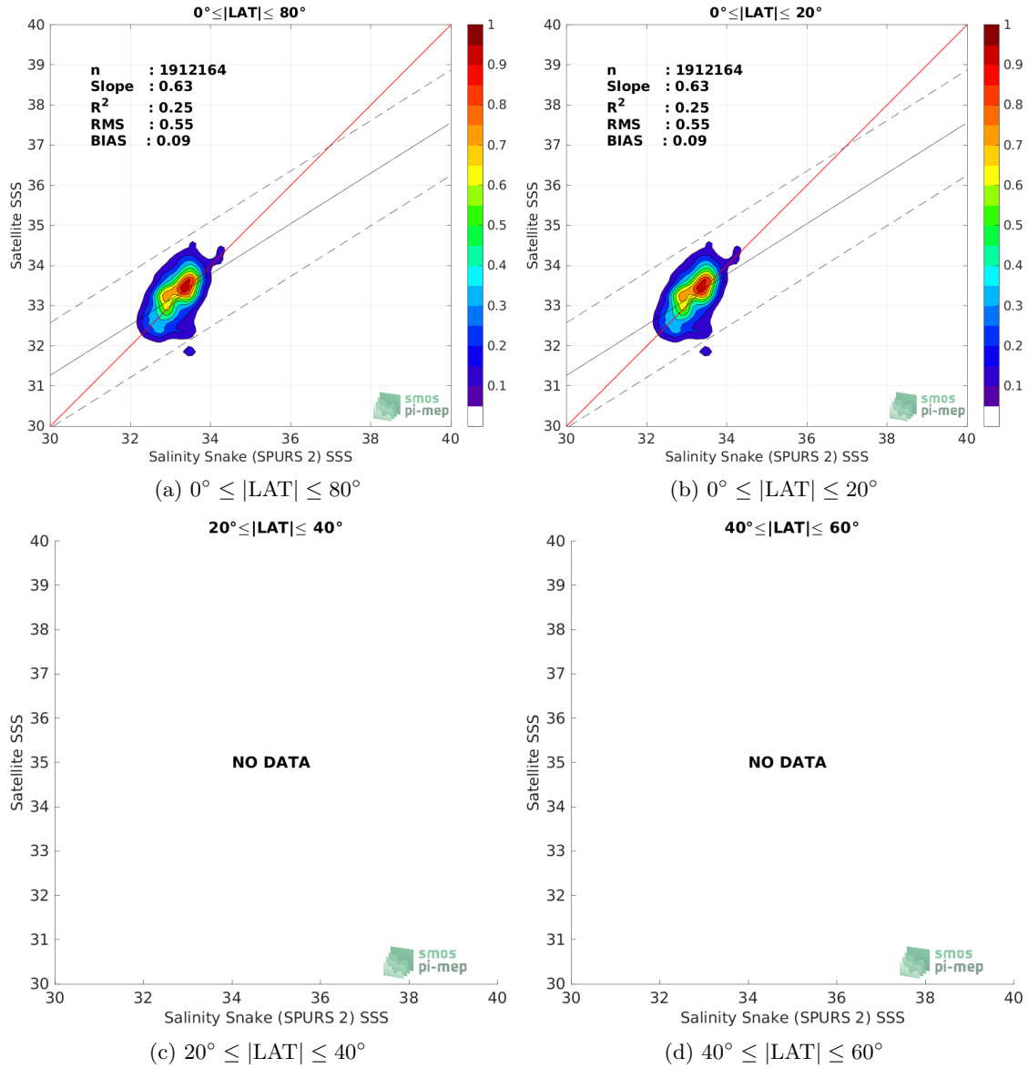
Figure 9: Contour maps of the concentration of SMAP SSS L2 v5 (RSS) SSS (y-axis) versus Salinity Snake (SPURS 2) SSS (x-axis) at match-up pairs for different latitude bands. For each plot, the red line shows x=y . The black thin and dashed lines indicate a linear fit through the data cloud and the \pm 95\% confidence levels, respectively. The number match-up pairs n , the slope and R^2 coefficient of the linear fit, the root mean square (RMS) and the mean bias between satellite and in situ data are indicated for each latitude band in each plots.
