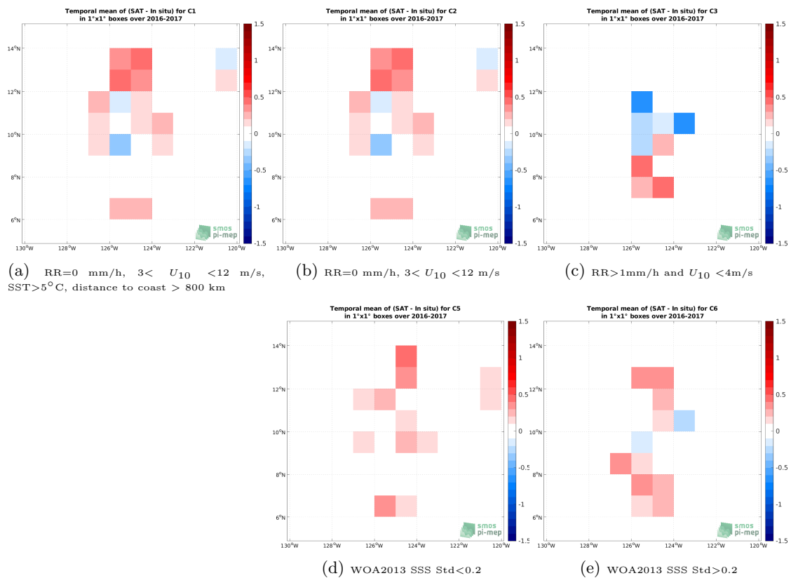
Figure 12: Temporal mean gridded over spatial boxes of size 1^\circ \times 1^\circ of \Delta SSS (SMAP SSS L2 v5 (RSS) - Salinity Snake (SPURS 2)) for 5 different subdatasets corresponding to:RR=0 mm/h, 3 < U_{10} < 12 m/s, SST >5^\circ C, distance to coast > 800 km (a), RR=0 mm/h, 3 < U_{10} < 12 m/s (b), RR >1 mm/h and U_{10} < 4 m/s (c), WOA2013 SSS Std <0.2 (d), WOA2013 SSS Std >0.2 (e).
