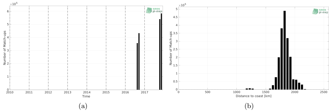
Figure 1: Number of match-ups between Salinity Snake (SPURS 2) and SMAP SSS L2 v5 (RSS) SSS as a function of time (a) and as function of the distance to coast (b) over the SPURS 2 Pi-MEP region and for the full satellite product period.
