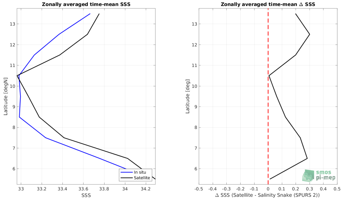
Figure 8: Left panel: Zonal mean SSS from SMAP SSS L2 v5 (RSS) satellite product (black) and from Salinity Snake (SPURS 2) (blue). Right panel: Zonal mean of \Delta SSS (Satellite - Salinity Snake (SPURS 2)) for all the collected Pi-MEP match-up pairs estimated over the full satellite product period.
