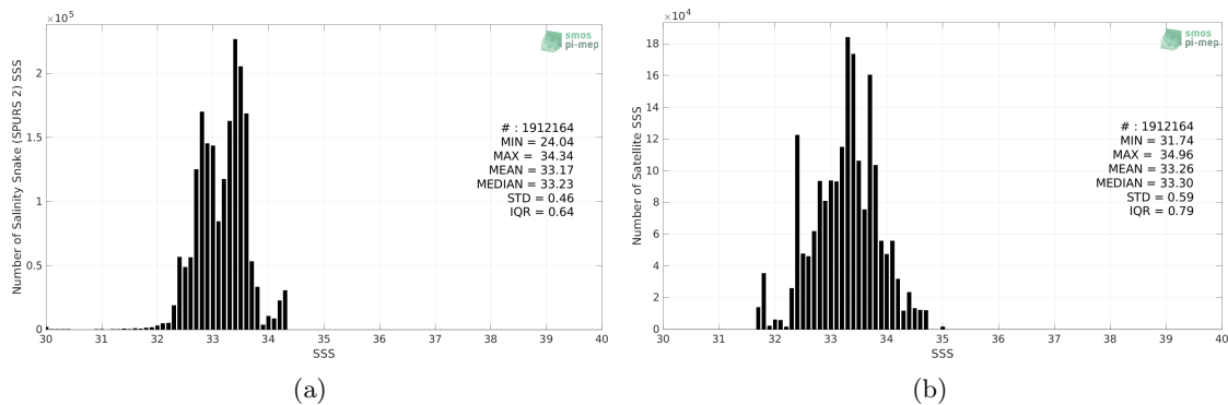
Figure 2: Histograms of SSS from Salinity Snake (SPURS 2) (a) and SMAP SSS L2 v5 (RSS) (b) considering all match-up pairs per bins of 0.1 over the SPURS 2 Pi-MEP region and for the full satellite product period.
