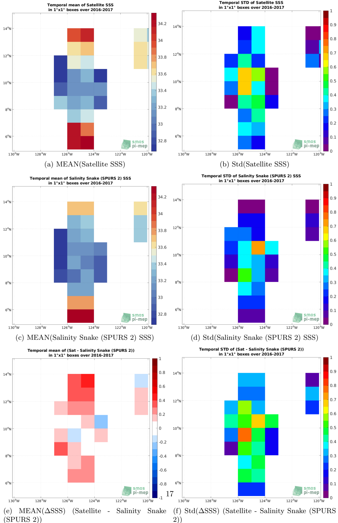
Figure 6: Temporal mean (left) and Std (right) of SSS from SMAP SSS L2 v5 (RSS) (top), Salinity Snake (SPURS 2) (middle), and of \Delta SSS (Satellite - Salinity Snake (SPURS 2)). Only match-up pairs are used to generate these maps.
