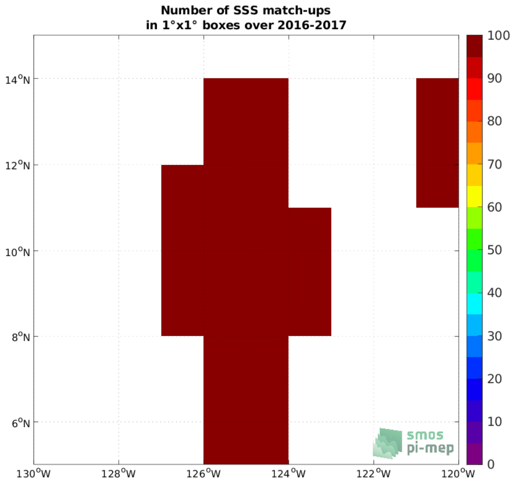
Figure 3: Number of SSS match-ups between Salinity Snake SSS and the SMAP SSS L2 v5 (RSS) SSS product for the SPURS 2 Pi-MEP region over 1°x1° boxes and for the full satellite product period.
