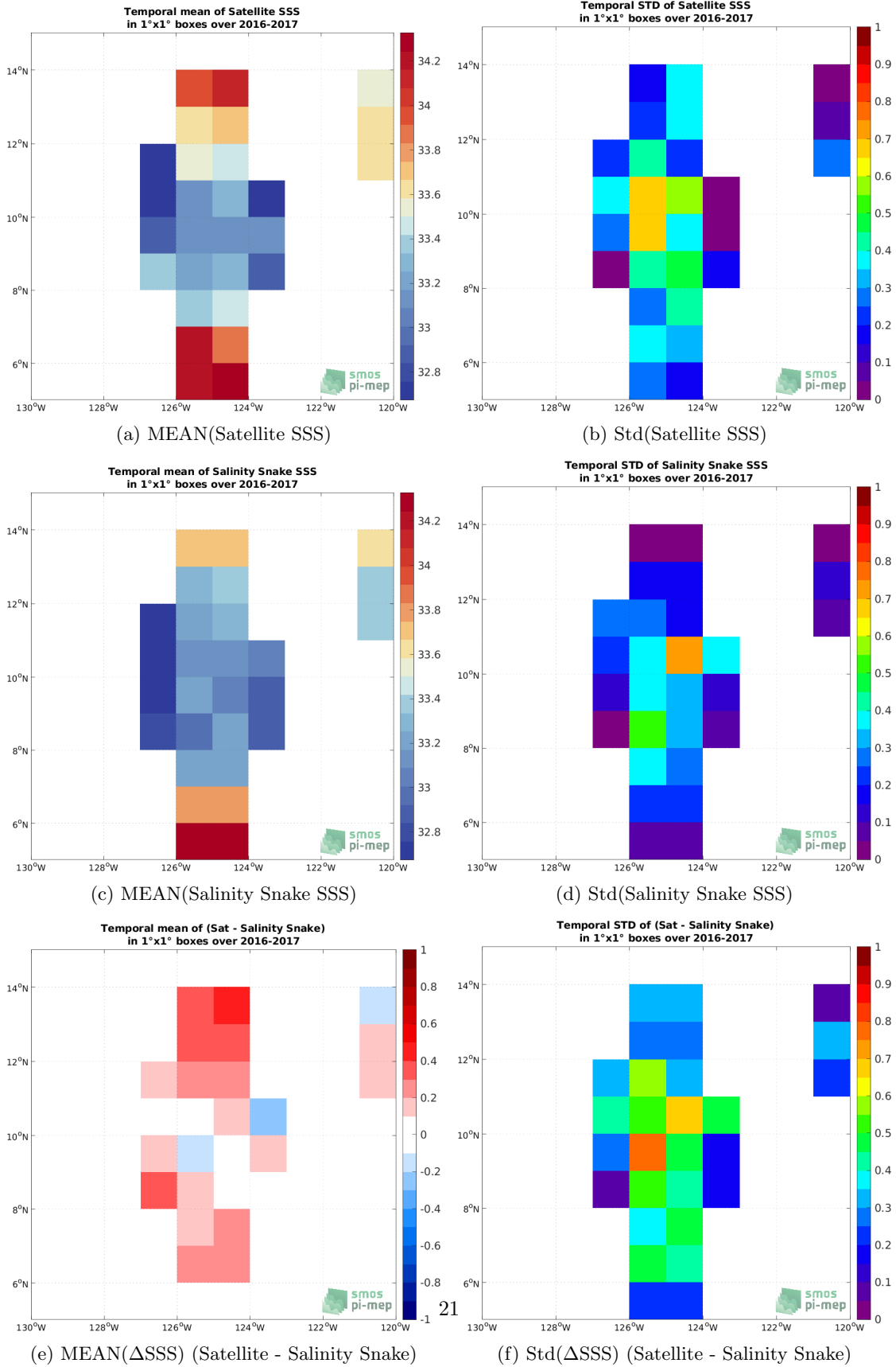
Figure 5: Temporal mean (left) and Std (right) of SSS from SMAP SSS L2 v5 (RSS) (top), Salinity Snake (middle), and of \Delta SSS (Satellite - Salinity Snake). Only match-up pairs are used to generate these maps.
