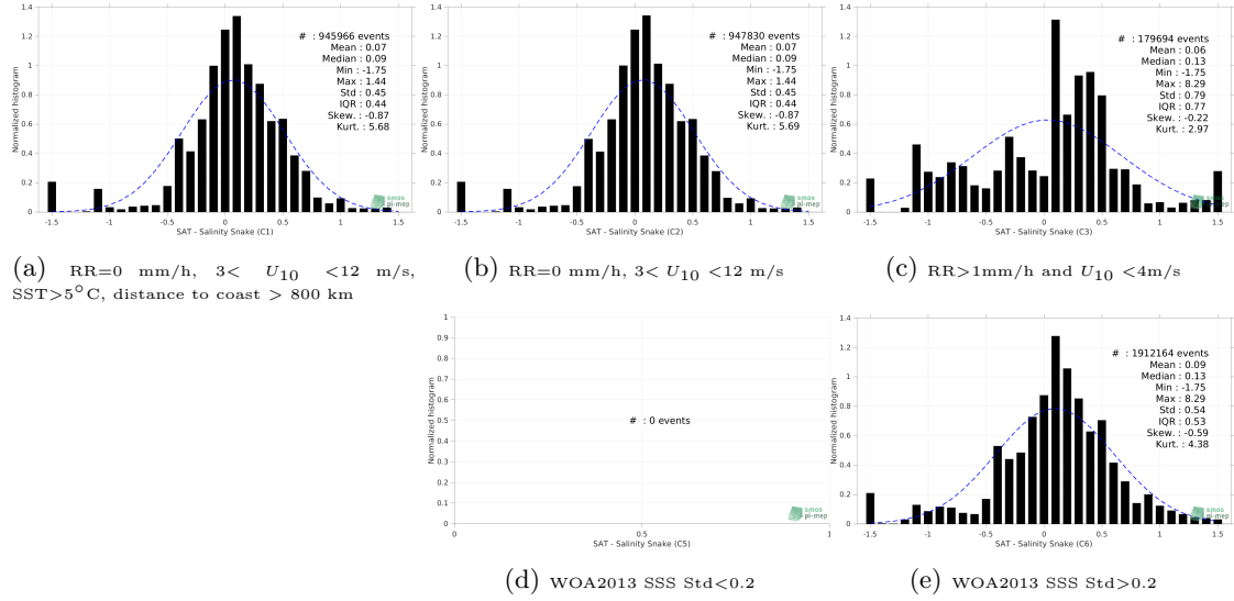
Figure 12: Normalized histogram of \Delta SSS (SMAP SSS L2 v5 (RSS) - Salinity Snake) for 5 different subdatasets corresponding to: RR=0 mm/h, 3 < U_{10} < 12 m/s, SST > 5°C, distance to coast > 800 km (a), RR=0 mm/h, 3 < U_{10} < 12 m/s (b), RR > 1mm/h and U_{10} < 4 m/s (c), WOA2013 SSS Std < 0.2 (d), WOA2013 SSS Std > 0.2 (e).
