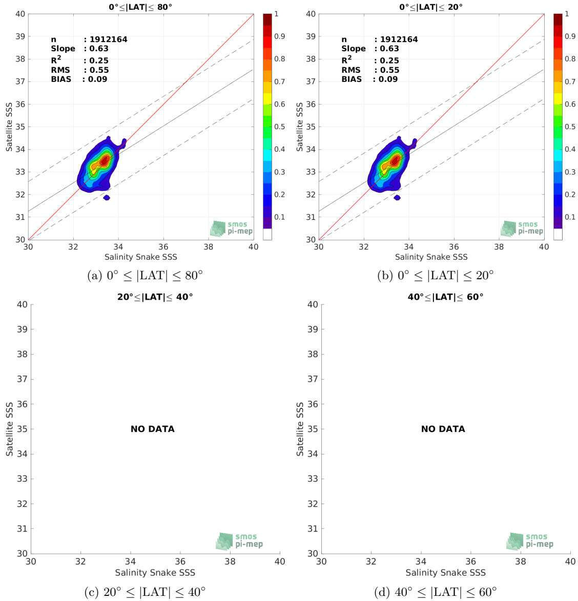
Figure 8: Contour maps of the concentration of SMAP SSS L2 v5 (RSS) SSS (y-axis) versus Salinity Snake SSS (x-axis) at match-up pairs for different latitude bands. For each plot, the red line shows x=y . The black thin and dashed lines indicate a linear fit through the data cloud and the \pm 95\% confidence levels, respectively. The number match-up pairs n , the slope and R^2 coefficient of the linear fit, the root mean square (RMS) and the mean bias between satellite and in situ data are indicated for each latitude band in each plots.
