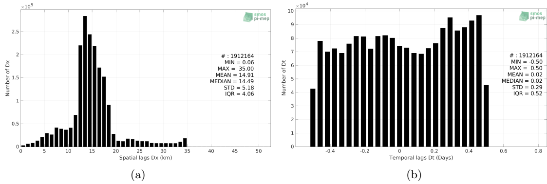
Figure 4: Histograms of the spatial (a) and temporal (b) lags between the location/time of the Salinity Snake measurement and the date of the corresponding SMAP SSS L2 v5 (RSS) SSS pixel.
