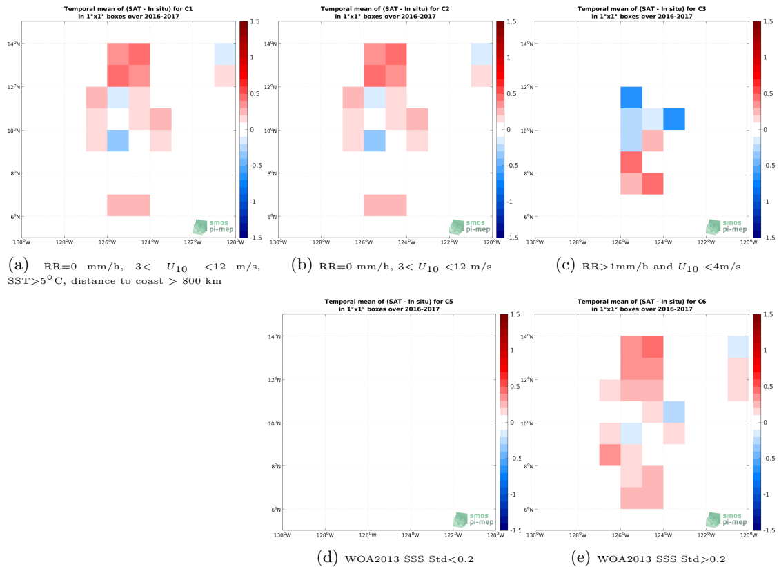
Figure 11: Temporal mean gridded over spatial boxes of size 1^\circ \times 1^\circ of \Delta SSS (SMAP SSS L2 v5 (RSS) - Salinity Snake) for 5 different subdatasets corresponding to:RR=0 mm/h, 3 < U_{10} < 12 m/s, SST >5^\circ C, distance to coast > 800 km (a), RR=0 mm/h, 3 < U_{10} < 12 m/s (b), RR >1 mm/h and U_{10} < 4 m/s (c), WOA2013 SSS Std <0.2 (d), WOA2013 SSS Std >0.2 (e).
