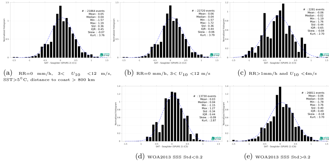
Figure 13: Normalized histogram of \Delta SSS (SMAP SSS L2 v5 (RSS) - Seaglider (SPURS 2)) for 5 different subdatasets corresponding to: RR=0 mm/h, 3 < U_{10} < 12 m/s, SST>5°C, distance to coast > 800 km (a), RR=0 mm/h, 3 < U_{10} < 12 m/s (b), RR>1mm/h and U_{10} < 4 m/s (c), WOA2013 SSS Std<0.2 (d), WOA2013 SSS Std>0.2 (e).
