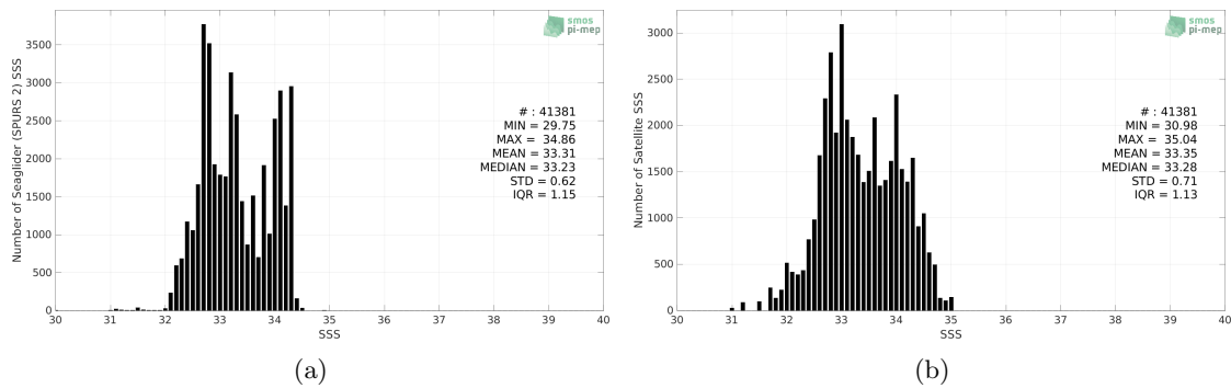
Figure 2: Histograms of SSS from Seaglider (SPURS 2) (a) and SMAP SSS L2 v5 (RSS) (b) considering all match-up pairs per bins of 0.1 over the SPURS 2 Pi-MEP region and for the full satellite product period.
