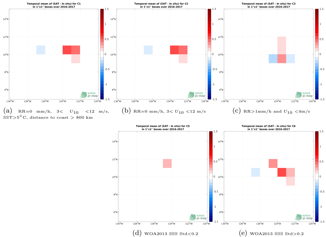
Figure 12: Temporal mean gridded over spatial boxes of size 1^\circ \times 1^\circ of \Delta SSS (SMAP SSS L2 v5 (RSS) - Seaglider (SPURS 2)) for 5 different subdatasets corresponding to:RR=0 mm/h, 3 < U_{10} < 12 m/s, SST >5^\circ\text{C} , distance to coast > 800 km (a), RR=0 mm/h, 3 < U_{10} < 12 m/s (b), RR >1 mm/h and U_{10} < 4 m/s (c), WOA2013 SSS Std <0.2 (d), WOA2013 SSS Std >0.2 (e).
