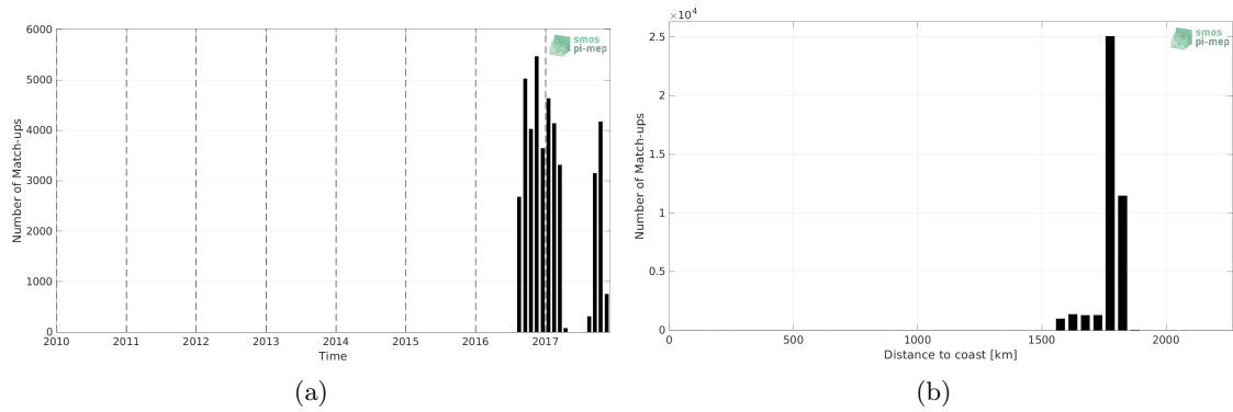
Figure 1: Number of match-ups between Seaglider (SPURS 2) and SMAP SSS L2 v5 (RSS) SSS as a function of time (a) and as function of the distance to coast (b) over the SPURS 2 Pi-MEP region and for the full satellite product period.
