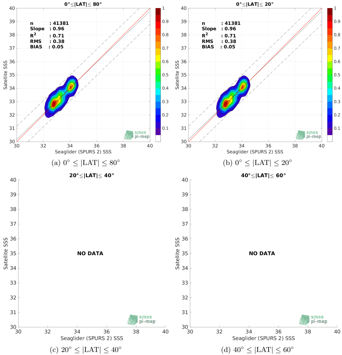
Figure 9: Contour maps of the concentration of SMAP SSS L2 v5 (RSS) SSS (y-axis) versus Seaglider (SPURS 2) SSS (x-axis) at match-up pairs for different latitude bands. For each plot, the red line shows x=y . The black thin and dashed lines indicate a linear fit through the data cloud and the \pm 95\% confidence levels, respectively. The number match-up pairs n , the slope and R^2 coefficient of the linear fit, the root mean square (RMS) and the mean bias between satellite and in situ data are indicated for each latitude band in each plots.
