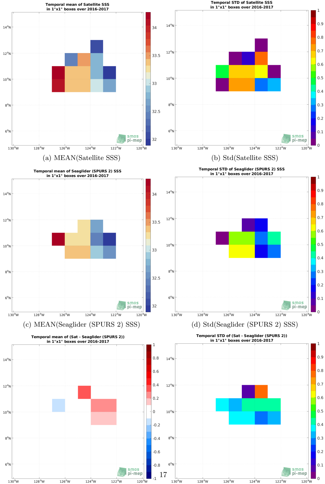
Figure 6: Temporal mean (left) and Std (right) of SSS from SMAP SSS L2 v5 (RSS) (top), Seaglider (SPURS 2) (middle), and of \Delta SSS (Satellite - Seaglider (SPURS 2)). Only match-up pairs are used to generate these maps.
