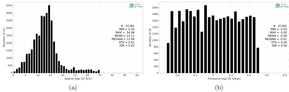
Figure 5: Histograms of the spatial (a) and temporal (b) lags between the location/time of the Seaglider (SPURS 2) measurement and the date of the corresponding SMAP SSS L2 v5 (RSS) SSS pixel.
