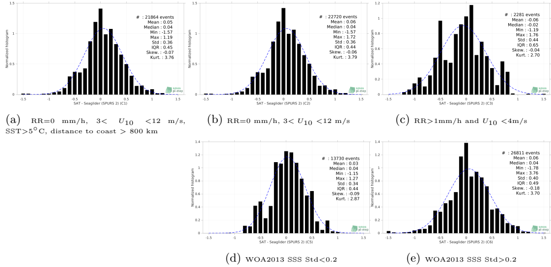
Figure 13: Normalized histogram of \Delta SSS (SMAP SSS L2 v5 (RSS) - Seaglider (SPURS 2)) for 5 different subdatasets corresponding to: RR=0 mm/h, 3 < U_{10} < 12 m/s, SST > 5°C, distance to coast > 800 km (a), RR=0 mm/h, 3 < U_{10} < 12 m/s (b), RR > 1mm/h and U_{10} < 4 m/s (c), WOA2013 SSS Std < 0.2 (d), WOA2013 SSS Std > 0.2 (e).
