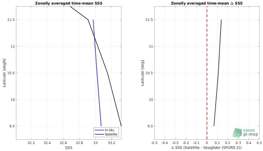
Figure 8: Left panel: Zonal mean SSS from SMAP SSS L2 v5 (RSS) satellite product (black) and from Seaglider (SPURS 2) (blue). Right panel: Zonal mean of \Delta SSS (Satellite - Seaglider (SPURS 2)) for all the collected Pi-MEP match-up pairs estimated over the full satellite product period.
