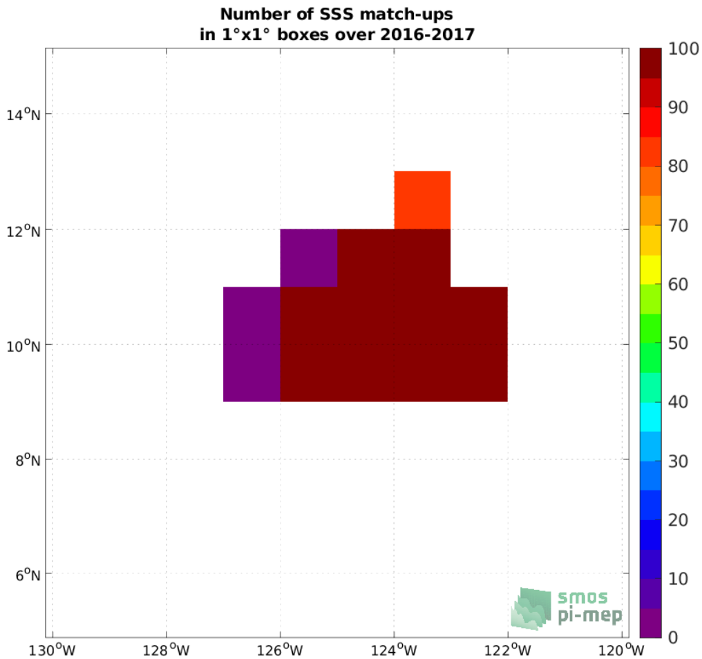
Figure 4: Number of SSS match-ups between Seaglider (SPURS 2) SSS and the SMAP SSS L2 v5 (RSS) SSS product for the SPURS 2 Pi-MEP region over 1°x1° boxes and for the full satellite product period.
