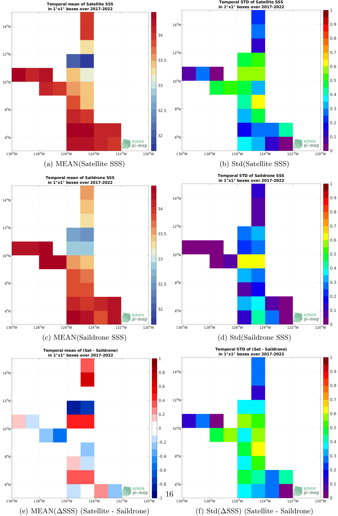
Figure 6: Temporal mean (left) and Std (right) of SSS from SMAP SSS L2 v5 (RSS) (top), Saildrone (middle), and of \Delta SSS (Satellite - Saildrone). Only match-up pairs are used to generate these maps.
