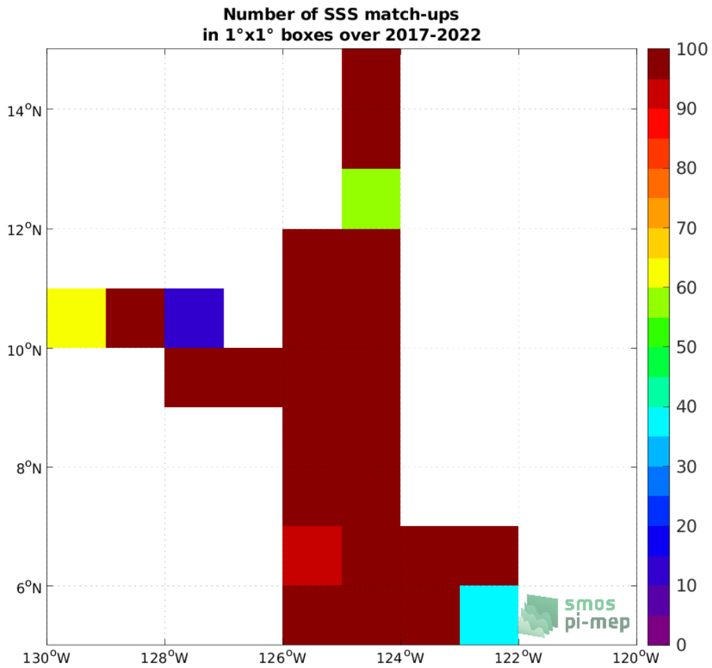
Figure 4: Number of SSS match-ups between Saildrone SSS and the SMAP SSS L2 v5 (RSS) SSS product for the SPURS 2 Pi-MEP region over 1°x1° boxes and for the full satellite product period.
