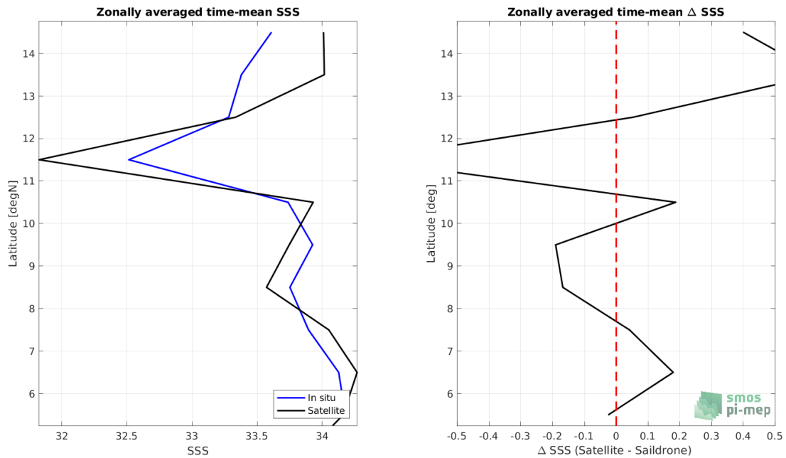
Figure 8: Left panel: Zonal mean SSS from SMAP SSS L2 v5 (RSS) satellite product (black) and from Sairdron (blue). Right panel: Zonal mean of \Delta SSS (Satellite - Sairdron) for all the collected Pi-MEP match-up pairs estimated over the full satellite product period.
