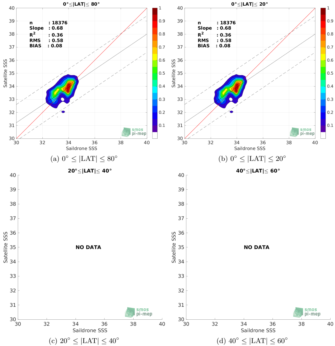
Figure 9: Contour maps of the concentration of SMAP SSS L2 v5 (RSS) SSS (y-axis) versus Saildrone SSS (x-axis) at match-up pairs for different latitude bands. For each plot, the red line shows x=y . The black thin and dashed lines indicate a linear fit through the data cloud and the \pm 95\% confidence levels, respectively. The number match-up pairs n , the slope and R^2 coefficient of the linear fit, the root mean square (RMS) and the mean bias between satellite and in situ data are indicated for each latitude band in each plots.
