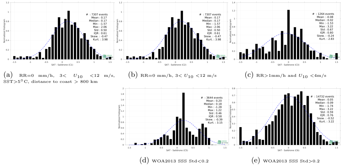
Figure 13: Normalized histogram of \Delta SSS (SMAP SSS L2 v5 (RSS) - Saildrone) for 5 different subdatasets corresponding to: RR=0 mm/h, 3 < U_{10} < 12 m/s, SST>5°C, distance to coast > 800 km (a), RR=0 mm/h, 3 < U_{10} < 12 m/s (b), RR>1mm/h and U_{10} < 4 m/s (c), WOA2013 SSS Std<0.2 (d), WOA2013 SSS Std>0.2 (e).
