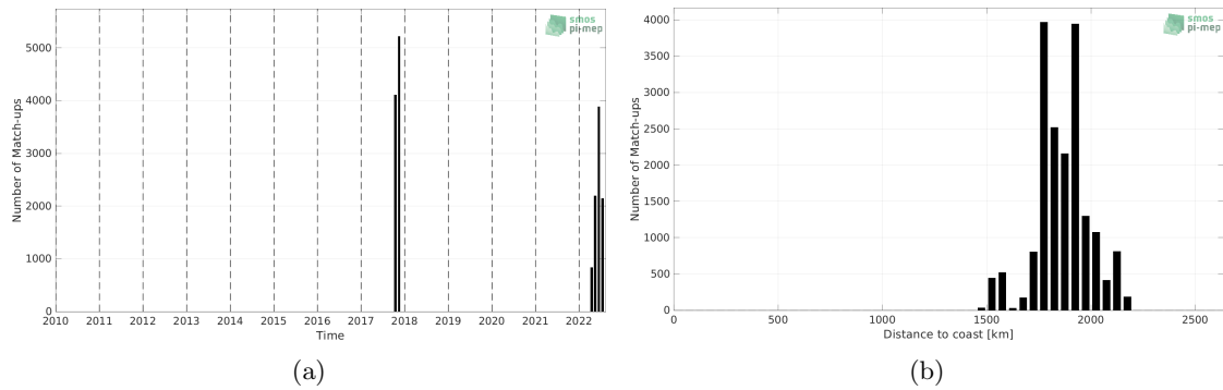
Figure 1: Number of match-ups between Saildrone and SMAP SSS L2 v5 (RSS) SSS as a function of time (a) and as function of the distance to coast (b) over the SPURS 2 Pi-MEP region and for the full satellite product period.
