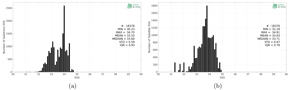
Figure 2: Histograms of SSS from Saildrone (a) and SMAP SSS L2 v5 (RSS) (b) considering all match-up pairs per bins of 0.1 over the SPURS 2 Pi-MEP region and for the full satellite product period.
