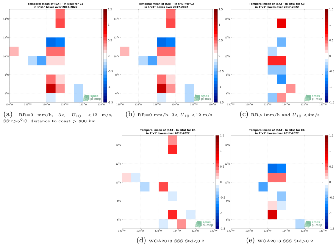
Figure 12: Temporal mean gridded over spatial boxes of size 1^\circ \times 1^\circ of \Delta SSS (SMAP SSS L2 v5 (RSS) - Saildrone) for 5 different subdatasets corresponding to:RR=0 mm/h, 3 < U_{10} < 12 m/s, SST >5^\circ C, distance to coast > 800 km (a), RR=0 mm/h, 3 < U_{10} < 12 m/s (b), RR >1 mm/h and U_{10} < 4 m/s (c), WOA2013 SSS Std <0.2 (d), WOA2013 SSS Std >0.2 (e).
