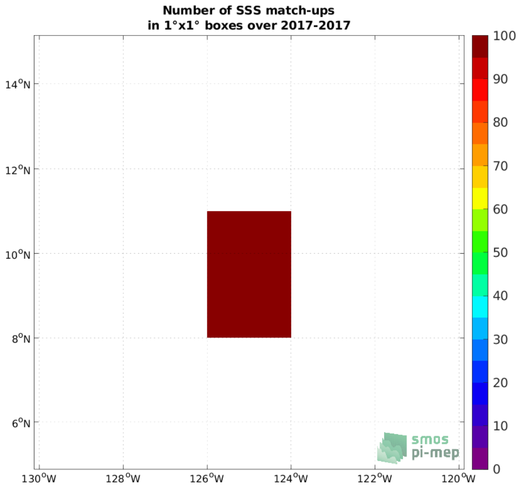
Figure 4: Number of SSS match-ups between Saildrone (SPURS 2) SSS and the SMAP SSS L2 v5 (RSS) SSS product for the SPURS 2 Pi-MEP region over 1°×1° boxes and for the full satellite product period.
