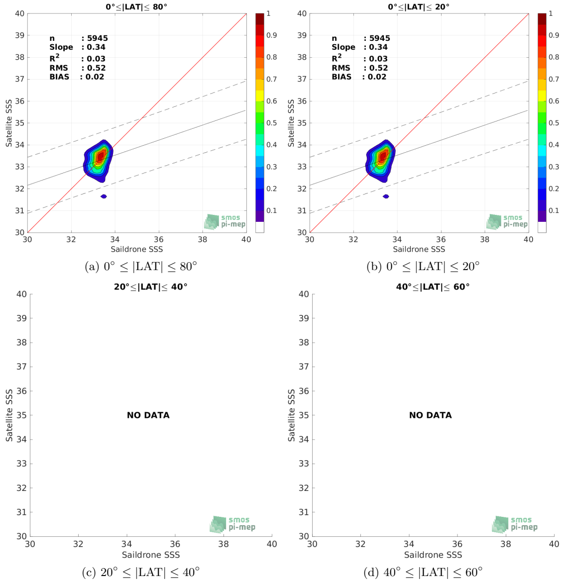
Figure 8: Contour maps of the concentration of SMAP SSS L2 v5 (RSS) SSS (y-axis) versus Saildrone SSS (x-axis) at match-up pairs for different latitude bands. For each plot, the red line shows x=y . The black thin and dashed lines indicate a linear fit through the data cloud and the \pm 95\% confidence levels, respectively. The number match-up pairs n , the slope and R^2 coefficient of the linear fit, the root mean square (RMS) and the mean bias between satellite and in situ data are indicated for each latitude band in each plots.
