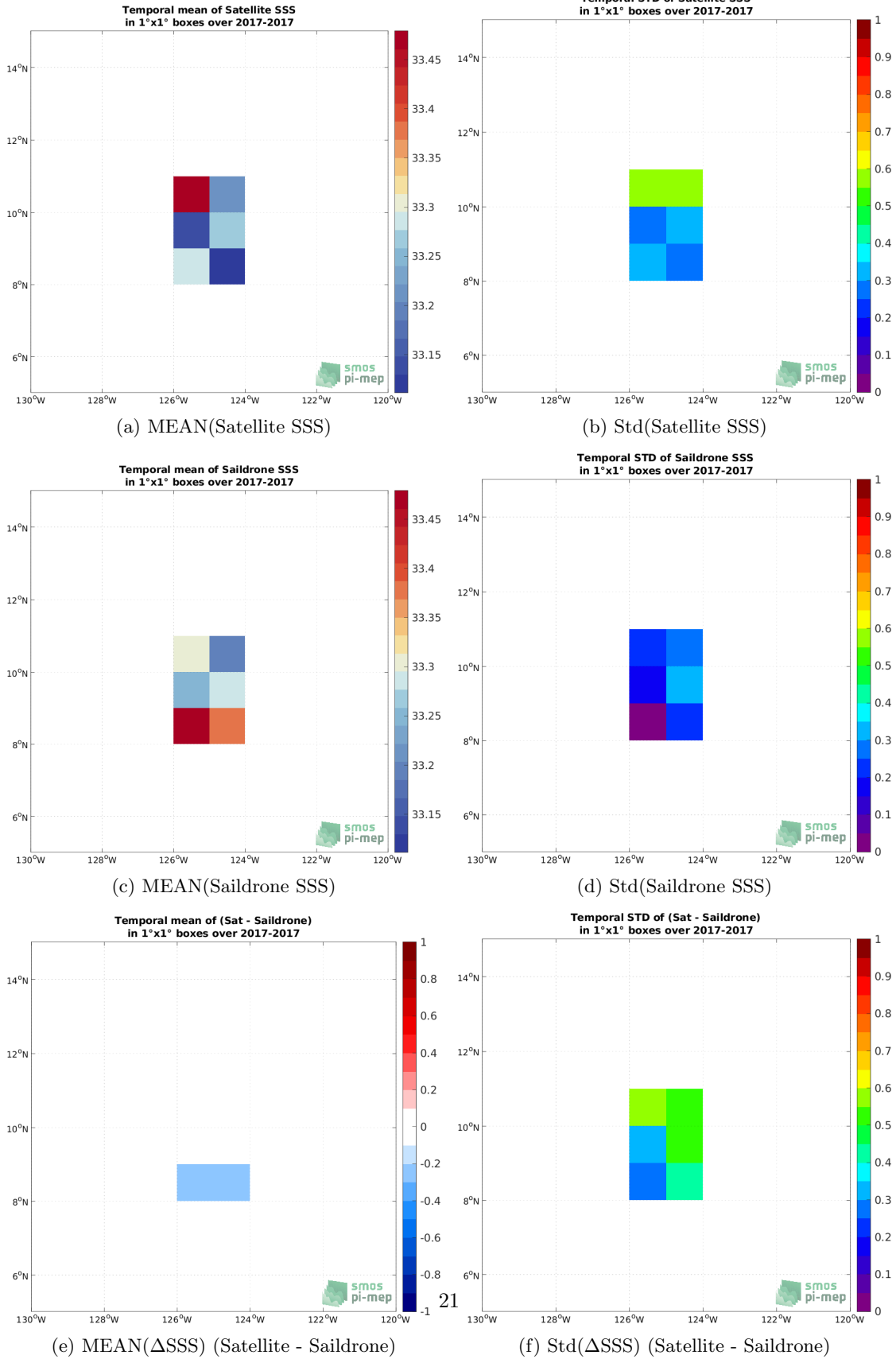
Figure 5: Temporal mean (left) and Std (right) of SSS from SMAP SSS L2 v5 (RSS) (top), Saildrone (middle), and of \Delta SSS (Satellite - Saildrone). Only match-up pairs are used to generate these maps.
