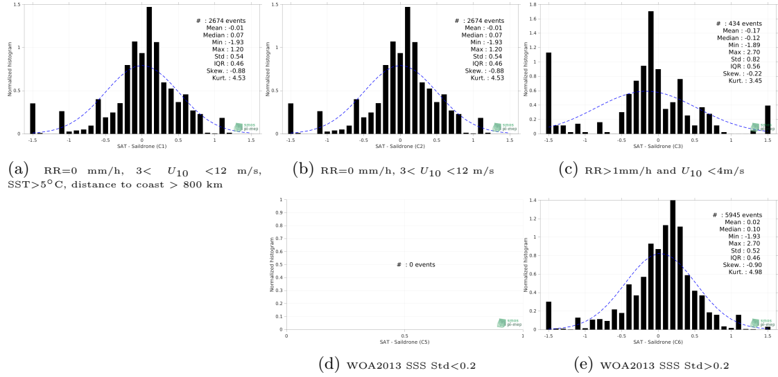
Figure 12: Normalized histogram of \Delta SSS (SMAP SSS L2 v5 (RSS) - Saildrone) for 5 different subdatasets corresponding to: RR=0 mm/h, 3 < U_{10} < 12 m/s, SST > 5°C, distance to coast > 800 km (a), RR=0 mm/h, 3 < U_{10} < 12 m/s (b), RR > 1mm/h and U_{10} < 4 m/s (c), WOA2013 SSS Std < 0.2 (d), WOA2013 SSS Std > 0.2 (e).
