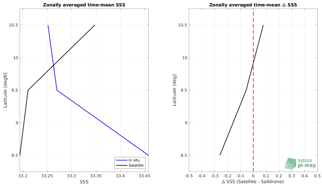
Figure 7: Left panel: Zonal mean SSS from SMAP SSS L2 v5 (RSS) satellite product (black) and from Sairdrone (blue). Right panel: Zonal mean of \Delta SSS (Satellite - Sairdrone) for all the collected Pi-MEP match-up pairs estimated over the full satellite product period.
