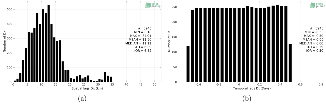
Figure 4: Histograms of the spatial (a) and temporal (b) lags between the location/time of the Saildrone measurement and the date of the corresponding SMAP SSS L2 v5 (RSS) SSS pixel.
