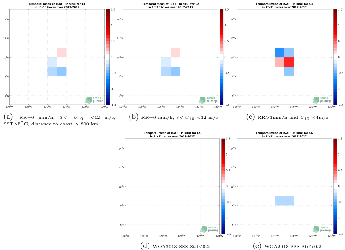
Figure 11: Temporal mean gridded over spatial boxes of size 1^\circ \times 1^\circ of \Delta SSS (SMAP SSS L2 v5 (RSS) - Saildrone) for 5 different subdatasets corresponding to:RR=0 mm/h, 3 < U_{10} < 12 m/s, SST >5^\circ C, distance to coast > 800 km (a), RR=0 mm/h, 3 < U_{10} < 12 m/s (b), RR >1 mm/h and U_{10} < 4 m/s (c), WOA2013 SSS Std <0.2 (d), WOA2013 SSS Std >0.2 (e).
