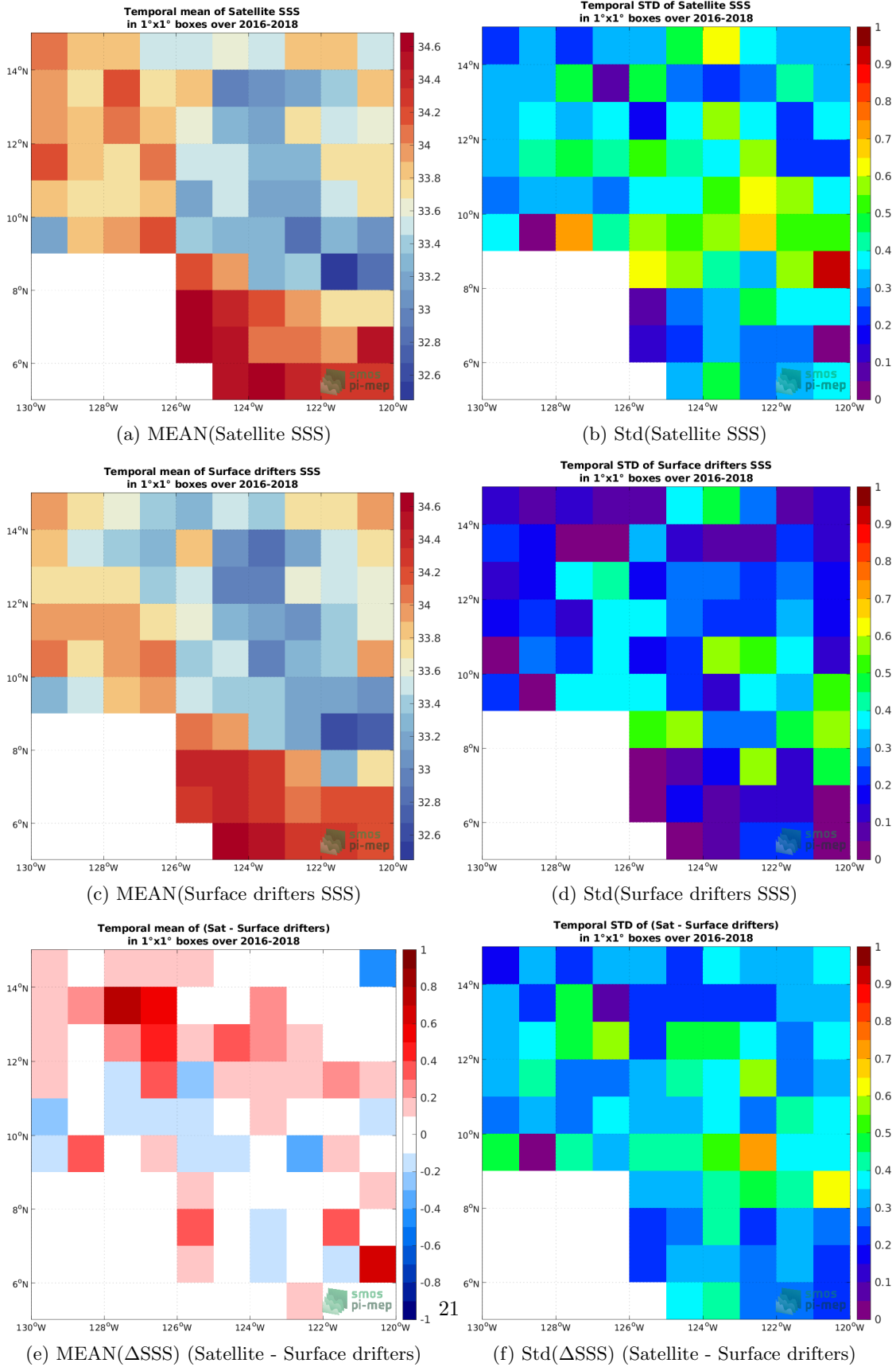
Figure 5: Temporal mean (left) and Std (right) of SSS from SMAP SSS L2 v5 (RSS) (top), Surface drifters (middle), and of \Delta SSS (Satellite - Surface drifters). Only match-up pairs are used to generate these maps.
