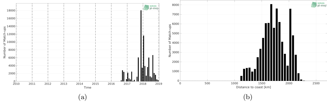
Figure 1: Number of match-ups between Surface drifters and SMAP SSS L2 v5 (RSS) SSS as a function of time (a) and as function of the distance to coast (b) over the SPURS 2 Pi-MEP region and for the full satellite product period.
