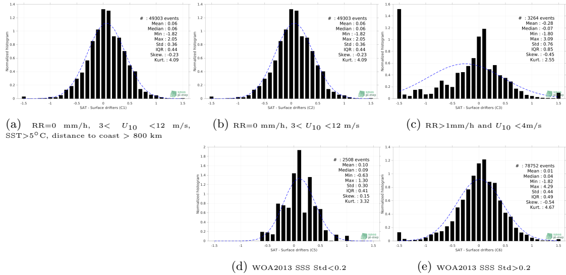
Figure 12: Normalized histogram of \Delta SSS (SMAP SSS L2 v5 (RSS) - Surface drifters) for 5 different subdatasets corresponding to: RR=0 mm/h, 3 < U_{10} < 12 m/s, SST>5°C, distance to coast > 800 km (a), RR=0 mm/h, 3 < U_{10} < 12 m/s (b), RR>1mm/h and U_{10} < 4 m/s (c), WOA2013 SSS Std<0.2 (d), WOA2013 SSS Std>0.2 (e).
