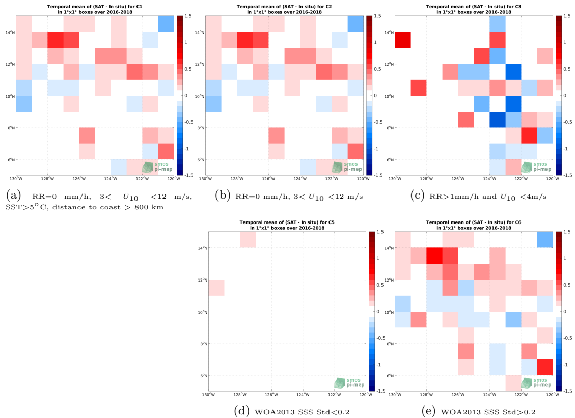
Figure 11: Temporal mean gridded over spatial boxes of size 1^\circ \times 1^\circ of \Delta SSS (SMAP SSS L2 v5 (RSS) - Surface drifters) for 5 different subdatasets corresponding to:RR=0 mm/h, 3 < U_{10} < 12 m/s, SST >5^\circ C, distance to coast > 800 km (a), RR=0 mm/h, 3 < U_{10} < 12 m/s (b), RR >1 mm/h and U_{10} < 4 m/s (c), WOA2013 SSS Std <0.2 (d), WOA2013 SSS Std >0.2 (e).
