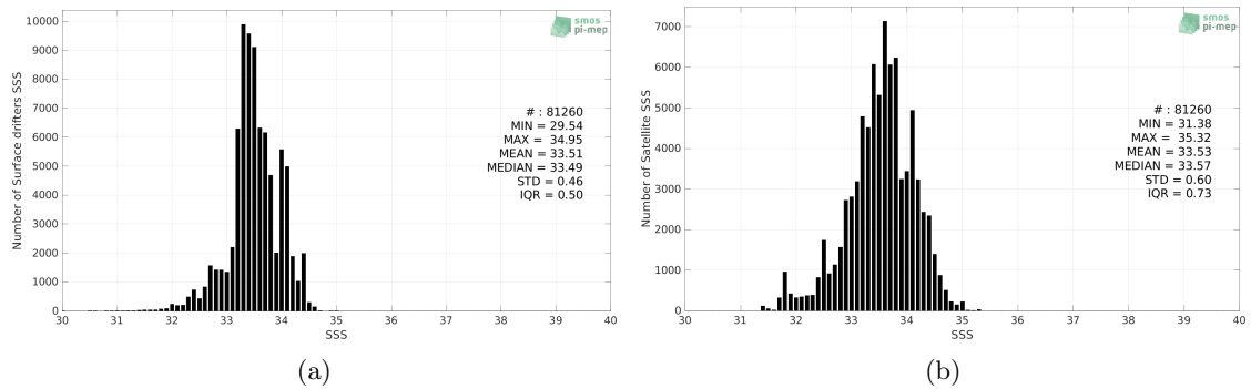
Figure 2: Histograms of SSS from Surface drifters (a) and SMAP SSS L2 v5 (RSS) (b) considering all match-up pairs per bins of 0.1 over the SPURS 2 Pi-MEP region and for the full satellite product period.
