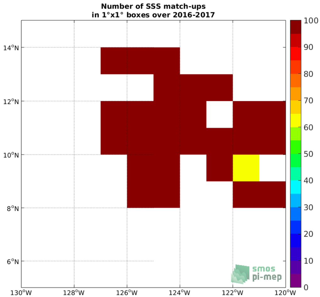
Figure 3: Number of SSS match-ups between Waveglider SSS and the SMAP SSS L2 v4 (RSS) SSS product for the SPURS 2 Pi-MEP region over 1°×1° boxes and for the full satellite product period.
