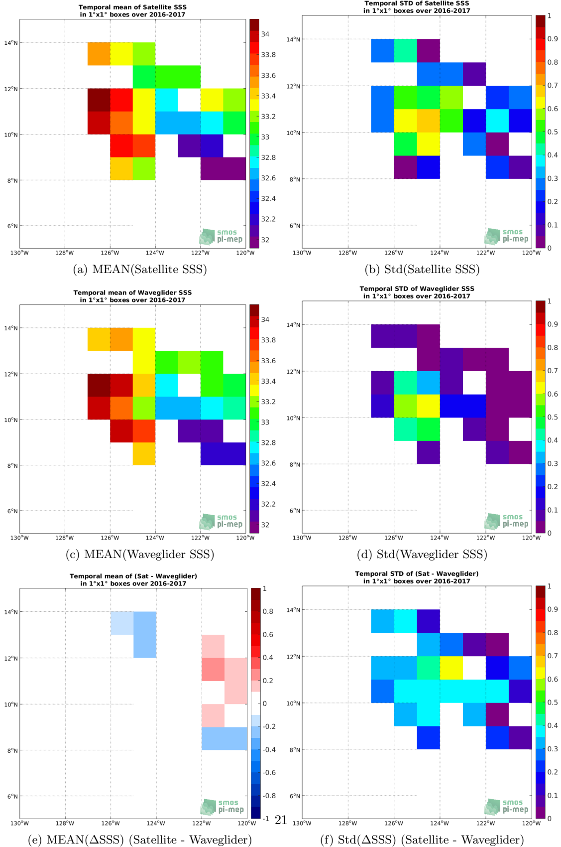
Figure 5: Temporal mean (left) and Std (right) of SSS from SMAP SSS L2 v4 (RSS) (top), Waveglider (middle), and of \Delta SSS (Satellite - Waveglider). Only match-up pairs are used to generate these maps.
