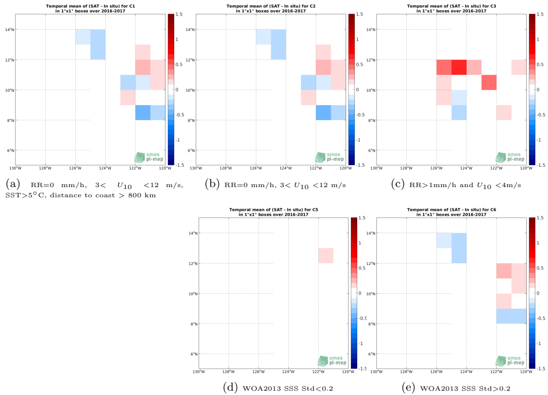
Figure 11: Temporal mean gridded over spatial boxes of size 1^\circ \times 1^\circ of \Delta\text{SSS} (SMAP SSS L2 v4 (RSS) - Waveglider) for 5 different subdatasets corresponding to:RR=0 mm/h, 3 < U_{10} < 12 m/s, SST >5^\circ\text{C} , distance to coast > 800 km (a), RR=0 mm/h, 3 < U_{10} < 12 m/s (b), RR >1 mm/h and U_{10} < 4 m/s (c), WOA2013 SSS Std <0.2 (d), WOA2013 SSS Std >0.2 (e).
