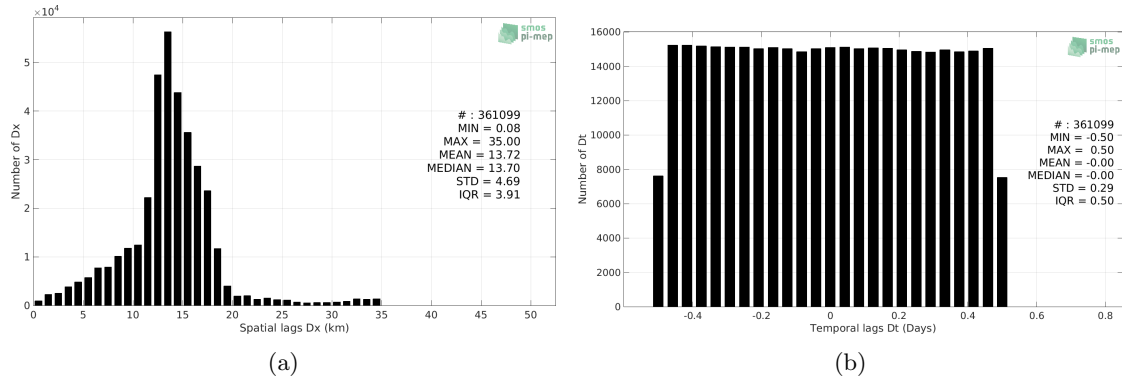
Figure 4: Histograms of the spatial (a) and temporal (b) lags between the location/time of the Waveglider measurement and the date of the corresponding SMAP SSS L2 v4 (RSS) SSS pixel.
