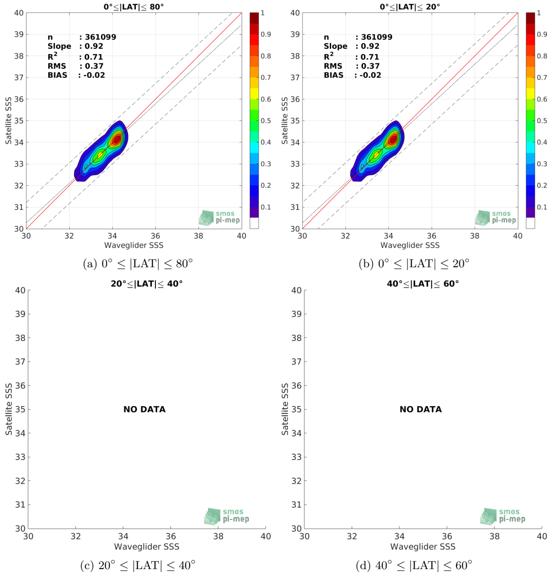
Figure 8: Contour maps of the concentration of SMAP SSS L2 v4 (RSS) SSS (y-axis) versus Waveglider SSS (x-axis) at match-up pairs for different latitude bands. For each plot, the red line shows x=y . The black thin and dashed lines indicate a linear fit through the data cloud and the \pm 95\% confidence levels, respectively. The number match-up pairs n , the slope and R^2 coefficient of the linear fit, the root mean square (RMS) and the mean bias between satellite and in situ data are indicated for each latitude band in each plots.
