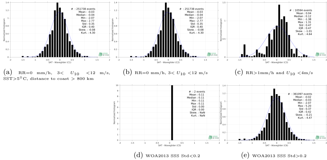
Figure 12: Normalized histogram of \Delta SSS (SMAP SSS L2 v4 (RSS) - Waveglider) for 5 different subdatasets corresponding to: RR=0 mm/h, 3 < U_{10} < 12 m/s, SST > 5°C, distance to coast > 800 km (a), RR=0 mm/h, 3 < U_{10} < 12 m/s (b), RR > 1mm/h and U_{10} < 4 m/s (c), WOA2013 SSS Std < 0.2 (d), WOA2013 SSS Std > 0.2 (e).
