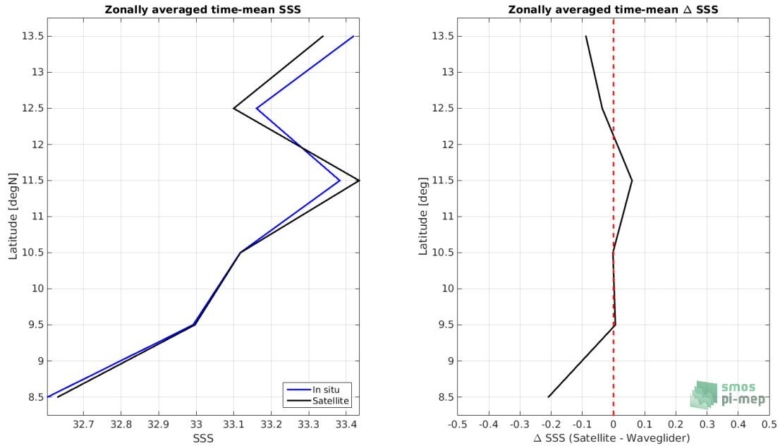
Figure 7: Left panel: Zonal mean SSS from SMAP SSS L2 v4 (RSS) satellite product (black) and from Waveglider (blue). Right panel: Zonal mean of \Delta SSS (Satellite - Waveglider) for all the collected Pi-MEP match-up pairs estimated over the full satellite product period.
