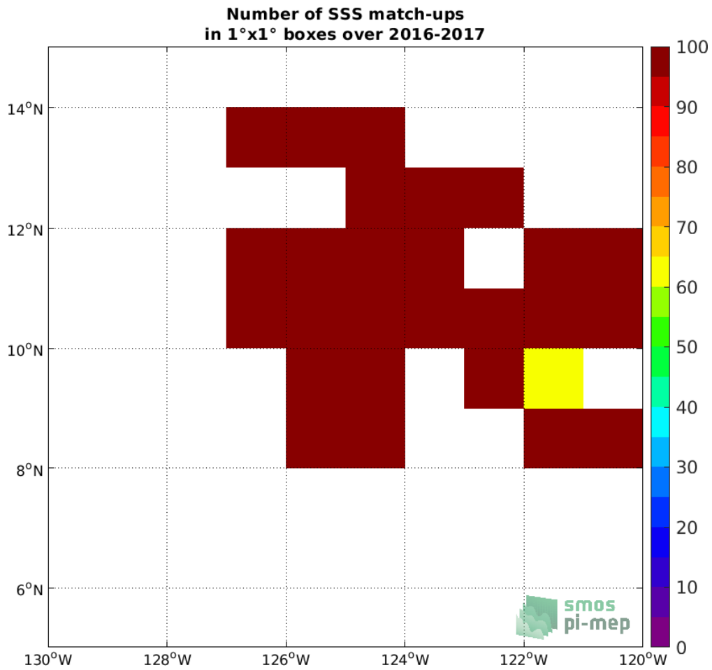
Figure 3: Number of SSS match-ups between Waveglider SSS and the SMAP SSS L2 v4 (RSS) SSS product for the SPURS 2 Pi-MEP region over 1°x1° boxes and for the full satellite product period.
