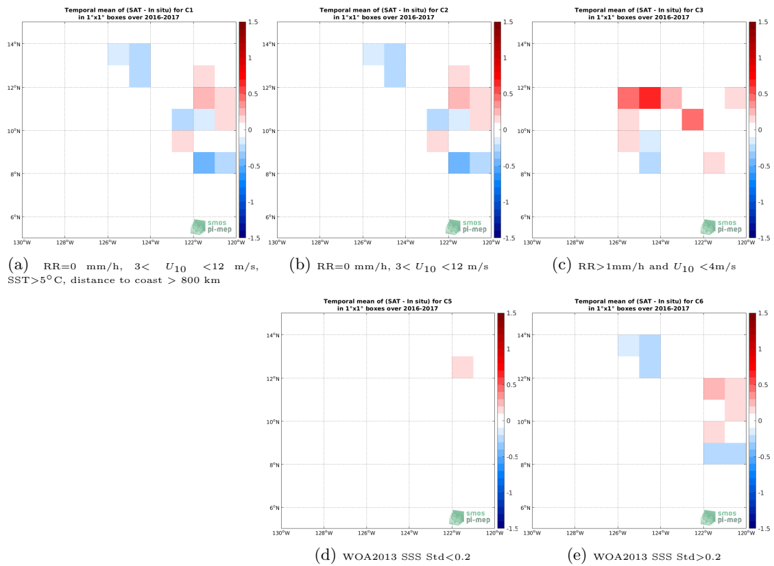
Figure 11: Temporal mean gridded over spatial boxes of size 1^\circ \times 1^\circ of \Delta SSS (SMAP SSS L2 v4 (RSS) - Waveglider) for 5 different subdatasets corresponding to:RR=0 mm/h, 3 < U_{10} < 12 m/s, SST >5^\circ\text{C} , distance to coast > 800 km (a), RR=0 mm/h, 3 < U_{10} < 12 m/s (b), RR >1 mm/h and U_{10} < 4 m/s (c), WOA2013 SSS Std <0.2 (d), WOA2013 SSS Std >0.2 (e).
