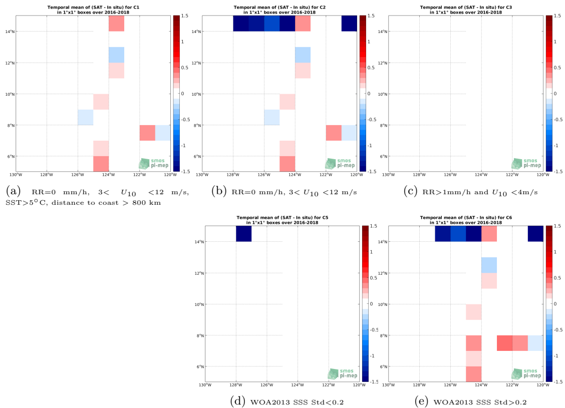
Figure 12: Temporal mean gridded over spatial boxes of size 1^\circ \times 1^\circ of \Delta SSS (SMAP SSS L2 v4 (RSS) - TSG (SAMOS)) for 5 different subdatasets corresponding to:RR=0 mm/h, 3 < U_{10} < 12 m/s, SST >5^\circ\text{C} , distance to coast > 800 km (a), RR=0 mm/h, 3 < U_{10} < 12 m/s (b), RR >1 mm/h and U_{10} < 4 m/s (c), WOA2013 SSS Std <0.2 (d), WOA2013 SSS Std >0.2 (e).
