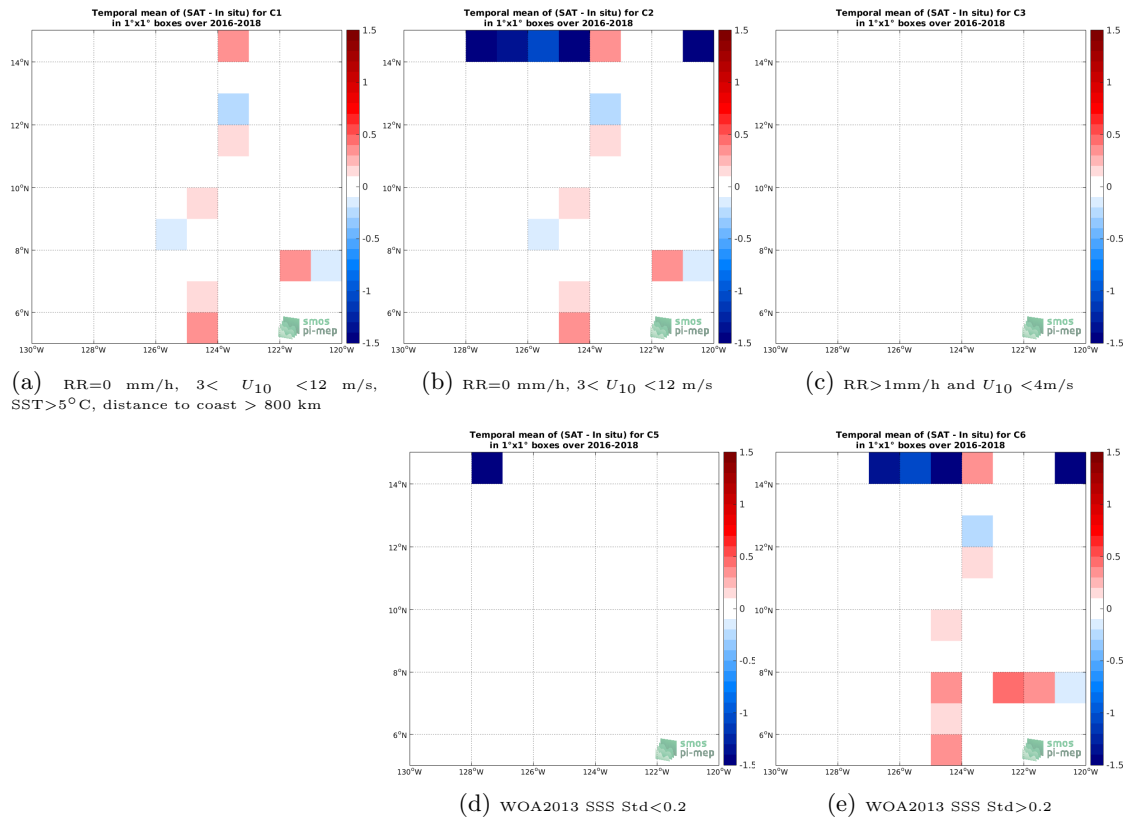
Figure 12: Temporal mean gridded over spatial boxes of size 1^\circ \times 1^\circ of \Delta SSS (SMAP-L2-RSS-V4 - TSG-SAMOS) for 5 different subdatasets corresponding to:RR=0 mm/h, 3 < U_{10} < 12 m/s, SST >5^\circ\text{C} , distance to coast > 800 km (a), RR=0 mm/h, 3 < U_{10} < 12 m/s (b), RR >1 mm/h and U_{10} < 4 m/s (c), WOA2013 SSS Std <0.2 (d), WOA2013 SSS Std >0.2 (e).
