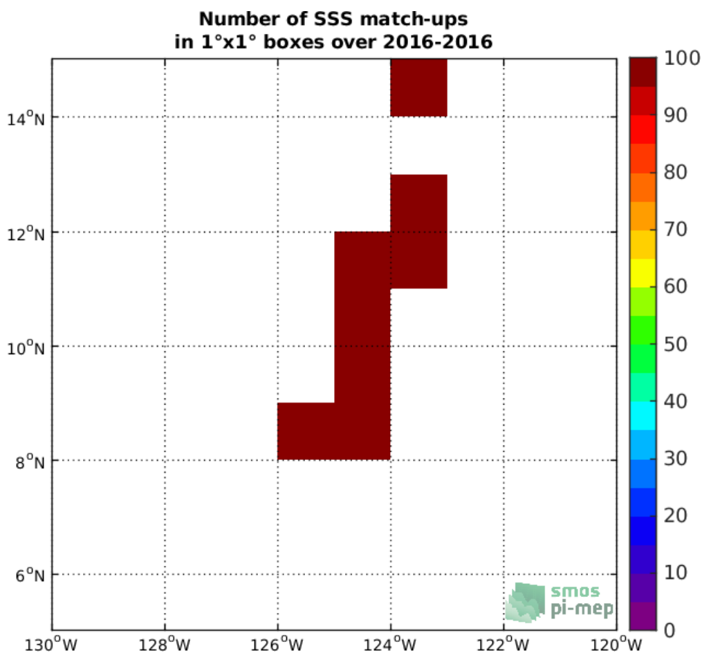
Figure 4: Number of SSS match-ups between TSG-SAMOS SSS and the SMAP-L2-RSS-V4 SSS product for the SPURS 2 Pi-MEP region over 1°x1° boxes and for the full satellite product period.
