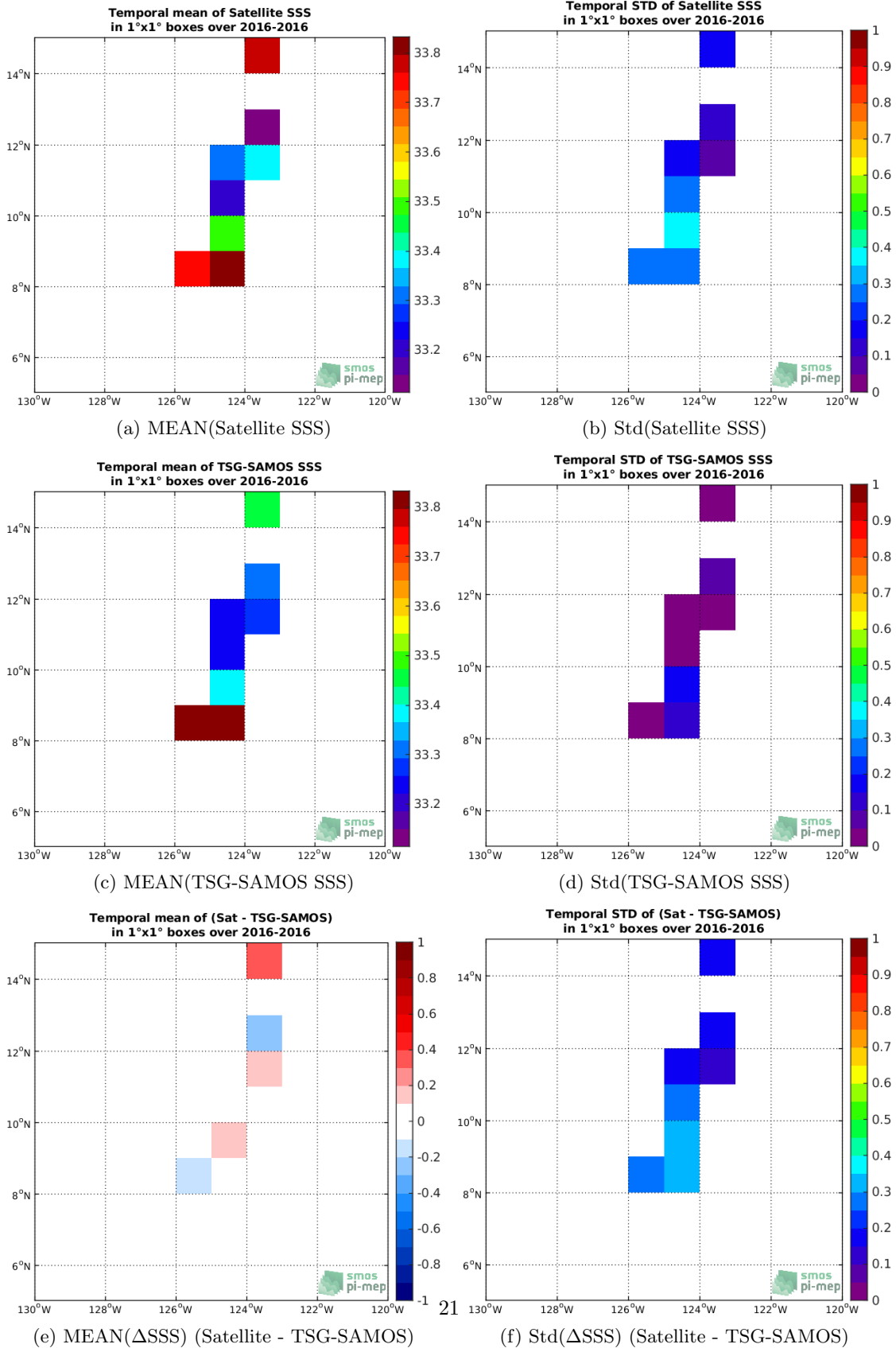
Figure 6: Temporal mean (left) and Std (right) of SSS from SMAP-L2-RSS-V4 (top), TSG-SAMOS (middle), and of \Delta SSS (Satellite - TSG-SAMOS). Only match-up pairs are used to generate these maps.
