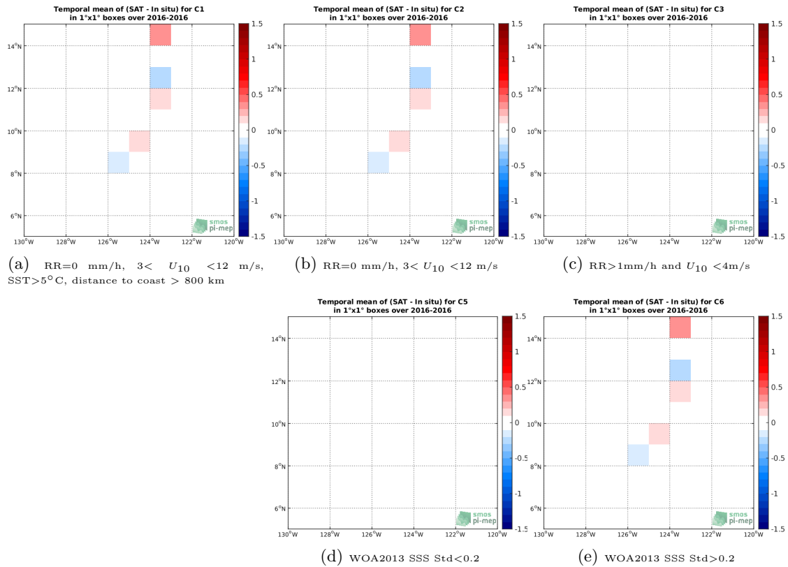
Figure 12: Temporal mean gridded over spatial boxes of size 1^\circ \times 1^\circ of \Delta SSS (SMAP-L2-RSS-V4 - TSG-SAMOS) for 5 different subdatasets corresponding to:RR=0 mm/h, 3 < U_{10} < 12 m/s, SST >5^\circ C, distance to coast > 800 km (a), RR=0 mm/h, 3 < U_{10} < 12 m/s (b), RR >1 mm/h and U_{10} < 4 m/s (c), WOA2013 SSS Std <0.2 (d), WOA2013 SSS Std >0.2 (e).
