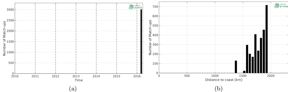
Figure 1: Number of match-ups between TSG-SAMOS and SMAP-L2-RSS-V4 SSS as a function of time (a) and as function of the distance to coast (b) over the SPURS 2 Pi-MEP region and for the full satellite product period.
