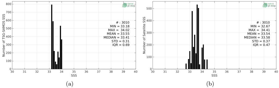
Figure 2: Histograms of SSS from TSG-SAMOS (a) and SMAP-L2-RSS-V4 (b) considering all match-up pairs per bins of 0.1 over the SPURS 2 Pi-MEP region and for the full satellite product period.
