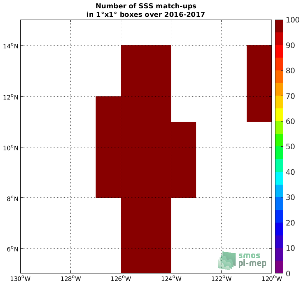
Figure 3: Number of SSS match-ups between Salinity Snake SSS and the SMAP SSS L2 v4 (RSS) SSS product for the SPURS 2 Pi-MEP region over 1°x1° boxes and for the full satellite product period.
