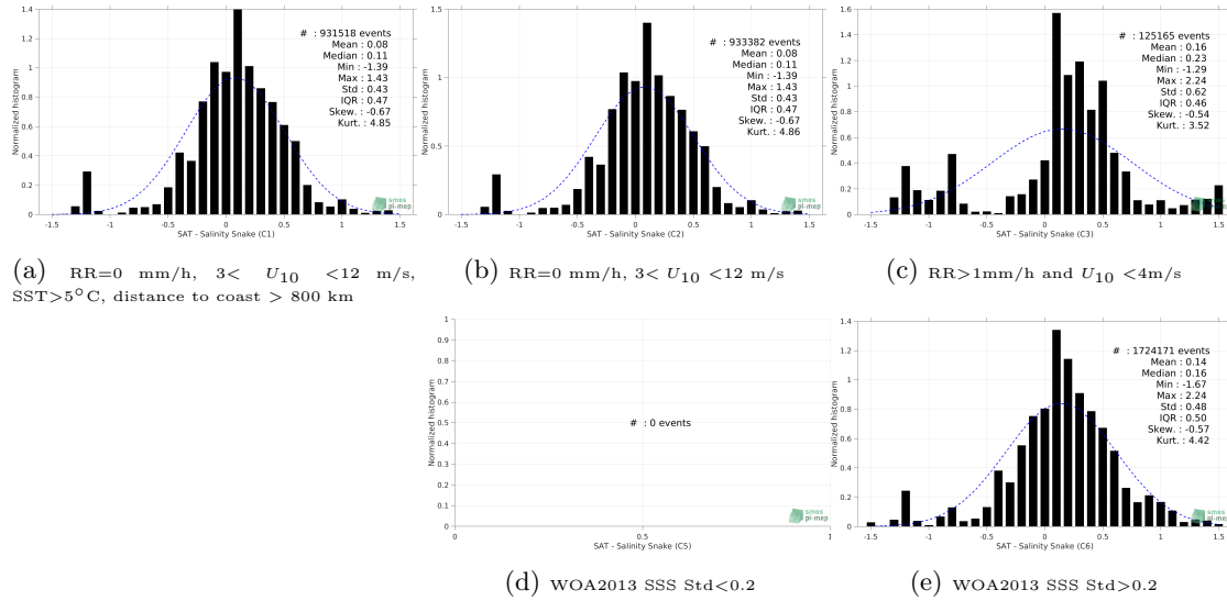
Figure 12: Normalized histogram of \Delta SSS (SMAP SSS L2 v4 (RSS) - Salinity Snake) for 5 different subdatasets corresponding to: RR=0 mm/h, 3 < U_{10} < 12 m/s, SST > 5°C, distance to coast > 800 km (a), RR=0 mm/h, 3 < U_{10} < 12 m/s (b), RR > 1mm/h and U_{10} < 4 m/s (c), WOA2013 SSS Std < 0.2 (d), WOA2013 SSS Std > 0.2 (e).
