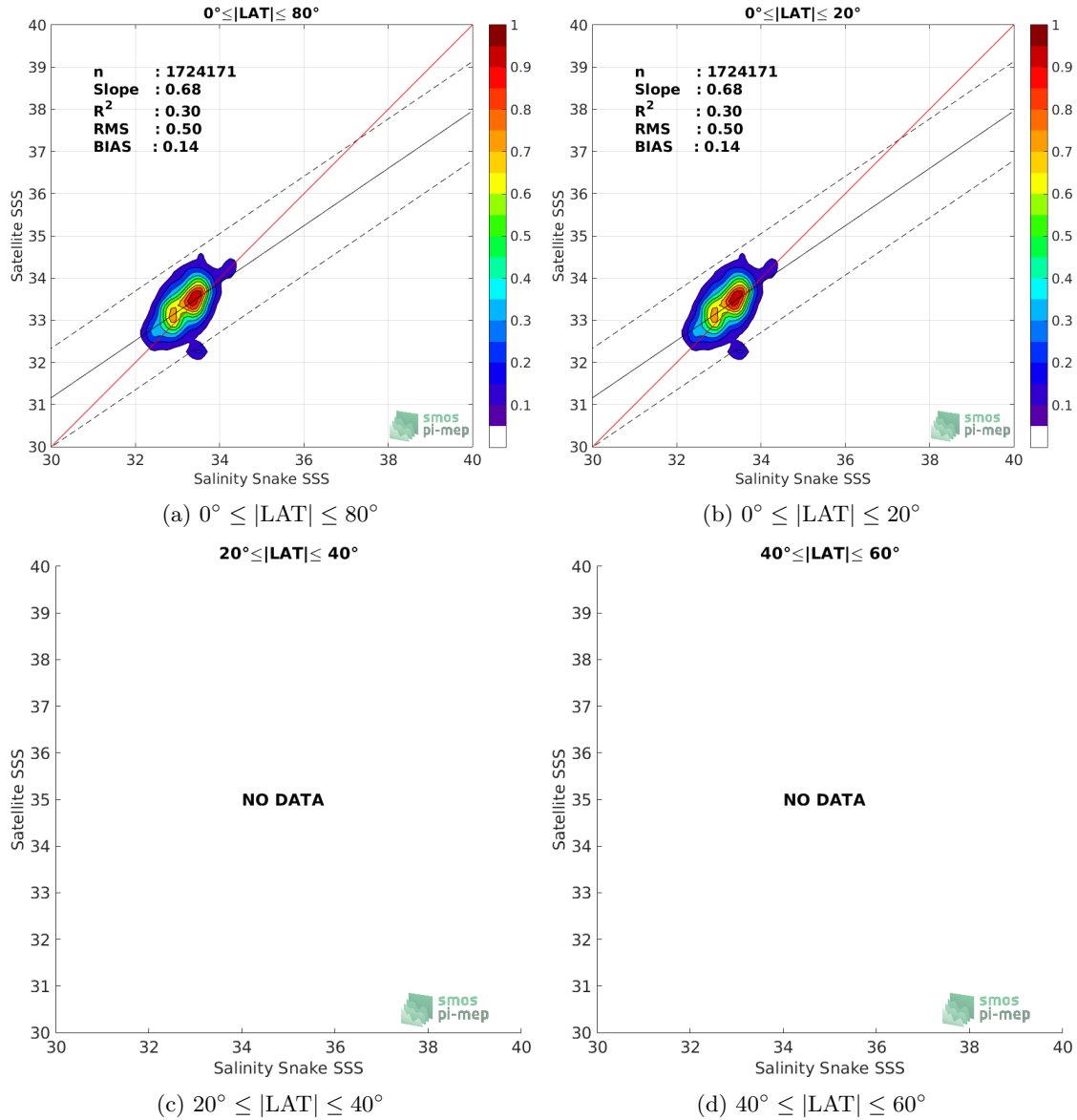
Figure 9: Contour maps of the concentration of SMAP SSS L2 v4 (RSS) SSS (y-axis) versus Salinity Snake SSS (x-axis) at match-up pairs for different latitude bands. For each plot, the red line shows x=y . The black thin and dashed lines indicate a linear fit through the data cloud and the \pm 95\% confidence levels, respectively. The number match-up pairs n , the slope and R^2 coefficient of the linear fit, the root mean square (RMS) and the mean bias between satellite and in situ data are indicated for each latitude band in each plots.
