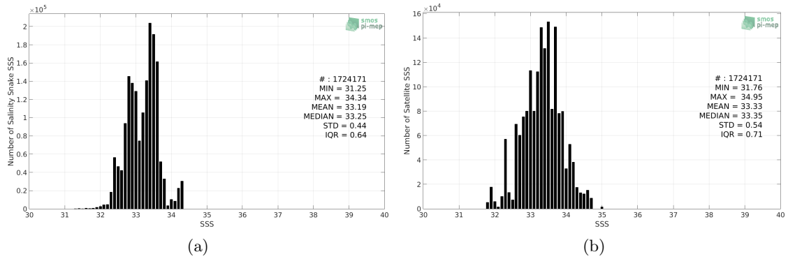
Figure 2: Histograms of SSS from Salinity Snake (a) and SMAP SSS L2 v4 (RSS) (b) considering all match-up pairs per bins of 0.1 over the SPURS 2 Pi-MEP region and for the full satellite product period.
