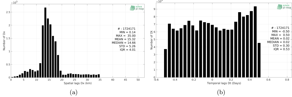
Figure 5: Histograms of the spatial (a) and temporal (b) lags between the time of the Salinity Snake measurements and the date of the corresponding SMAP SSS L2 v4 (RSS) SSS product.
