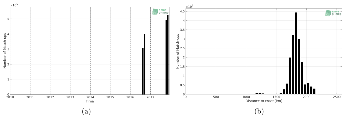
Figure 1: Number of match-ups between Salinity Snake and SMAP SSS L2 v4 (RSS) SSS as a function of time (a) and as function of the distance to coast (b) over the SPURS 2 Pi-MEP region and for the full satellite product period.
