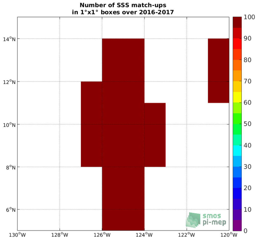
Figure 4: Number of SSS match-ups between Salinity Snake SSS and the SMAP SSS L2 v4 (RSS) SSS product for the SPURS 2 Pi-MEP region over 1°x1° boxes and for the full satellite product period.
