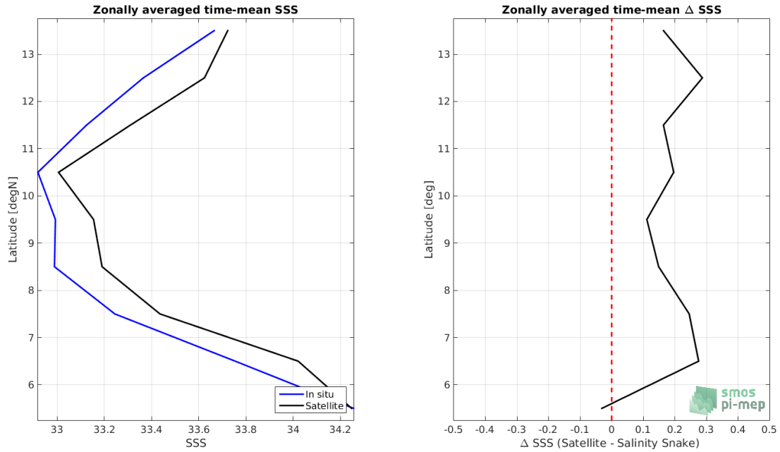
Figure 8: Left panel: Zonal mean SSS from SMAP SSS L2 v4 (RSS) satellite product (black) and from Salinity Snake (blue). Right panel: Zonal mean of \Delta SSS (Satellite - Salinity Snake) for all the collected Pi-MEP match-up pairs estimated over the full satellite product period.
