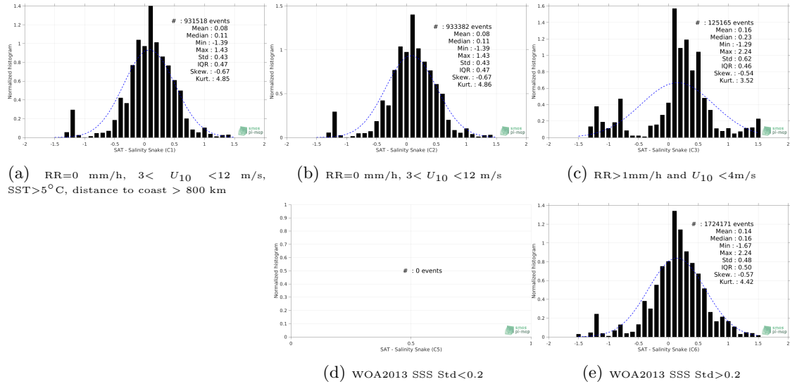
Figure 13: Normalized histogram of \Delta SSS (SMAP SSS L2 v4 (RSS) - Salinity Snake) for 5 different subdatasets corresponding to: RR=0 mm/h, 3 < U_{10} < 12 m/s, SST > 5°C, distance to coast > 800 km (a), RR=0 mm/h, 3 < U_{10} < 12 m/s (b), RR > 1mm/h and U_{10} < 4 m/s (c), WOA2013 SSS Std < 0.2 (d), WOA2013 SSS Std > 0.2 (e).
