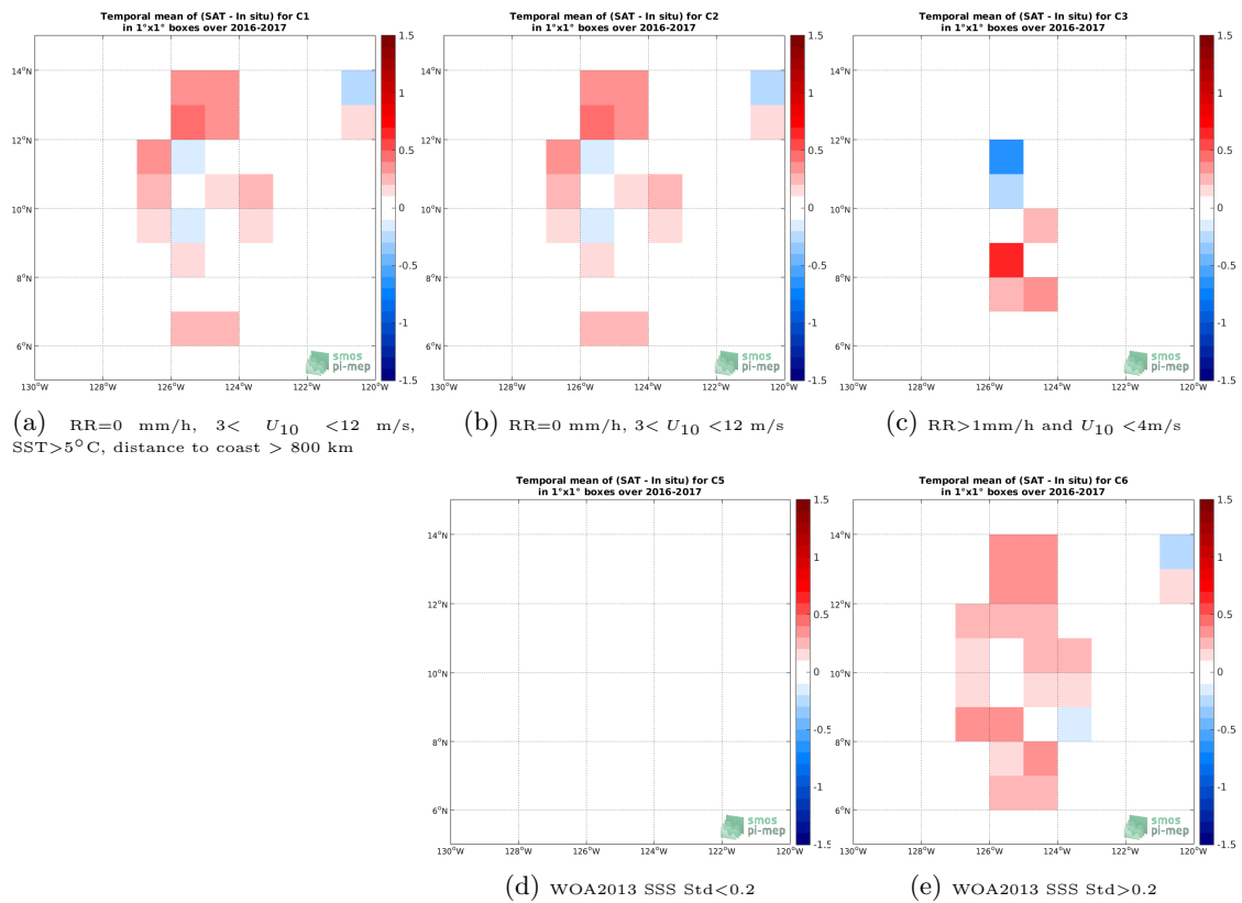
Figure 12: Temporal mean gridded over spatial boxes of size 1^\circ \times 1^\circ of \Delta SSS (SMAP SSS L2 v4 (RSS) - Salinity Snake) for 5 different subdatasets corresponding to:RR=0 mm/h, 3 < U_{10} < 12 m/s, SST >5^\circ\text{C} , distance to coast > 800 km (a), RR=0 mm/h, 3 < U_{10} < 12 m/s (b), RR >1 mm/h and U_{10} < 4 m/s (c), WOA2013 SSS Std <0.2 (d), WOA2013 SSS Std >0.2 (e).
