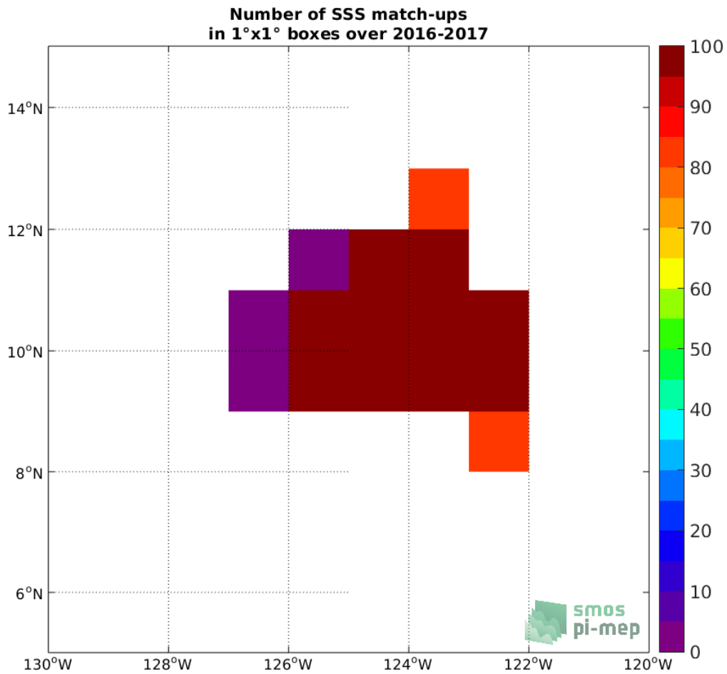
Figure 3: Number of SSS match-ups between Seaglider SSS and the SMAP SSS L2 v4 (RSS) SSS product for the SPURS 2 Pi-MEP region over 1°×1° boxes and for the full satellite product period.
