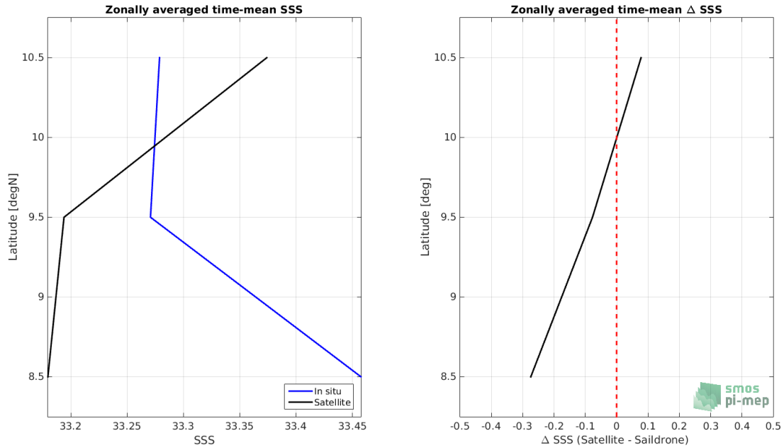
Figure 7: Left panel: Zonal mean SSS from SMAP SSS L2 v4 (RSS) satellite product (black) and from Sairdrone (blue). Right panel: Zonal mean of \Delta SSS (Satellite - Sairdrone) for all the collected Pi-MEP match-up pairs estimated over the full satellite product period.
