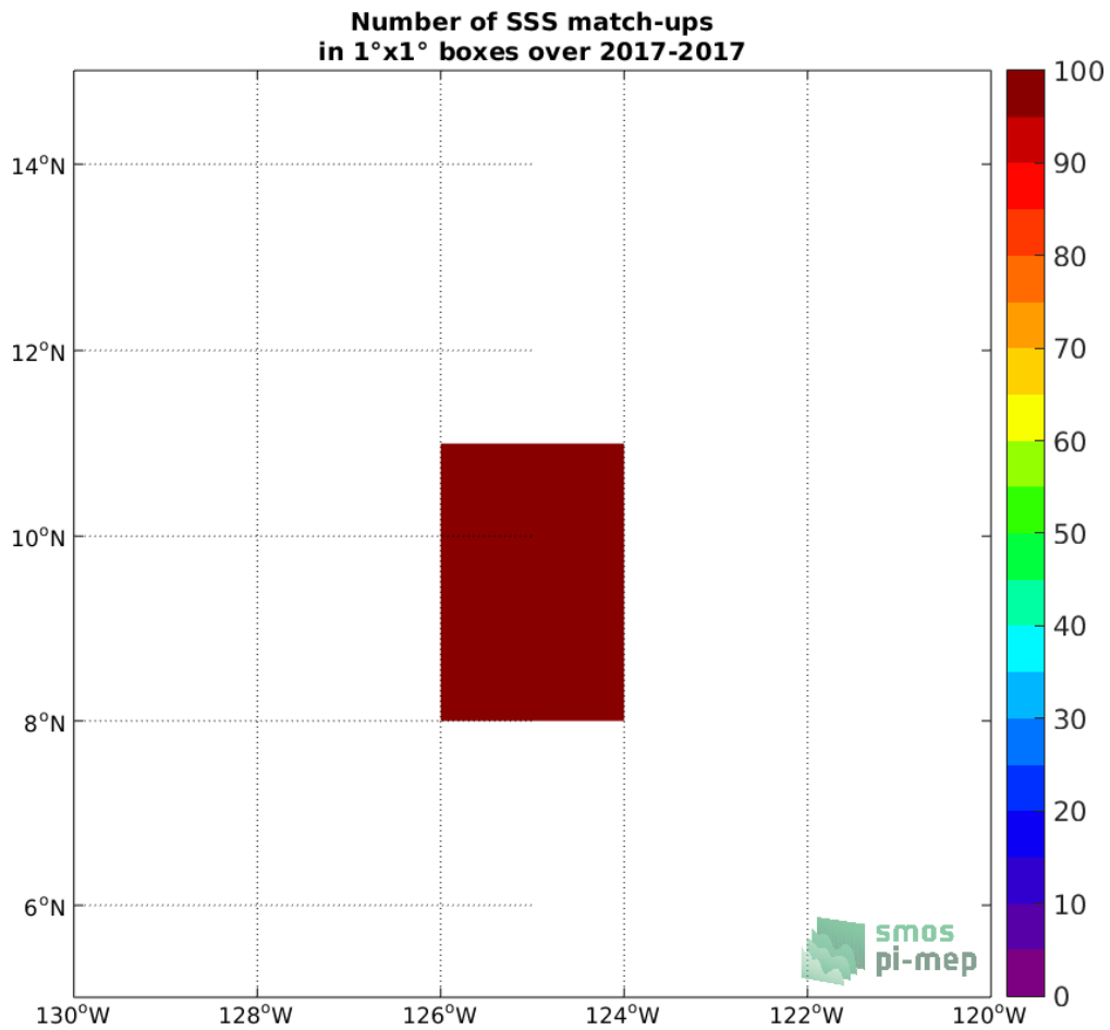
Figure 3: Number of SSS match-ups between Saildrone SSS and the SMAP SSS L2 v4 (RSS) SSS product for the SPURS 2 Pi-MEP region over 1°×1° boxes and for the full satellite product period.
