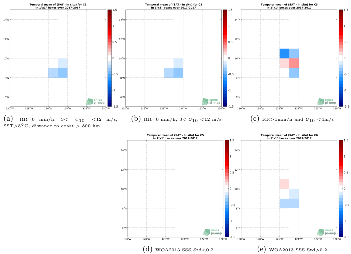
Figure 11: Temporal mean gridded over spatial boxes of size 1^\circ \times 1^\circ of \Delta\text{SSS} (SMAP SSS L2 v4 (RSS) - Saildrone) for 5 different subdatasets corresponding to:RR=0 mm/h, 3 < U_{10} < 12 m/s, SST >5^\circ\text{C} , distance to coast > 800 km (a), RR=0 mm/h, 3 < U_{10} < 12 m/s (b), RR >1 mm/h and U_{10} < 4 m/s (c), WOA2013 SSS Std <0.2 (d), WOA2013 SSS Std >0.2 (e).
