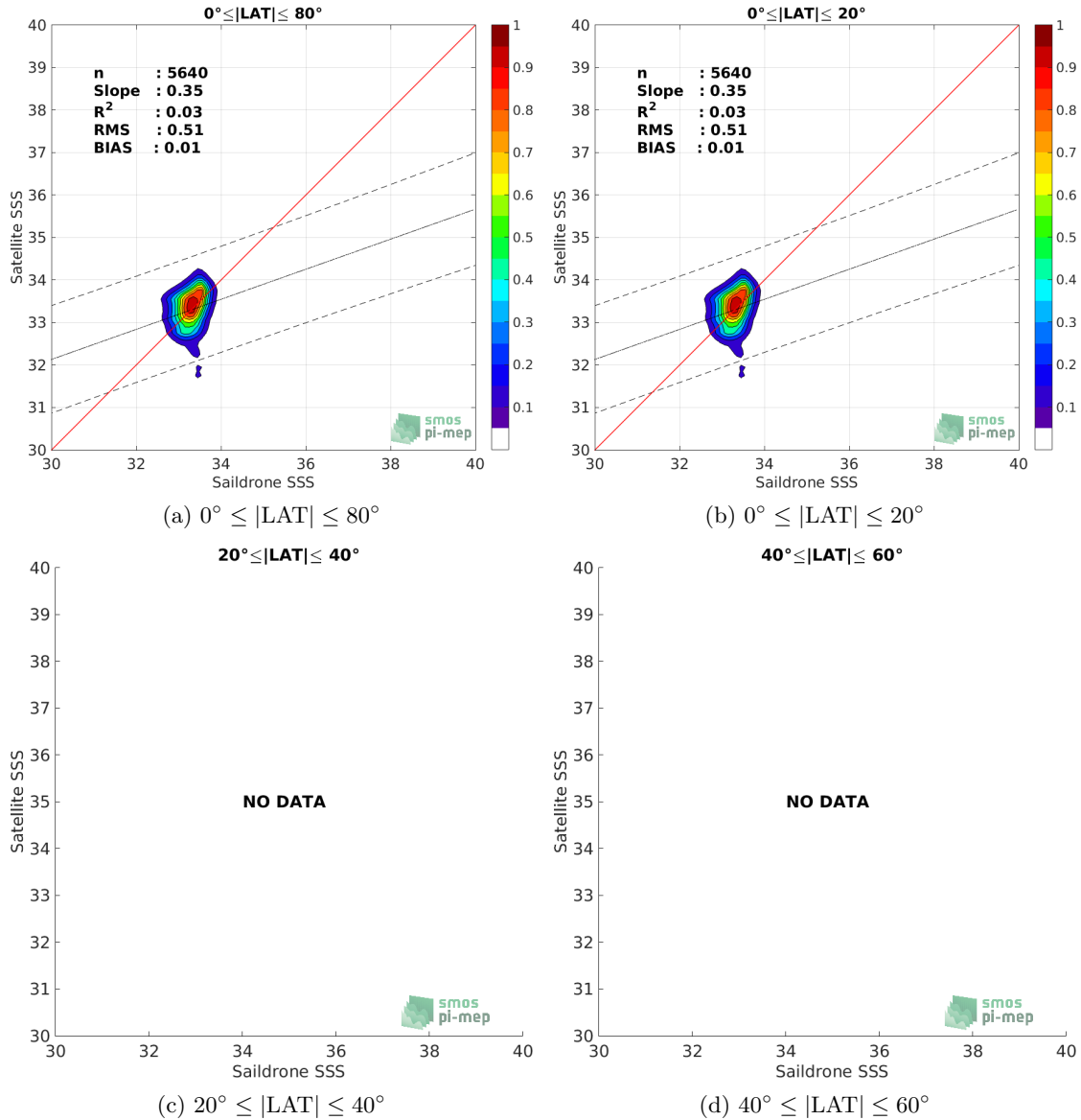
Figure 8: Contour maps of the concentration of SMAP SSS L2 v4 (RSS) SSS (y-axis) versus Saildrone SSS (x-axis) at match-up pairs for different latitude bands. For each plot, the red line shows x=y . The black thin and dashed lines indicate a linear fit through the data cloud and the \pm 95\% confidence levels, respectively. The number match-up pairs n , the slope and R^2 coefficient of the linear fit, the root mean square (RMS) and the mean bias between satellite and in situ data are indicated for each latitude band in each plots.
