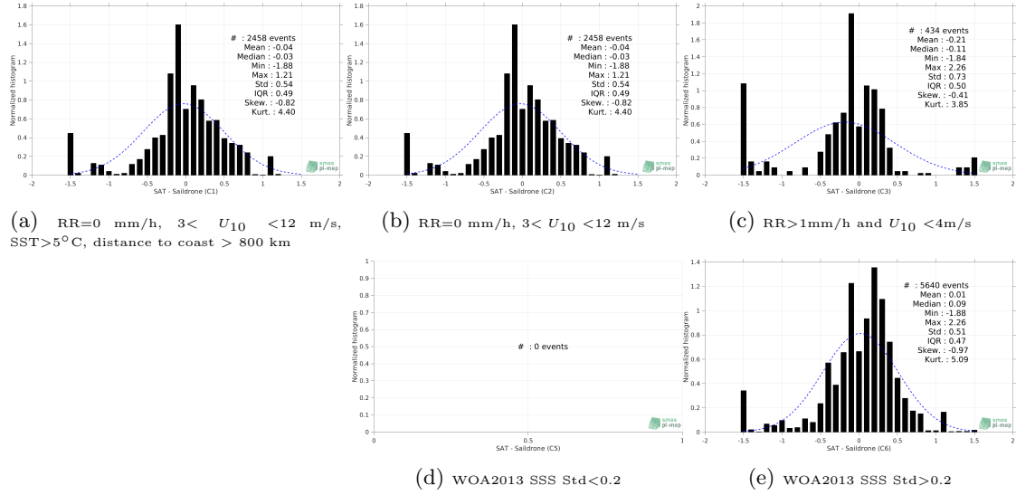
Figure 12: Normalized histogram of \Delta SSS (SMAP SSS L2 v4 (RSS) - Saildrone) for 5 different subdatasets corresponding to: RR=0 mm/h, 3 < U_{10} < 12 m/s, SST > 5°C, distance to coast > 800 km (a), RR=0 mm/h, 3 < U_{10} < 12 m/s (b), RR > 1mm/h and U_{10} < 4 m/s (c), WOA2013 SSS Std < 0.2 (d), WOA2013 SSS Std > 0.2 (e).
