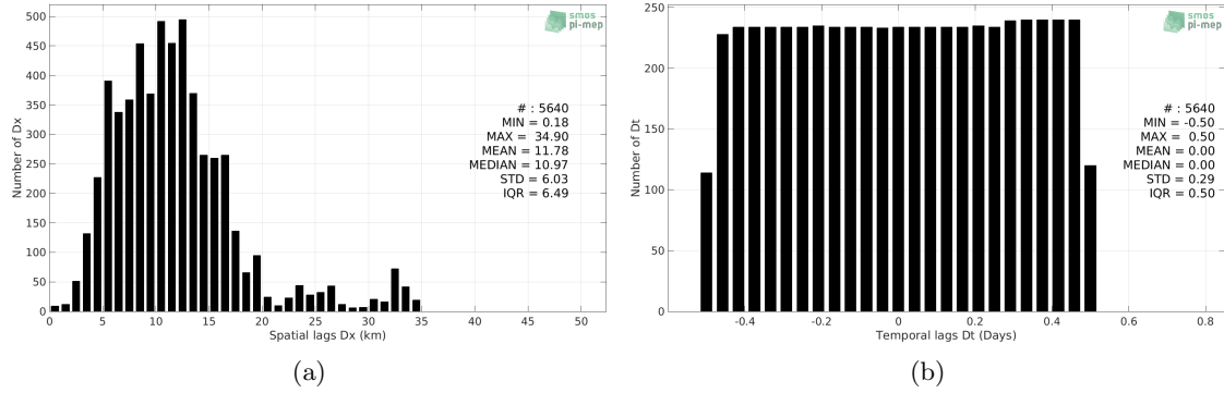
Figure 4: Histograms of the spatial (a) and temporal (b) lags between the location/time of the Sairdrone measurement and the date of the corresponding SMAP SSS L2 v4 (RSS) SSS pixel.
