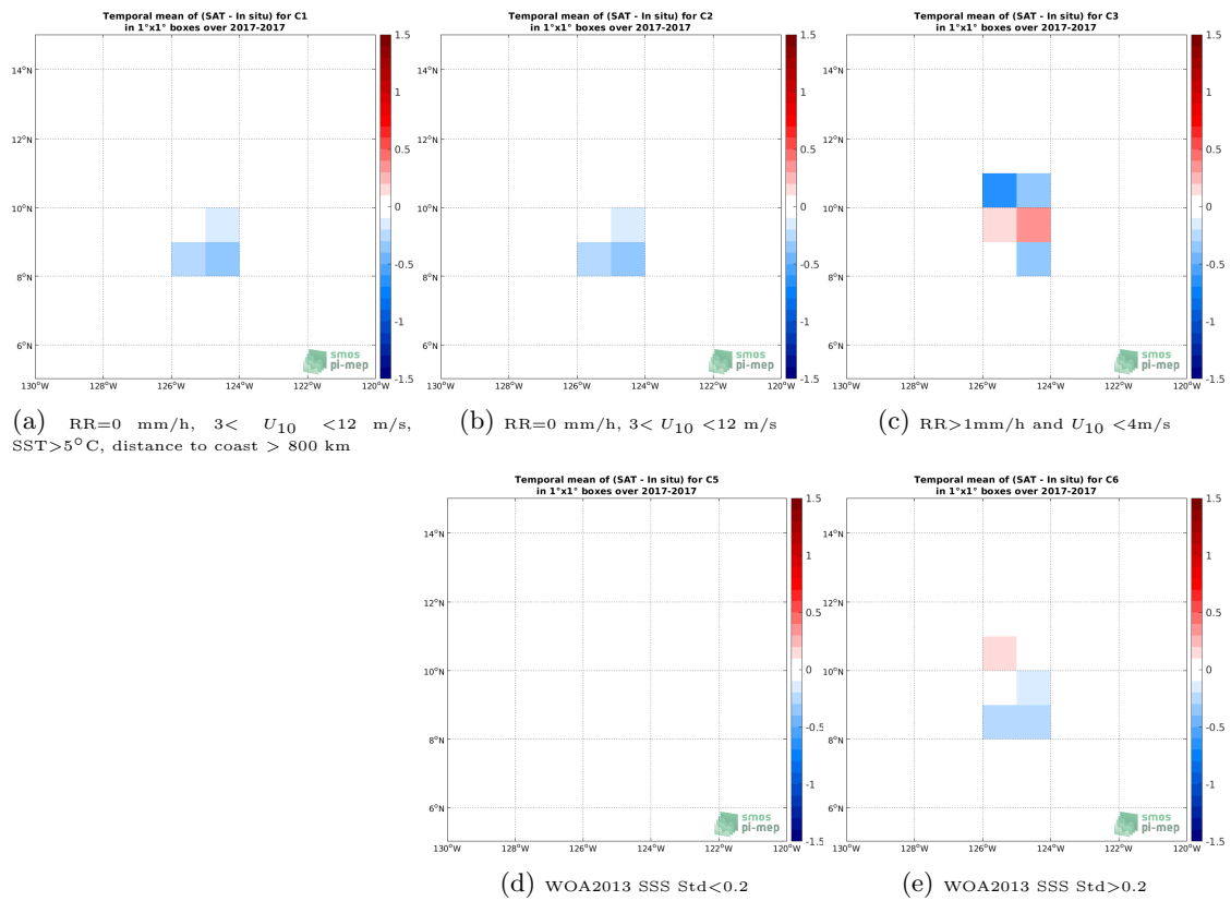
Figure 11: Temporal mean gridded over spatial boxes of size 1^\circ \times 1^\circ of \Delta SSS (SMAP SSS L2 v4 (RSS) - Saildrone) for 5 different subdatasets corresponding to:RR=0 mm/h, 3 < U_{10} < 12 m/s, SST >5^\circ\text{C} , distance to coast > 800 km (a), RR=0 mm/h, 3 < U_{10} < 12 m/s (b), RR >1 mm/h and U_{10} < 4 m/s (c), WOA2013 SSS Std <0.2 (d), WOA2013 SSS Std >0.2 (e).
