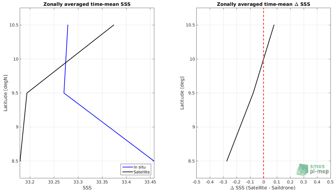
Figure 8: Left panel: Zonal mean SSS from SMAP SSS L2 v4 (RSS) satellite product (black) and from Sairdrone (blue). Right panel: Zonal mean of \Delta SSS (Satellite - Sairdrone) for all the collected Pi-MEP match-up pairs estimated over the full satellite product period.
