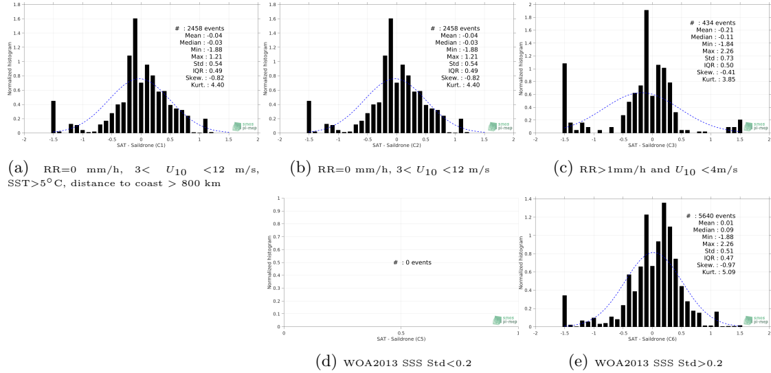
Figure 13: Normalized histogram of \Delta SSS (SMAP SSS L2 v4 (RSS) - Saildrone) for 5 different subdatasets corresponding to: RR=0 mm/h, 3 < U_{10} < 12 m/s, SST > 5°C, distance to coast > 800 km (a), RR=0 mm/h, 3 < U_{10} < 12 m/s (b), RR > 1mm/h and U_{10} < 4 m/s (c), WOA2013 SSS Std < 0.2 (d), WOA2013 SSS Std > 0.2 (e).
