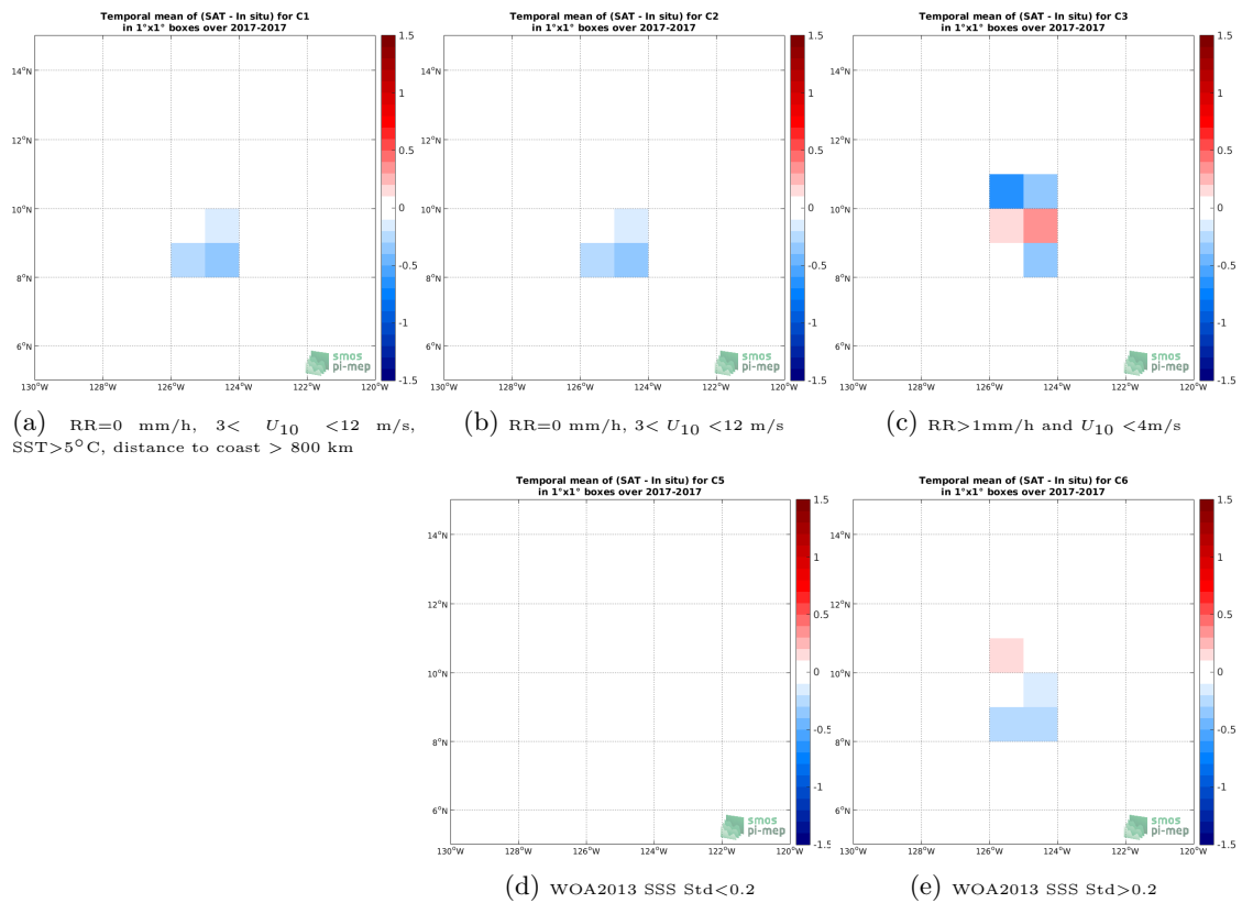
Figure 12: Temporal mean gridded over spatial boxes of size 1^\circ \times 1^\circ of \Delta SSS (SMAP SSS L2 v4 (RSS) - Saildrone) for 5 different subdatasets corresponding to: RR=0 mm/h, 3 < U_{10} < 12 m/s, SST > 5^\circ C , distance to coast > 800 km (a), RR=0 mm/h, 3 < U_{10} < 12 m/s (b), RR > 1 mm/h and U_{10} < 4 m/s (c), WOA2013 SSS Std < 0.2 (d), WOA2013 SSS Std > 0.2 (e).
