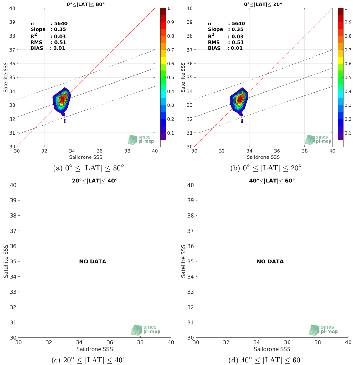
Figure 9: Contour maps of the concentration of SMAP SSS L2 v4 (RSS) SSS (y-axis) versus Saildrone SSS (x-axis) at match-up pairs for different latitude bands. For each plot, the red line shows x=y . The black thin and dashed lines indicate a linear fit through the data cloud and the \pm 95\% confidence levels, respectively. The number match-up pairs n , the slope and R^2 coefficient of the linear fit, the root mean square (RMS) and the mean bias between satellite and in situ data are indicated for each latitude band in each plots.
