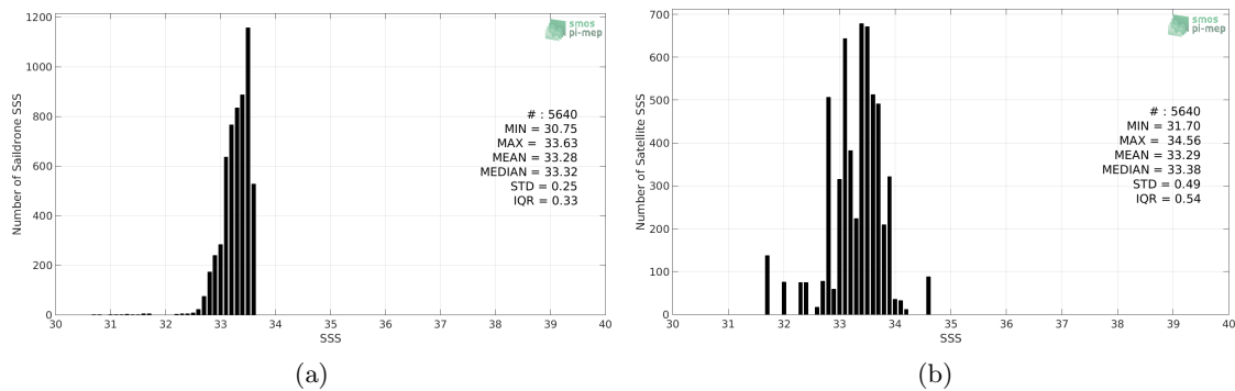
Figure 2: Histograms of SSS from Saildrone (a) and SMAP SSS L2 v4 (RSS) (b) considering all match-up pairs per bins of 0.1 over the SPURS 2 Pi-MEP region and for the full satellite product period.
