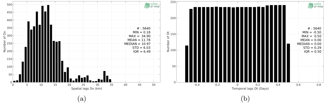
Figure 5: Histograms of the spatial (a) and temporal (b) lags between the time of the Sairdrone measurements and the date of the corresponding SMAP SSS L2 v4 (RSS) SSS product.
