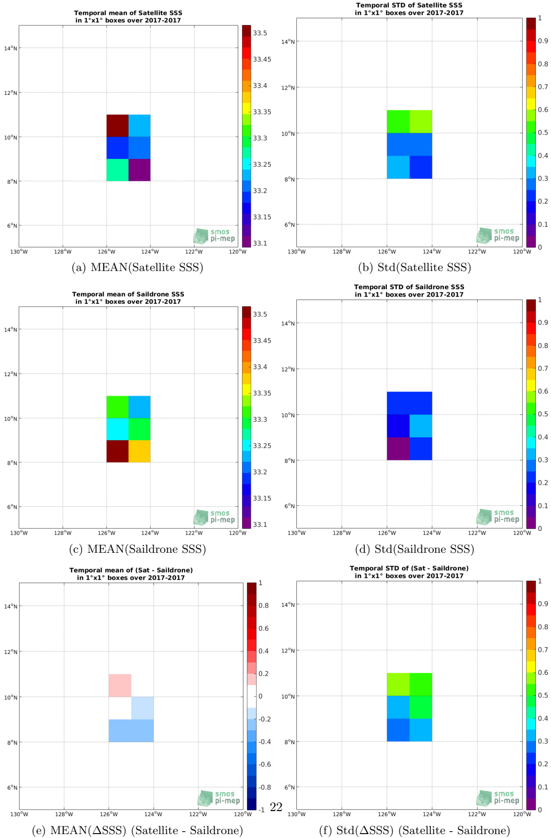
Figure 6: Temporal mean (left) and Std (right) of SSS from SMAP SSS L2 v4 (RSS) (top), Saildrone (middle), and of \Delta SSS (Satellite - Saildrone). Only match-up pairs are used to generate these maps.
