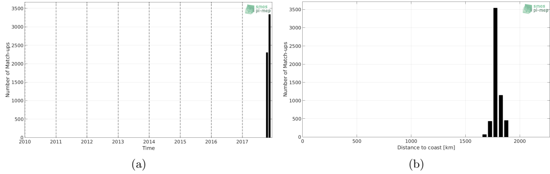
Figure 1: Number of match-ups between Saildrone and SMAP SSS L2 v4 (RSS) SSS as a function of time (a) and as function of the distance to coast (b) over the SPURS 2 Pi-MEP region and for the full satellite product period.
