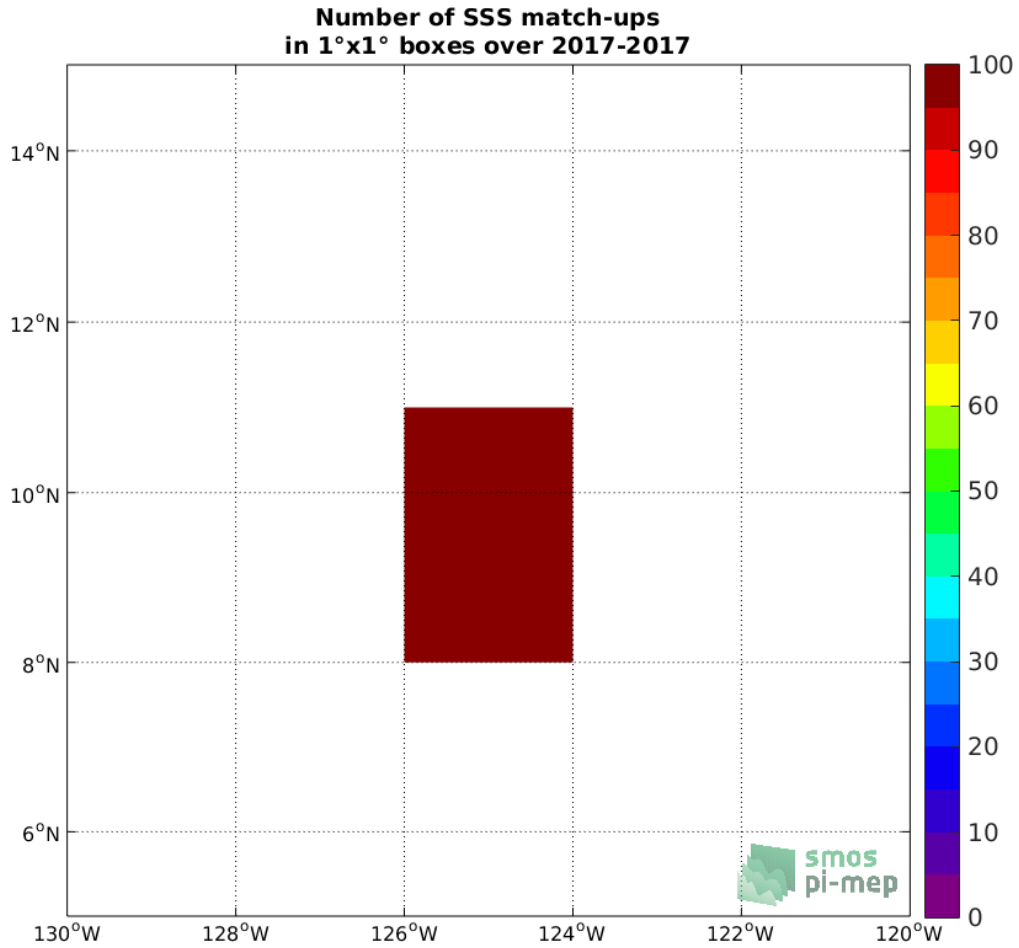
Figure 4: Number of SSS match-ups between Saildrone SSS and the SMAP SSS L2 v4 (RSS) SSS product for the SPURS 2 Pi-MEP region over 1°x1° boxes and for the full satellite product period.
