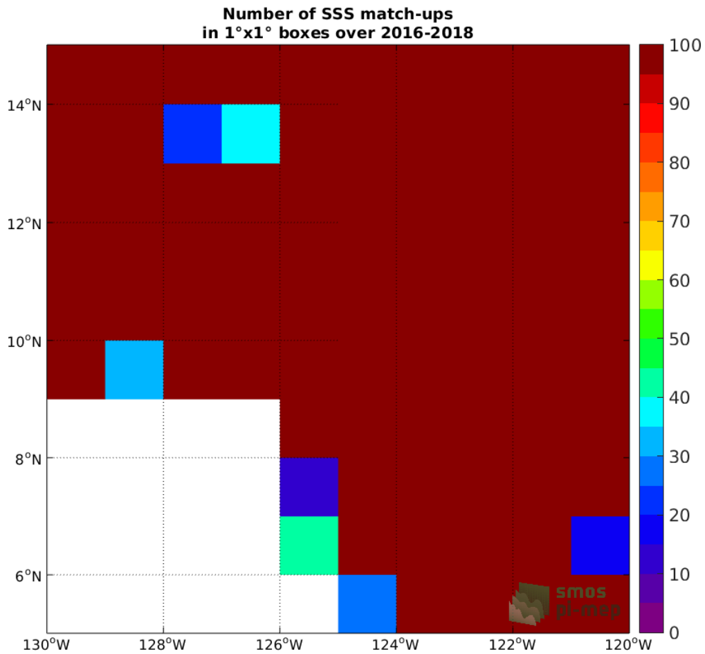
Figure 3: Number of SSS match-ups between Surface drifters SSS and the SMAP SSS L2 v4 (RSS) SSS product for the SPURS 2 Pi-MEP region over 1°x1° boxes and for the full satellite product period.
