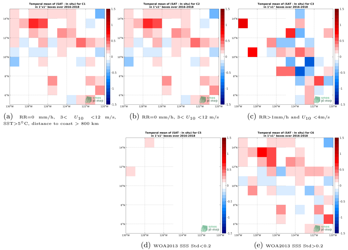
Figure 11: Temporal mean gridded over spatial boxes of size 1^\circ \times 1^\circ of \Delta SSS (SMAP SSS L2 v4 (RSS) - Surface drifters) for 5 different subdatasets corresponding to:RR=0 mm/h, 3 < U_{10} < 12 m/s, SST >5^\circ\text{C} , distance to coast > 800 km (a), RR=0 mm/h, 3 < U_{10} < 12 m/s (b), RR >1 mm/h and U_{10} < 4 m/s (c), WOA2013 SSS Std <0.2 (d), WOA2013 SSS Std >0.2 (e).
