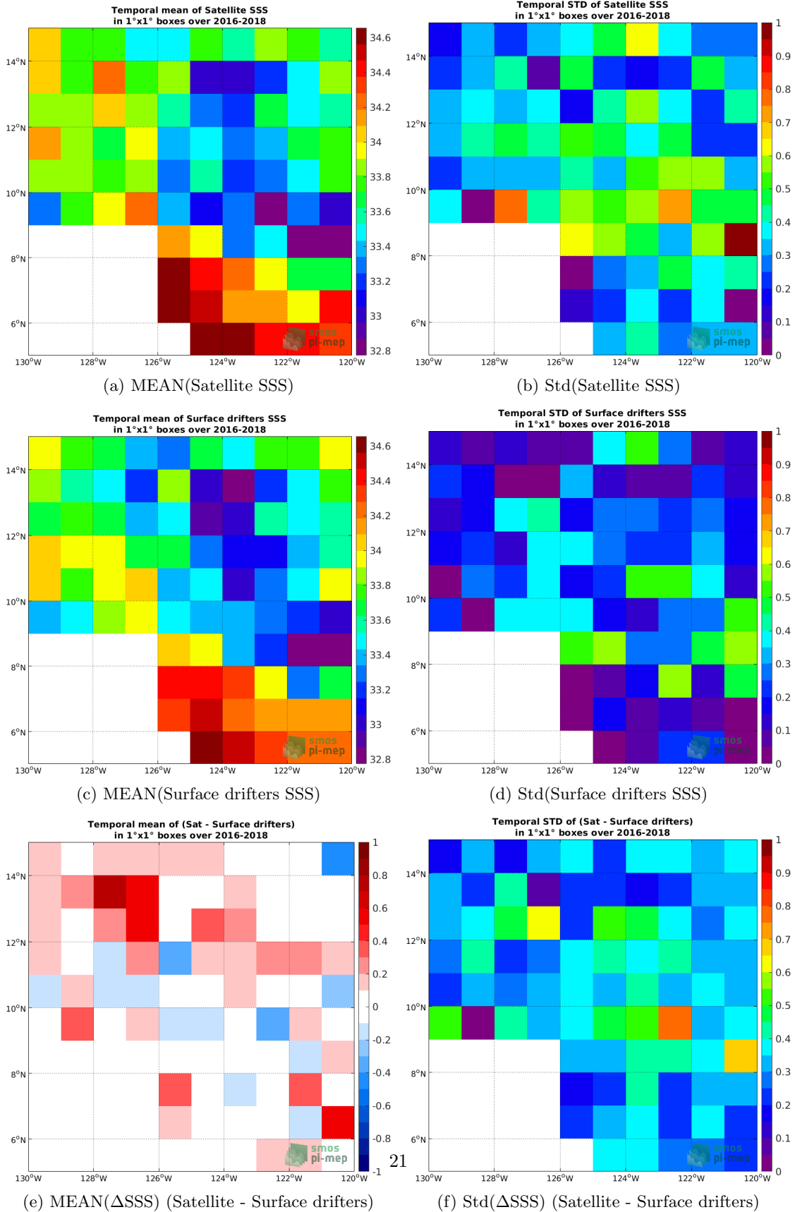
Figure 5: Temporal mean (left) and Std (right) of SSS from SMAP SSS L2 v4 (RSS) (top), Surface drifters (middle), and of \Delta SSS (Satellite - Surface drifters). Only match-up pairs are used to generate these maps.
