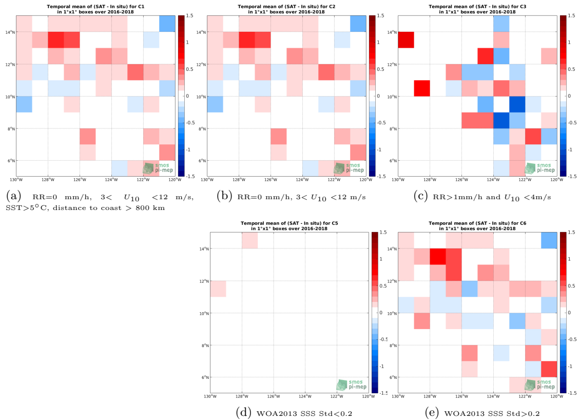
Figure 11: Temporal mean gridded over spatial boxes of size 1^\circ \times 1^\circ of \Delta SSS (SMAP-L2-RSS-V4 - Surface drifters) for 5 different subdatasets corresponding to:RR=0 mm/h, 3 < U_{10} < 12 m/s, SST >5^\circ\text{C} , distance to coast > 800 km (a), RR=0 mm/h, 3 < U_{10} < 12 m/s (b), RR >1 mm/h and U_{10} < 4 m/s (c), WOA2013 SSS Std <0.2 (d), WOA2013 SSS Std >0.2 (e).
