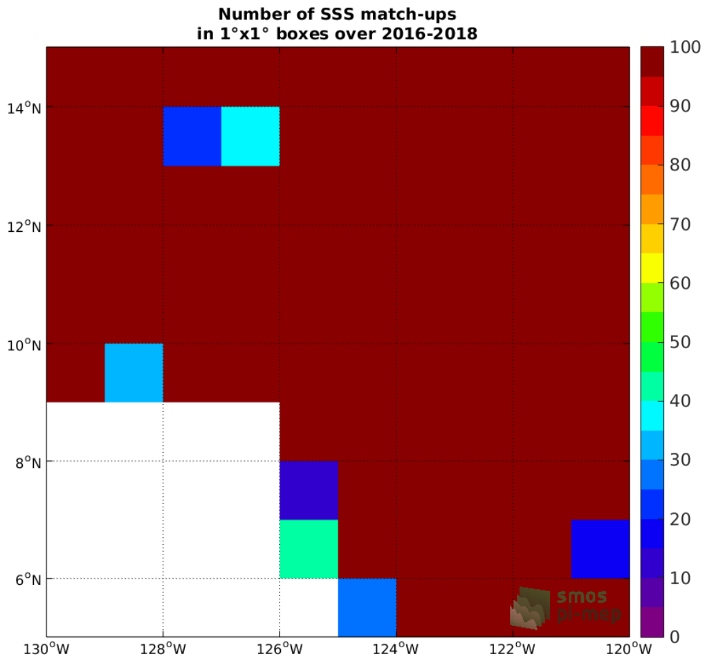
Figure 3: Number of SSS match-ups between Surface drifters SSS and the SMAP-L2-RSS-V4 SSS product for the SPURS 2 Pi-MEP region over 1°x1° boxes and for the full satellite product period.
