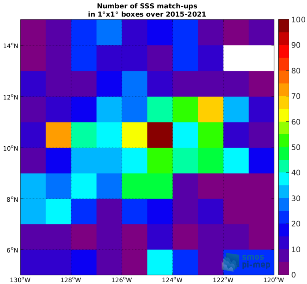
Figure 4: Number of SSS match-ups between Argo SSS and the SMAP SSS L2 v4 (RSS) SSS product for the SPURS 2 Pi-MEP region over 1°×1° boxes and for the full satellite product period.
