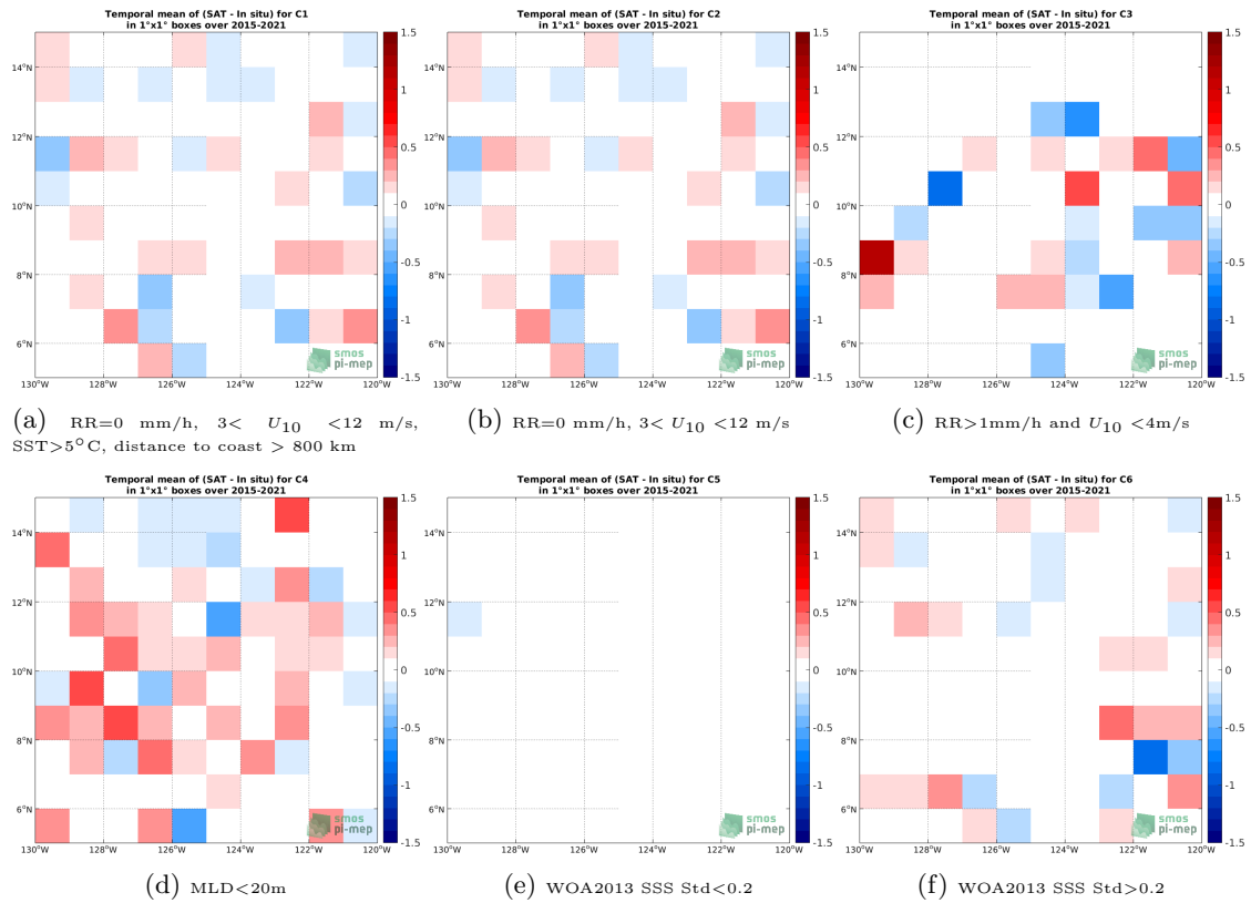
Figure 12: Temporal mean gridded over spatial boxes of size 1^\circ \times 1^\circ of \Delta SSS (SMAP SSS L2 v4 (RSS) - Argo) for 6 different subdatasets corresponding to:RR=0 mm/h, 3 < U_{10} < 12 m/s, SST >5^\circ C, distance to coast > 800 km (a), RR=0 mm/h, 3 < U_{10} < 12 m/s (b), RR >1 mm/h and U_{10} < 4 m/s (c),MLD <20 m (d),WOA2013 SSS Std <0.2 (e),WOA2013 SSS Std >0.2 (f).
