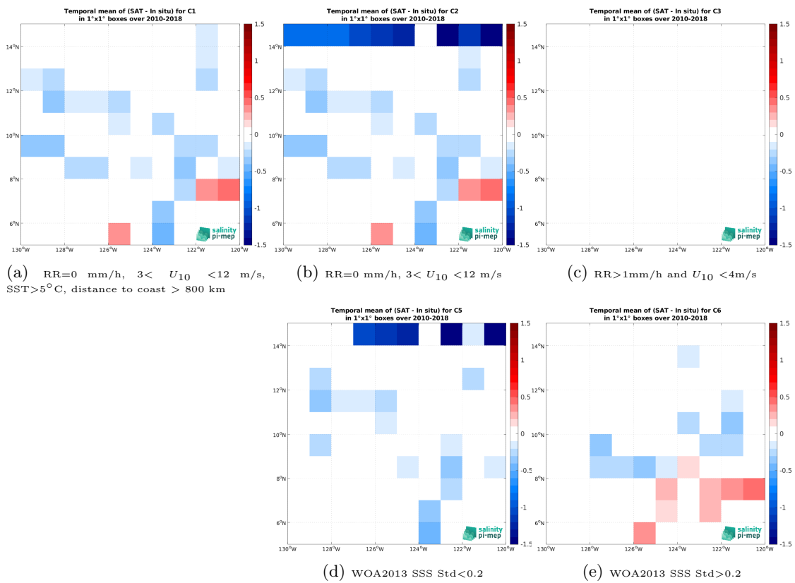
Figure 14: Temporal mean gridded over spatial boxes of size 1^\circ \times 1^\circ of \Delta\text{SSS} (CCI SSS L4 Merged-OI v4.41 - 30-day running (ESA) - TSG (SAMOS)) for 5 different subdatasets corresponding to:RR=0 mm/h, 3 < U_{10} < 12 m/s, SST>5°C, distance to coast > 800 km (a), RR=0 mm/h, 3 < U_{10} < 12 m/s (b), RR>1mm/h and U_{10} < 4 m/s (c), WOA2013 SSS Std<0.2 (d), WOA2013 SSS Std>0.2 (e).
