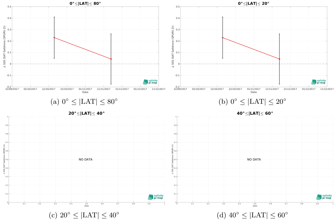
Figure 11: Monthly median (red curves) of \Delta SSS (Satellite - Sairdrome (SPURS 2)) and \pm 1 Std (black vertical thick bars) as function of time for all the collected Pi-MEP match-up pairs estimated over the SPURS 2 Pi-MEP region and for the full satellite product period are shown for different latitude bands: (a) 80^\circ\text{S}-80^\circ\text{N} , (b) 20^\circ\text{S}-20^\circ\text{N} , (c) 40^\circ\text{S}-20^\circ\text{S} and 20^\circ\text{N}-40^\circ\text{N} and (d) 60^\circ\text{S}-40^\circ\text{S} and 40^\circ\text{N}-60^\circ\text{N} .
