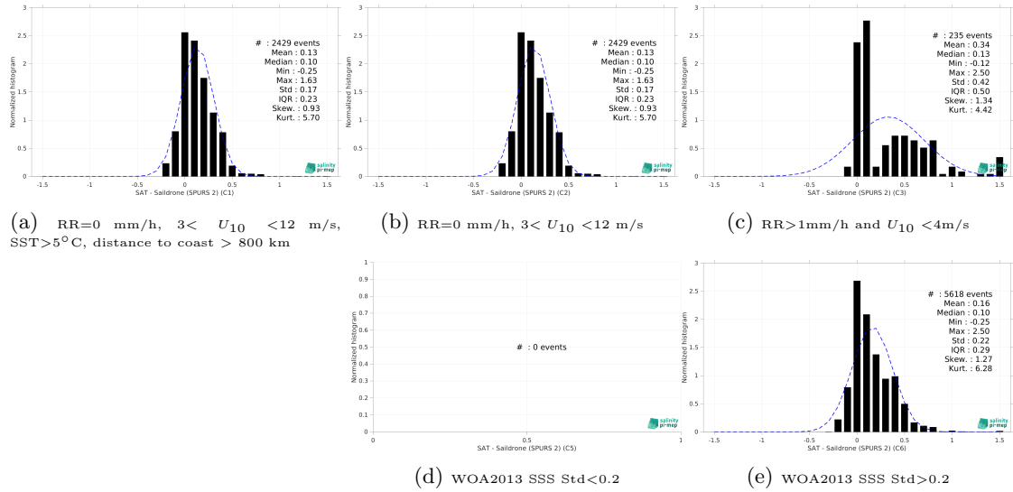
Figure 15: Normalized histogram of \Delta SSS (CCI SSS L4 Merged-OI v4.41 - 30-day running (ESA) - Saildrone (SPURS 2)) for 5 different subdatasets corresponding to: RR=0 mm/h, 3 < U_{10} < 12 m/s, SST>5°C, distance to coast > 800 km (a), RR=0 mm/h, 3 < U_{10} < 12 m/s (b), RR>1mm/h and U_{10} < 4 m/s (c), WOA2013 SSS Std<0.2 (d), WOA2013 SSS Std>0.2 (e).
