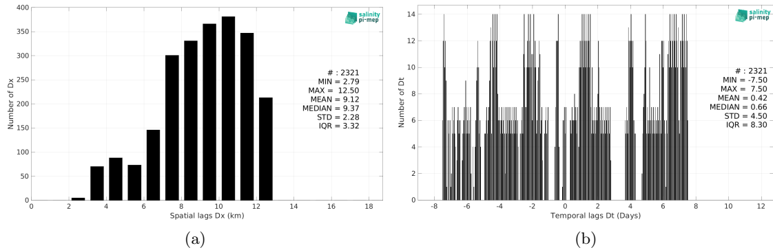
Figure 6: Histograms of the spatial (a) and temporal (b) lags between the location/time of the Saildrone (SPURS 2) measurement and the date of the corresponding CCI SSS L4 Merged-OI v4.41 - 30-day running (ESA) SSS pixel.
