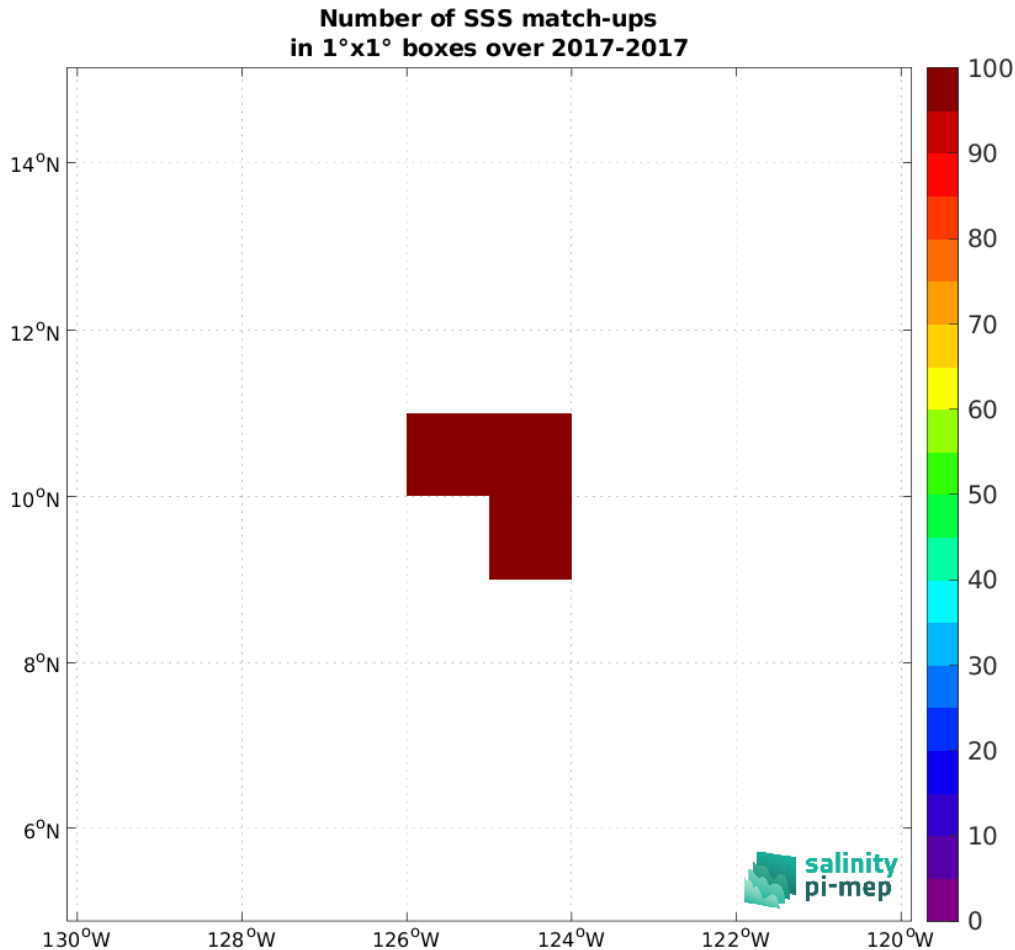
Figure 5: Number of SSS match-ups between Saildrone (SPURS 2) SSS and the CCI SSS L4 Merged-OI v4.41 - 30-day running (ESA) SSS product for the SPURS 2 Pi-MEP region over 1^\circ \times 1^\circ boxes and for the full satellite product period.
