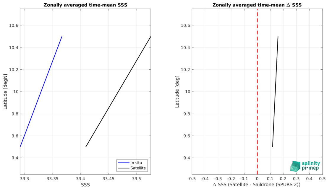
Figure 9: Left panel: Zonal mean SSS from CCI SSS L4 Merged-OI v4.41 - 30-day running (ESA) satellite product (black) and from Sairdron (SPURS 2) (blue). Right panel: Zonal mean of \Delta SSS (Satellite - Sairdron (SPURS 2)) for all the collected Pi-MEP match-up pairs estimated over the full satellite product period.
