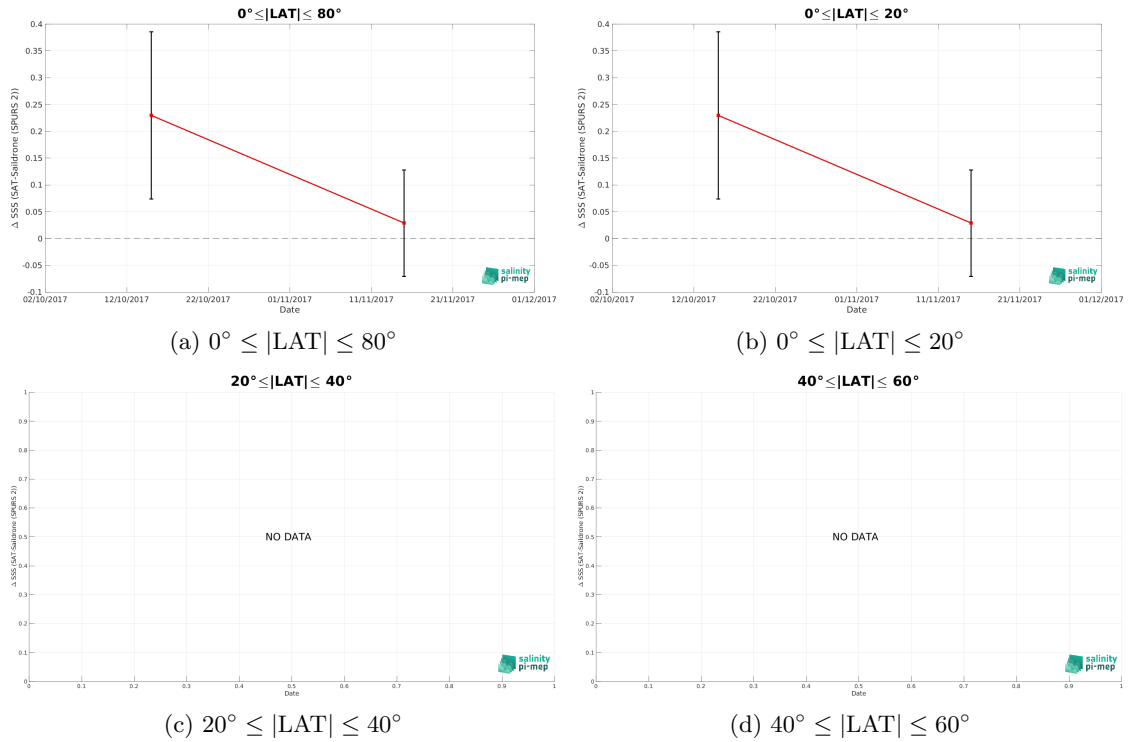
Figure 11: Monthly median (red curves) of \Delta SSS (Satellite - Sailability (SPURS 2)) and \pm 1 Std (black vertical thick bars) as function of time for all the collected Pi-MEP match-up pairs estimated over the SPURS 2 Pi-MEP region and for the full satellite product period are shown for different latitude bands: (a) 80^\circ\text{S}-80^\circ\text{N} , (b) 20^\circ\text{S}-20^\circ\text{N} , (c) 40^\circ\text{S}-20^\circ\text{S} and 20^\circ\text{N}-40^\circ\text{N} and (d) 60^\circ\text{S}-40^\circ\text{S} and 40^\circ\text{N}-60^\circ\text{N} .
