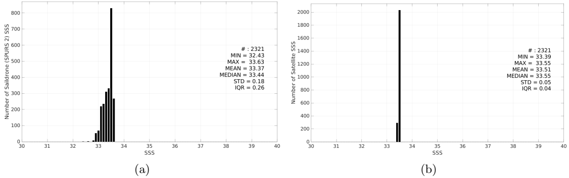
Figure 3: Histograms of SSS from Saildrone (SPURS 2) (a) and CCI SSS L4 Merged-OI v4.41 - 30-day running (ESA) (b) considering all match-up pairs per bins of 0.1 over the SPURS 2 Pi-MEP region and for the full satellite product period.
