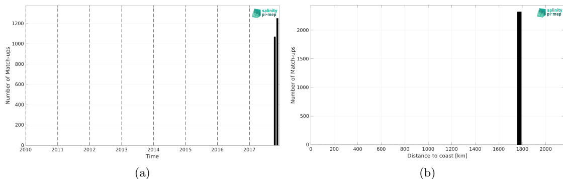
Figure 2: Number of match-ups between Saildrone (SPURS 2) and CCI SSS L4 Merged-OI v4.41 - 30-day running (ESA) SSS as a function of time (a) and as function of the distance to coast (b) over the SPURS 2 Pi-MEP region and for the full satellite product period.
