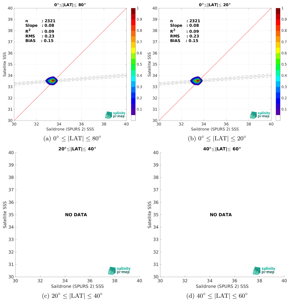
Figure 10: Contour maps of the concentration of CCI SSS L4 Merged-OI v4.41 - 30-day running (ESA) SSS (y-axis) versus Saildrone (SPURS 2) SSS (x-axis) at match-up pairs for different latitude bands. For each plot, the red line shows x=y . The black thin and dashed lines indicate a linear fit through the data cloud and the \pm 95\% confidence levels, respectively. The number match-up pairs n , the slope and R^2 coefficient of the linear fit, the root mean square (RMS) and the mean bias between satellite and in situ data are indicated for each latitude band in each plots.
