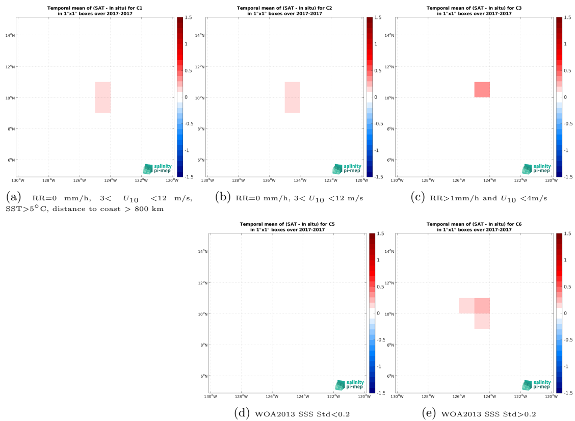
Figure 14: Temporal mean gridded over spatial boxes of size 1^\circ \times 1^\circ of \Delta SSS (CCI SSS L4 Merged-OI v4.41 - 30-day running (ESA) - Saildrone (SPURS 2)) for 5 different subdatasets corresponding to:RR=0 mm/h, 3 < U_{10} < 12 m/s, SST >5^\circ C, distance to coast > 800 km (a), RR=0 mm/h, 3 < U_{10} < 12 m/s (b), RR >1 mm/h and U_{10} < 4 m/s (c), WOA2013 SSS Std <0.2 (d), WOA2013 SSS Std >0.2 (e).
