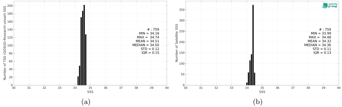
Figure 2: Histograms of SSS from TSG (GOSUD-Research-vessel) (a) and CCI SSS L4 Merged-OI v4.4 - 30-day running (ESA) (b) considering all match-up pairs per bins of 0.1 over the SPURS 2 Pi-MEP region and for the full satellite product period.
