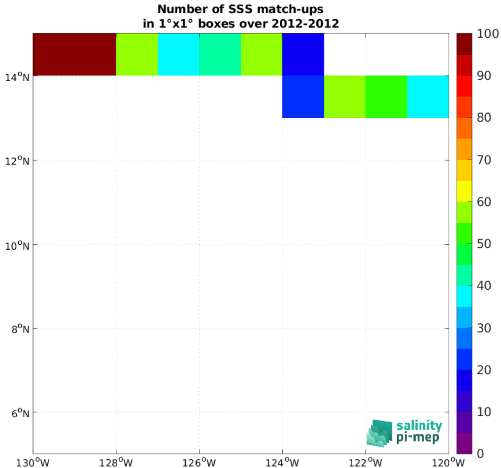
Figure 4: Number of SSS match-ups between TSG (GOSUD-Research-vessel) SSS and the CCI SSS L4 Merged-OI v4.4 - 30-day running (ESA) SSS product for the SPURS 2 Pi-MEP region over 1^\circ \times 1^\circ boxes and for the full satellite product period.
