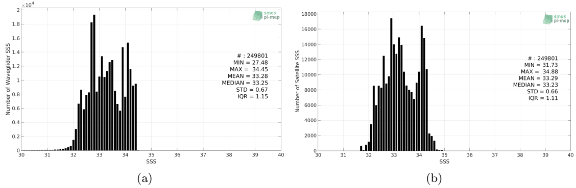
Figure 2: Histograms of SSS from Waveglider (a) and CCI SSS L4 Merged-OI v2.31 - 7-day running (ESA) (b) considering all match-up pairs per bins of 0.1 over the SPURS 2 Pi-MEP region and for the full satellite product period.
