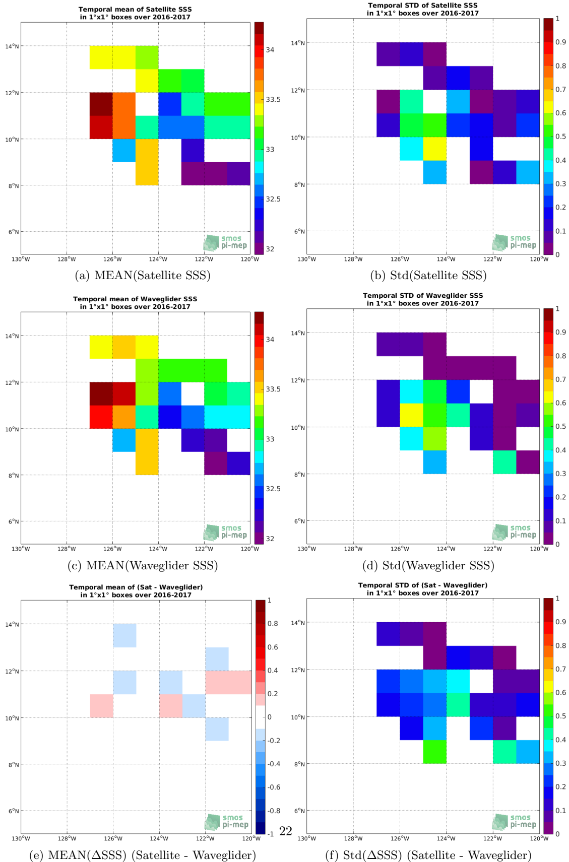
Figure 6: Temporal mean (left) and Std (right) of SSS from CCI SSS L4 Merged-OI v2.31 - 7-day running (ESA) (top), Waveglider (middle), and of \Delta SSS (Satellite - Waveglider). Only match-up pairs are used to generate these maps.
