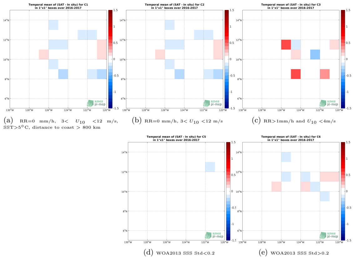
Figure 12: Temporal mean gridded over spatial boxes of size 1^\circ \times 1^\circ of \Delta SSS (CCI SSS L4 Merged-OI v2.31 - 7-day running (ESA) - Waveglider) for 5 different subdatasets corresponding to:RR=0 mm/h, 3 < U_{10} < 12 m/s, SST >5^\circ\text{C} , distance to coast > 800 km (a), RR=0 mm/h, 3 < U_{10} < 12 m/s (b), RR >1 mm/h and U_{10} < 4 m/s (c), WOA2013 SSS Std <0.2 (d), WOA2013 SSS Std >0.2 (e).
