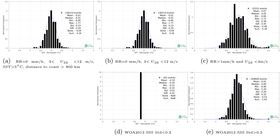
Figure 13: Normalized histogram of \Delta SSS (CCI SSS L4 Merged-OI v2.31 - 7-day running (ESA) - Waveglider) for 5 different subdatasets corresponding to: RR=0 mm/h, 3 < U_{10} < 12 m/s, SST > 5°C, distance to coast > 800 km (a), RR=0 mm/h, 3 < U_{10} < 12 m/s (b), RR > 1mm/h and U_{10} < 4 m/s (c), WOA2013 SSS Std < 0.2 (d), WOA2013 SSS Std > 0.2 (e).
