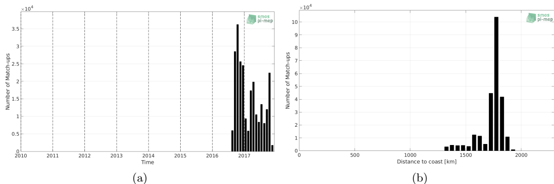
Figure 1: Number of match-ups between Waveglider and CCI SSS L4 Merged-OI v2.31 - 7-day running (ESA) SSS as a function of time (a) and as function of the distance to coast (b) over the SPURS 2 Pi-MEP region and for the full satellite product period.
