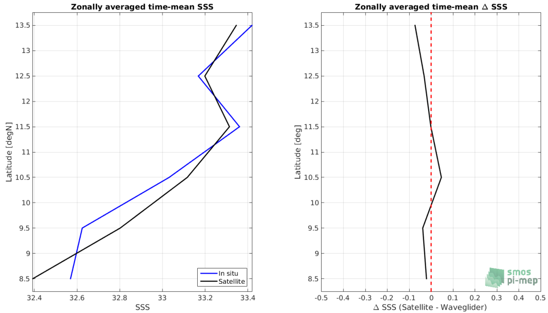
Figure 8: Left panel: Zonal mean SSS from CCI SSS L4 Merged-OI v2.31 - 7-day running (ESA) satellite product (black) and from Waveglider (blue). Right panel: Zonal mean of \Delta SSS (Satellite - Waveglider) for all the collected Pi-MEP match-up pairs estimated over the full satellite product period.
