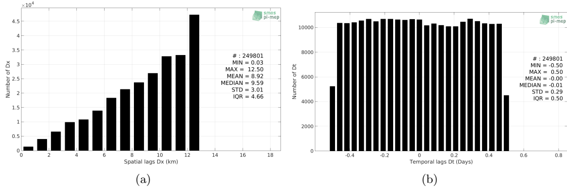
Figure 5: Histograms of the spatial (a) and temporal (b) lags between the time of the Waveglider measurements and the date of the corresponding CCI SSS L4 Merged-OI v2.31 - 7-day running (ESA) SSS product.
