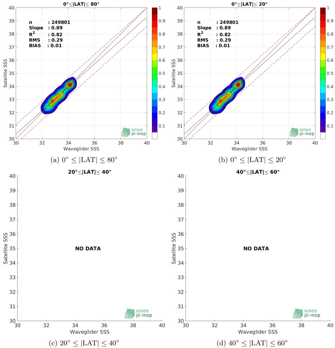
Figure 9: Contour maps of the concentration of CCI SSS L4 Merged-OI v2.31 - 7-day running (ESA) SSS (y-axis) versus Waveglider SSS (x-axis) at match-up pairs for different latitude bands. For each plot, the red line shows x=y . The black thin and dashed lines indicate a linear fit through the data cloud and the \pm 95\% confidence levels, respectively. The number match-up pairs n , the slope and R^2 coefficient of the linear fit, the root mean square (RMS) and the mean bias between satellite and in situ data are indicated for each latitude band in each plots.
