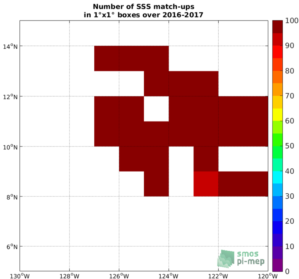
Figure 4: Number of SSS match-ups between Waveglider SSS and the CCI SSS L4 Merged-OI v2.31 - 7-day running (ESA) SSS product for the SPURS 2 Pi-MEP region over 1°x1° boxes and for the full satellite product period.
