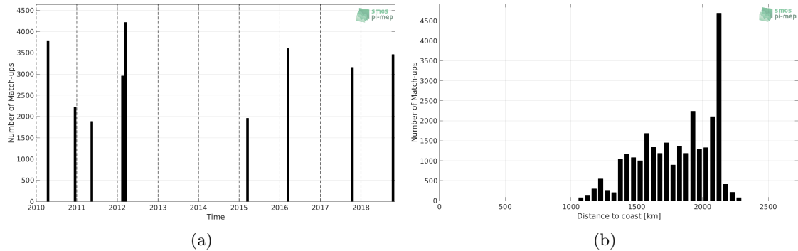
Figure 1: Number of match-ups between TSG (SAMOS) and CCI SSS L4 Merged-OI v2.31 - 7-day running (ESA) SSS as a function of time (a) and as function of the distance to coast (b) over the SPURS 2 Pi-MEP region and for the full satellite product period.
