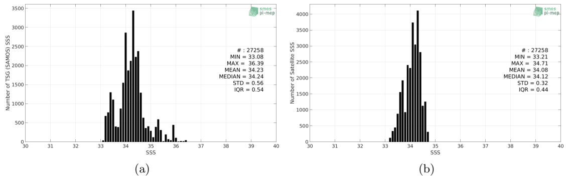
Figure 2: Histograms of SSS from TSG (SAMOS) (a) and CCI SSS L4 Merged-OI v2.31 - 7-day running (ESA) (b) considering all match-up pairs per bins of 0.1 over the SPURS 2 Pi-MEP region and for the full satellite product period.
