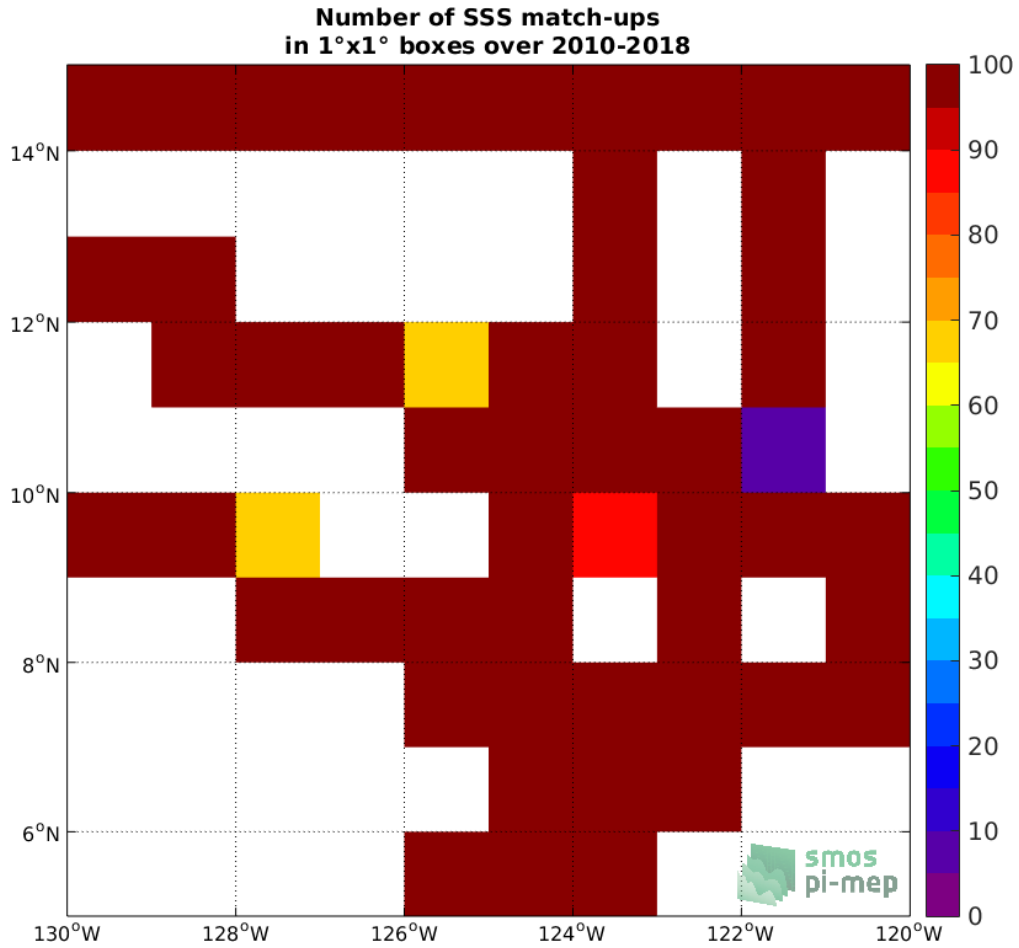
Figure 4: Number of SSS match-ups between TSG (SAMOS) SSS and the CCI SSS L4 Merged-OI v2.31 - 7-day running (ESA) SSS product for the SPURS 2 Pi-MEP region over 1°x1° boxes and for the full satellite product period.
