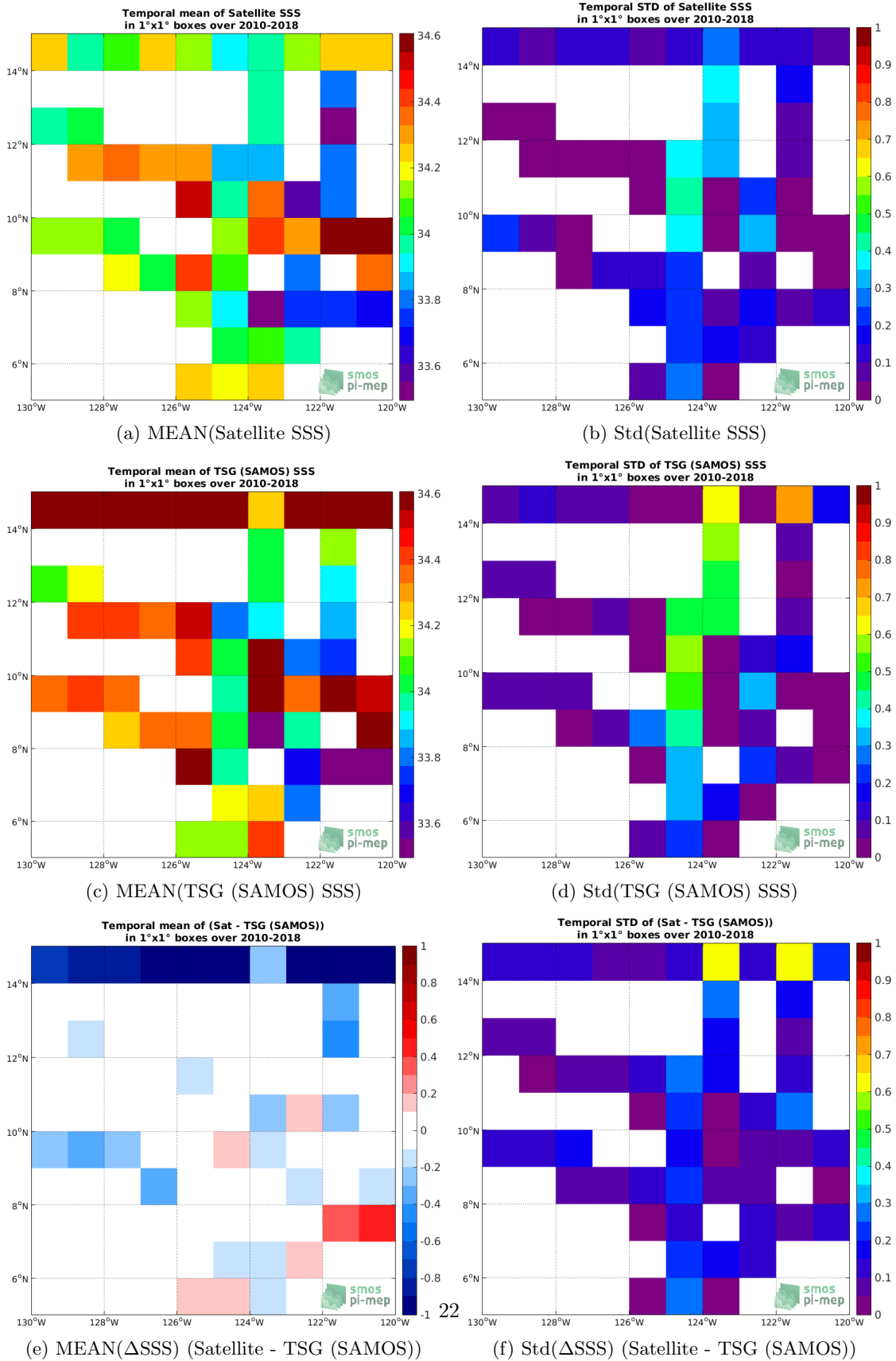
Figure 6: Temporal mean (left) and Std (right) of SSS from CCI SSS L4 Merged-OI v2.31 - 7-day running (ESA) (top), TSG (SAMOS) (middle), and of \Delta SSS (Satellite - TSG (SAMOS)). Only match-up pairs are used to generate these maps.
