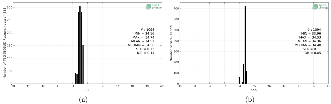
Figure 2: Histograms of SSS from TSG (GOSUD-Research-vessel) (a) and CCI L4 Merged-OI v2.31 - 7-day running (ESA) (b) considering all match-up pairs per bins of 0.1 over the SPURS 2 Pi-MEP region and for the full satellite product period.
