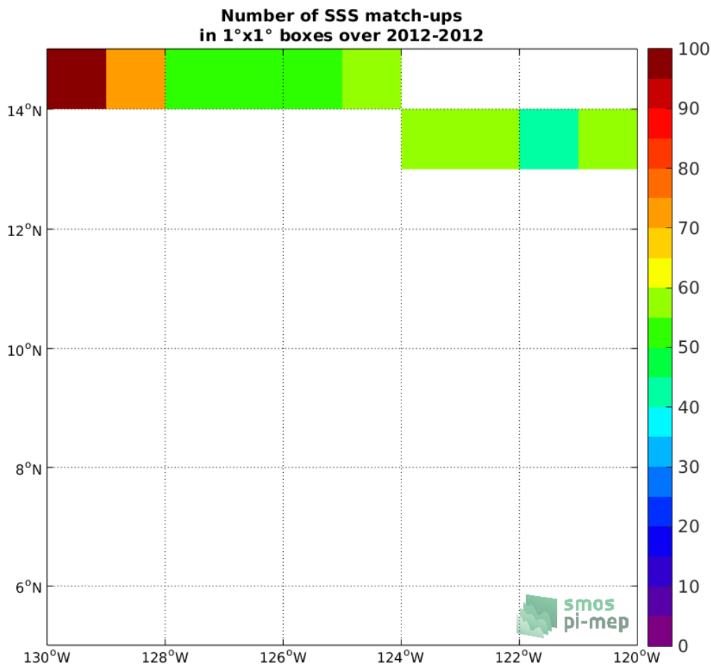
Figure 4: Number of SSS match-ups between TSG (GOSUD-Research-vessel) SSS and the CCI L4 Merged-OI v2.31 - 7-day running (ESA) SSS product for the SPURS 2 Pi-MEP region over 1°x1° boxes and for the full satellite product period.
