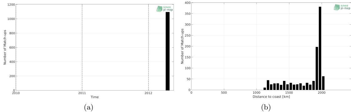
Figure 1: Number of match-ups between TSG (GOSUD-Research-vessel) and CCI L4 Merged-OI v2.31 - 7-day running (ESA) SSS as a function of time (a) and as function of the distance to coast (b) over the SPURS 2 Pi-MEP region and for the full satellite product period.
