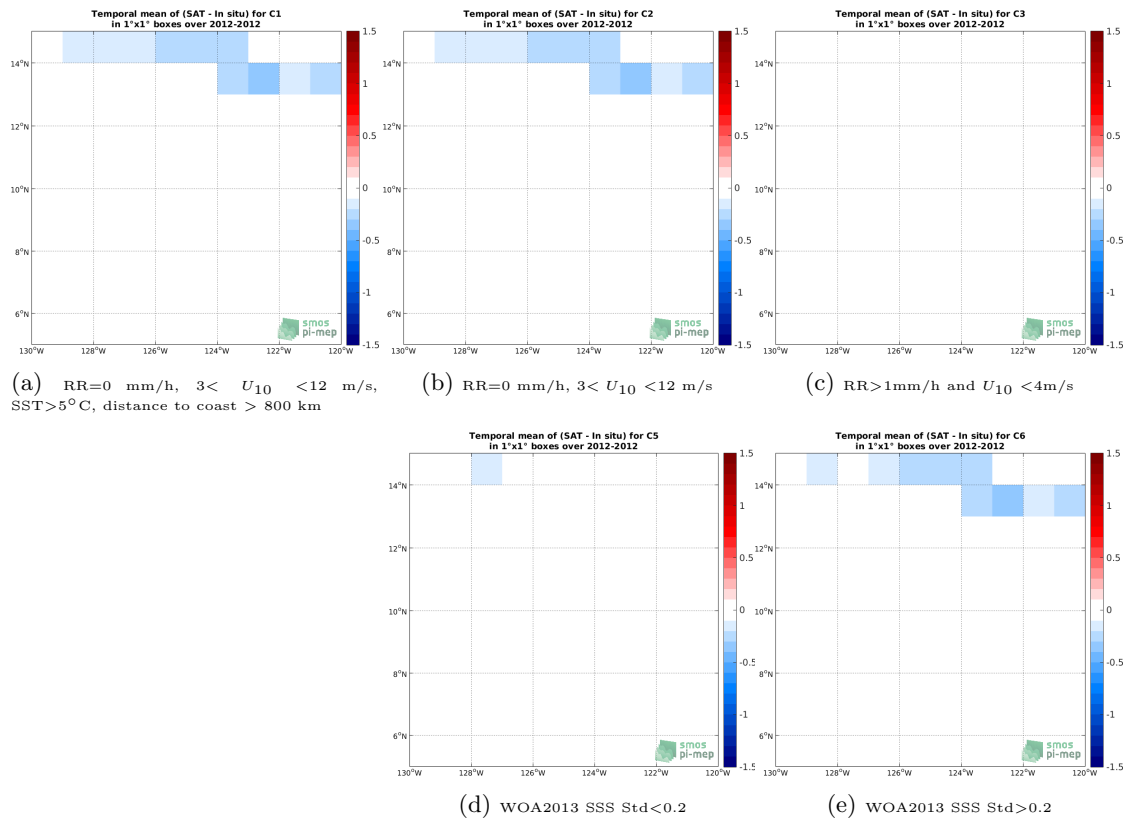
Figure 12: Temporal mean gridded over spatial boxes of size 1^\circ \times 1^\circ of \Delta SSS (CCI L4 Merged-OI v2.31 - 7-day running (ESA) - TSG (GOSUD-Research-vessel)) for 5 different subdatasets corresponding to: RR=0 mm/h, 3 < U_{10} < 12 m/s, SST>5°C, distance to coast > 800 km (a), RR=0 mm/h, 3 < U_{10} < 12 m/s (b), RR>1mm/h and U_{10} < 4 m/s (c), WOA2013 SSS Std<0.2 (d), WOA2013 SSS Std>0.2 (e).
