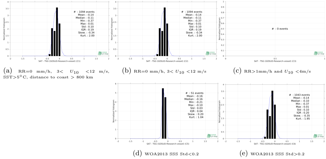
Figure 13: Normalized histogram of \Delta SSS (CCI L4 Merged-OI v2.31 - 7-day running (ESA) - TSG (GOSUD-Research-vessel)) for 5 different subdatasets corresponding to: RR=0 mm/h, 3 < U_{10} < 12 m/s, SST>5°C, distance to coast > 800 km (a), RR=0 mm/h, 3 < U_{10} < 12 m/s (b), RR>1mm/h and U_{10} < 4 m/s (c), WOA2013 SSS Std<0.2 (d), WOA2013 SSS Std>0.2 (e).
