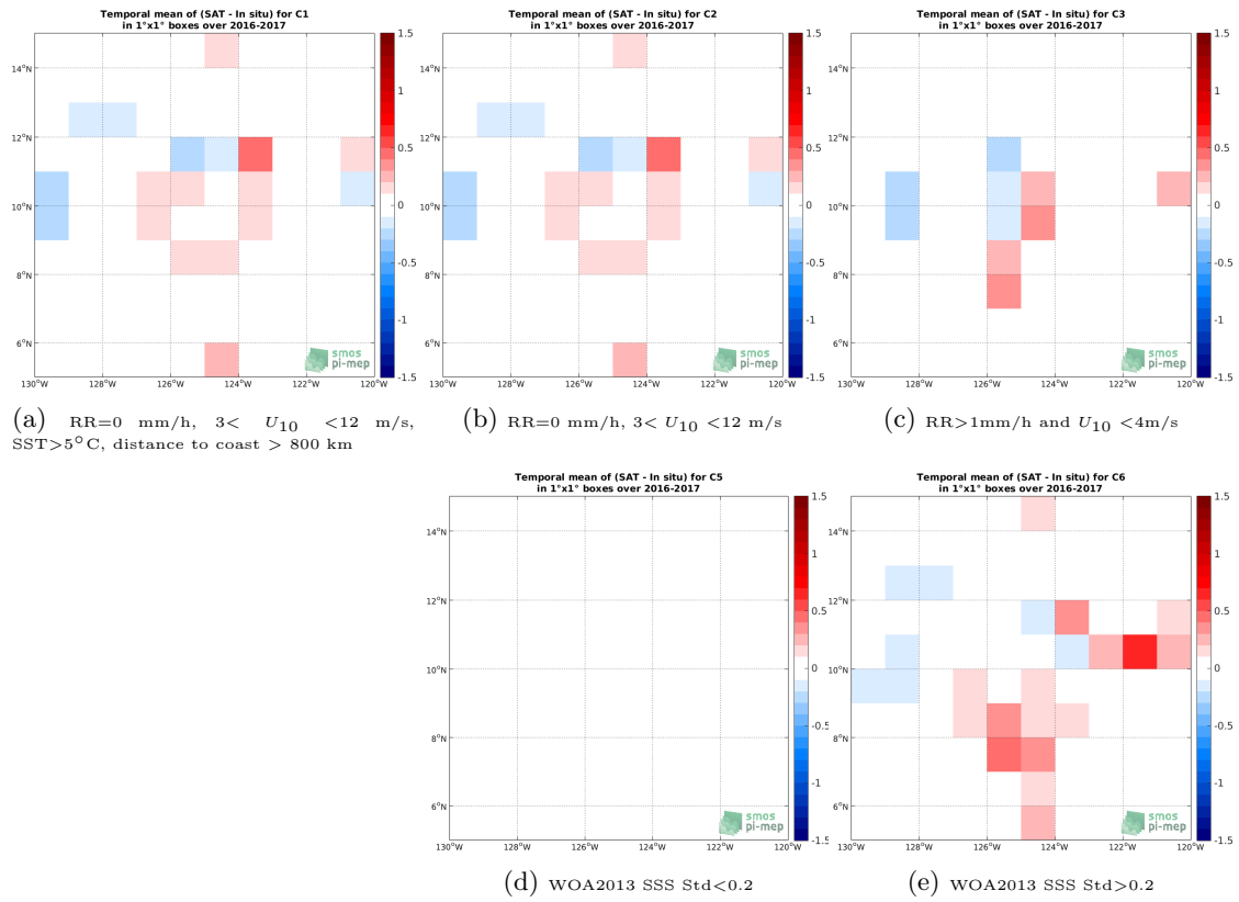
Figure 12: Temporal mean gridded over spatial boxes of size 1^\circ \times 1^\circ of \Delta SSS (CCI SSS L4 Merged-OI v2.31 - 7-day running (ESA) - Salinity Snake) for 5 different subdatasets corresponding to:RR=0 mm/h, 3 < U_{10} < 12 m/s, SST >5^\circ\text{C} , distance to coast > 800 km (a), RR=0 mm/h, 3 < U_{10} < 12 m/s (b), RR >1 mm/h and U_{10} < 4 m/s (c), WOA2013 SSS Std <0.2 (d), WOA2013 SSS Std >0.2 (e).
