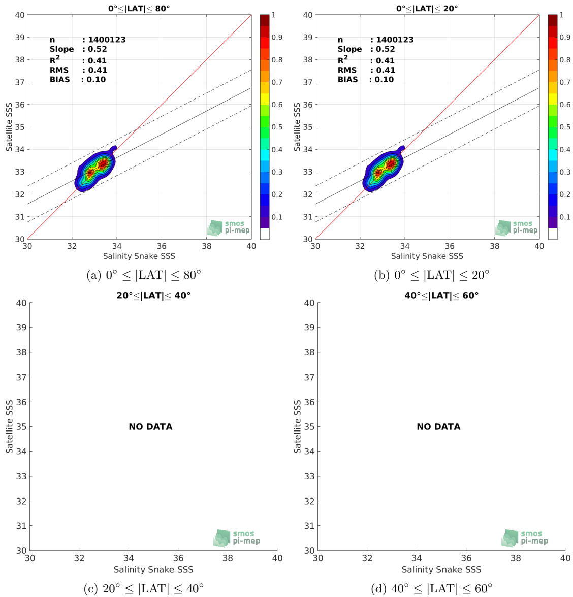
Figure 9: Contour maps of the concentration of CCI SSS L4 Merged-OI v2.31 - 7-day running (ESA) SSS (y-axis) versus Salinity Snake SSS (x-axis) at match-up pairs for different latitude bands. For each plot, the red line shows x=y . The black thin and dashed lines indicate a linear fit through the data cloud and the \pm 95\% confidence levels, respectively. The number match-up pairs n , the slope and R^2 coefficient of the linear fit, the root mean square (RMS) and the mean bias between satellite and in situ data are indicated for each latitude band in each plots.
