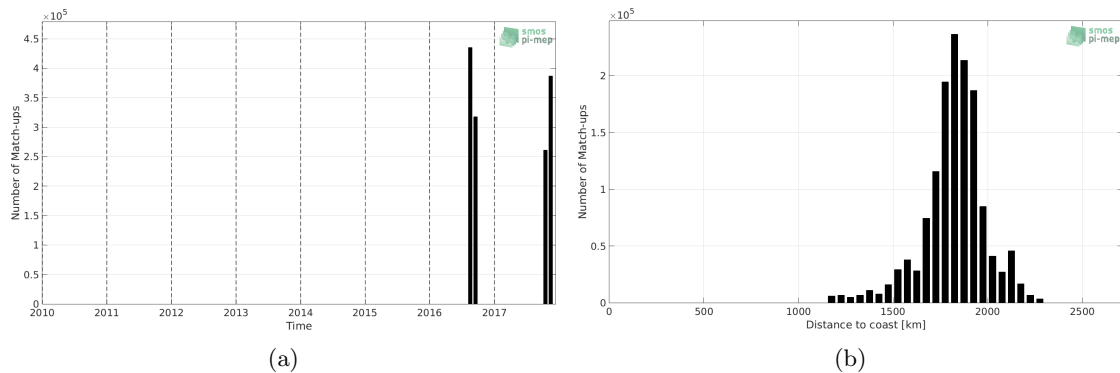
Figure 1: Number of match-ups between Salinity Snake and CCI SSS L4 Merged-OI v2.31 - 7-day running (ESA) SSS as a function of time (a) and as function of the distance to coast (b) over the SPURS 2 Pi-MEP region and for the full satellite product period.
