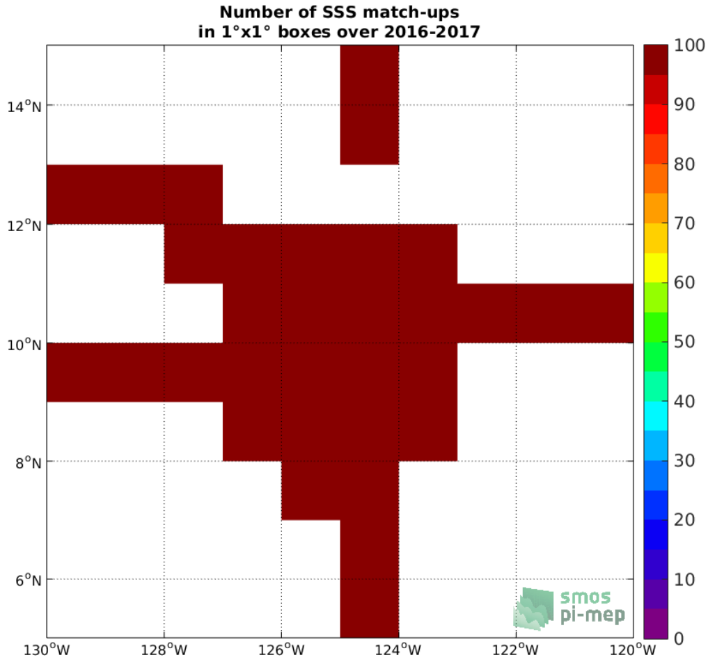
Figure 4: Number of SSS match-ups between Salinity Snake SSS and the CCI SSS L4 Merged-OI v2.31 - 7-day running (ESA) SSS product for the SPURS 2 Pi-MEP region over 1°x1° boxes and for the full satellite product period.
