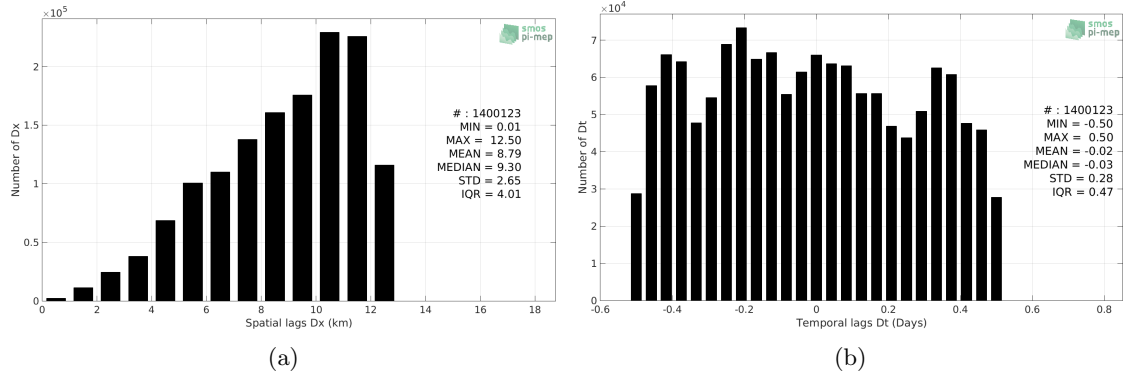
Figure 5: Histograms of the spatial (a) and temporal (b) lags between the time of the Salinity Snake measurements and the date of the corresponding CCI SSS L4 Merged-OI v2.31 - 7-day running (ESA) SSS product.
