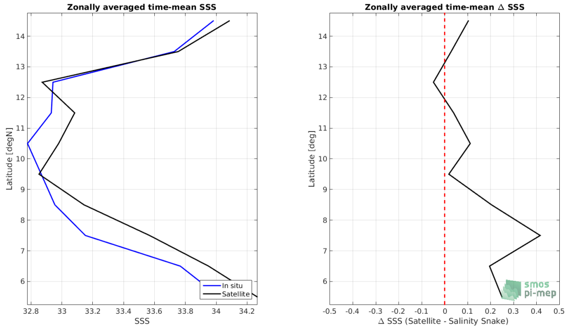
Figure 8: Left panel: Zonal mean SSS from CCI SSS L4 Merged-OI v2.31 - 7-day running (ESA) satellite product (black) and from Salinity Snake (blue). Right panel: Zonal mean of \Delta SSS (Satellite - Salinity Snake) for all the collected Pi-MEP match-up pairs estimated over the full satellite product period.
