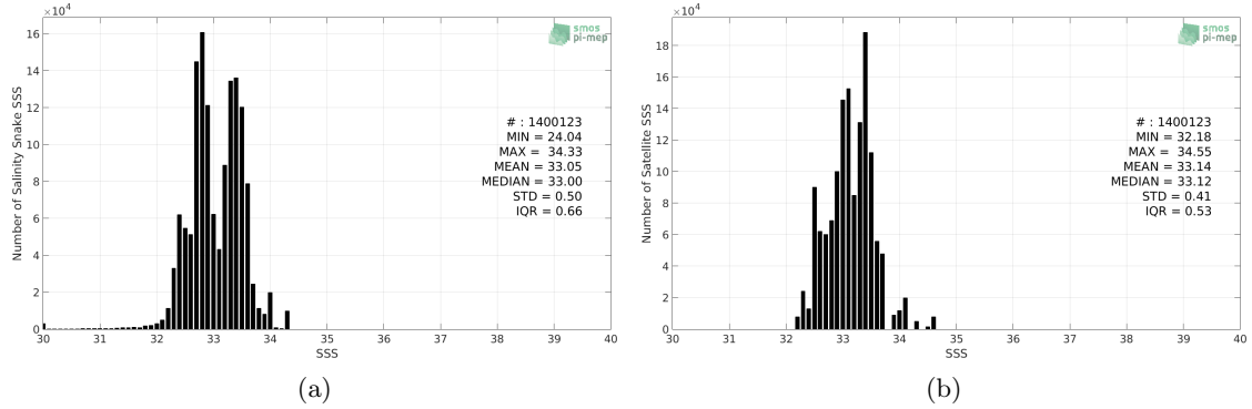
Figure 2: Histograms of SSS from Salinity Snake (a) and CCI SSS L4 Merged-OI v2.31 - 7-day running (ESA) (b) considering all match-up pairs per bins of 0.1 over the SPURS 2 Pi-MEP region and for the full satellite product period.
