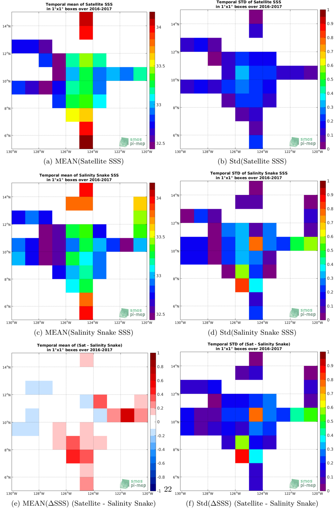
Figure 6: Temporal mean (left) and Std (right) of SSS from CCI SSS L4 Merged-OI v2.31 - 7-day running (ESA) (top), Salinity Snake (middle), and of \Delta SSS (Satellite - Salinity Snake). Only match-up pairs are used to generate these maps.
