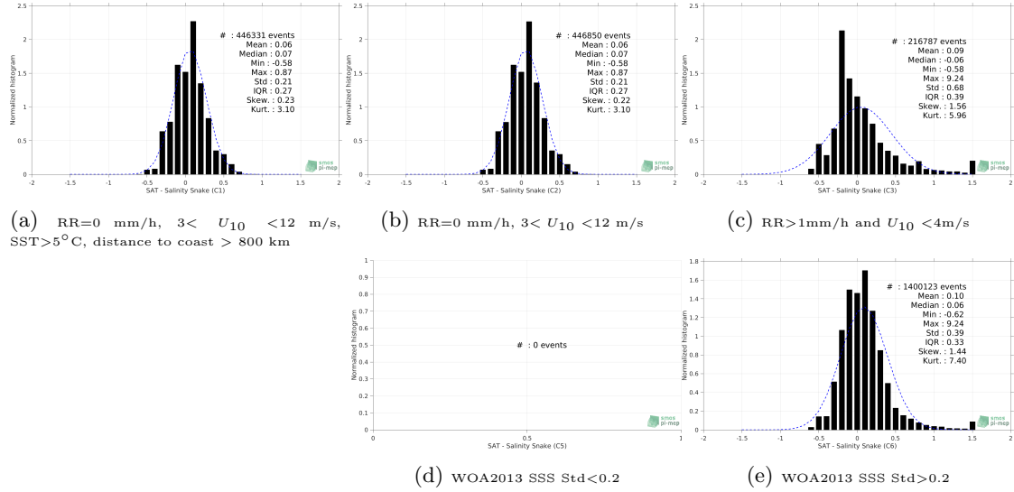
Figure 13: Normalized histogram of \Delta SSS (CCI SSS L4 Merged-OI v2.31 - 7-day running (ESA) - Salinity Snake) for 5 different subdatasets corresponding to: RR=0 mm/h, 3 < U_{10} < 12 m/s, SST>5°C, distance to coast > 800 km (a), RR=0 mm/h, 3 < U_{10} < 12 m/s (b), RR>1mm/h and U_{10} < 4 m/s (c), WOA2013 SSS Std<0.2 (d), WOA2013 SSS Std>0.2 (e).
