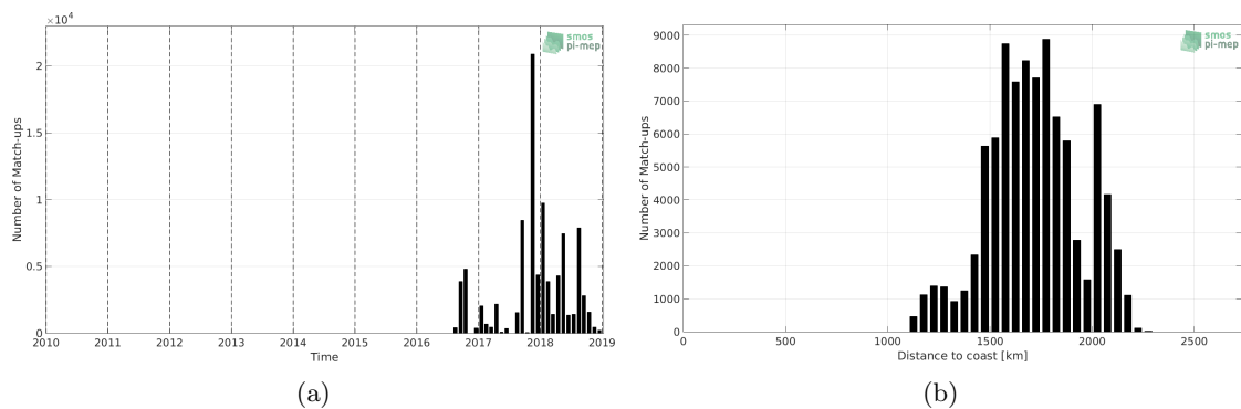
Figure 1: Number of match-ups between Surface drifters and CCI L4 Merged-OI v2.31 - 7-day running (ESA) SSS as a function of time (a) and as function of the distance to coast (b) over the SPURS 2 Pi-MEP region and for the full satellite product period.
