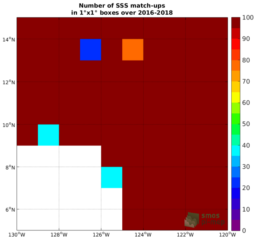
Figure 3: Number of SSS match-ups between Surface drifters SSS and the CCI L4 Merged-OI v2.31 - 7-day running (ESA) SSS product for the SPURS 2 Pi-MEP region over 1°x1° boxes and for the full satellite product period.
