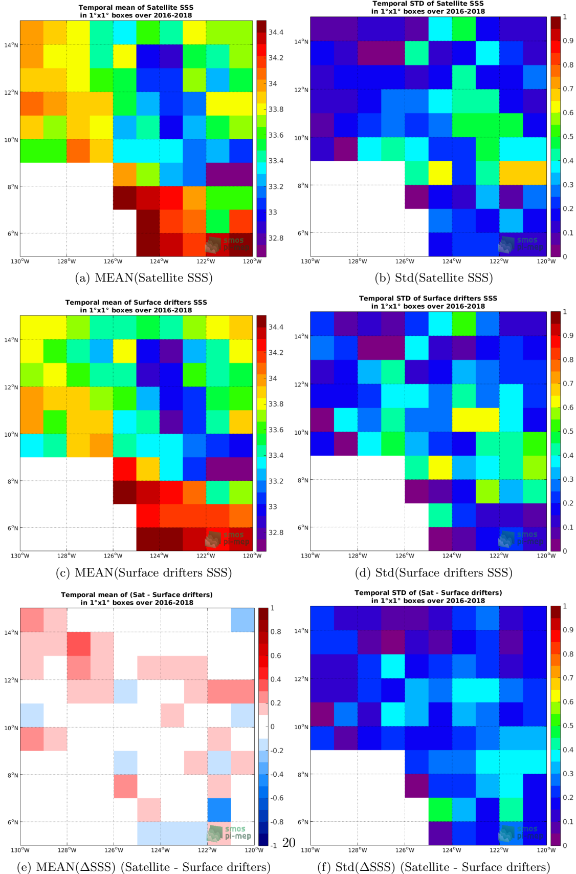
Figure 5: Temporal mean (left) and Std (right) of SSS from CCI L4 Merged-OI v2.31 - 7-day running (ESA) (top), Surface drifters (middle), and of \Delta SSS (Satellite - Surface drifters). Only match-up pairs are used to generate these maps.
