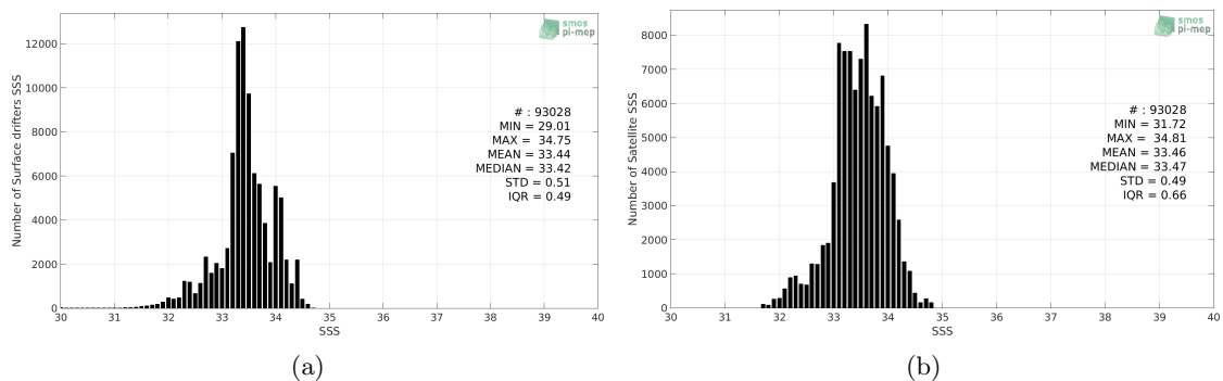
Figure 2: Histograms of SSS from Surface drifters (a) and CCI L4 Merged-OI v2.31 - 7-day running (ESA) (b) considering all match-up pairs per bins of 0.1 over the SPURS 2 Pi-MEP region and for the full satellite product period.
