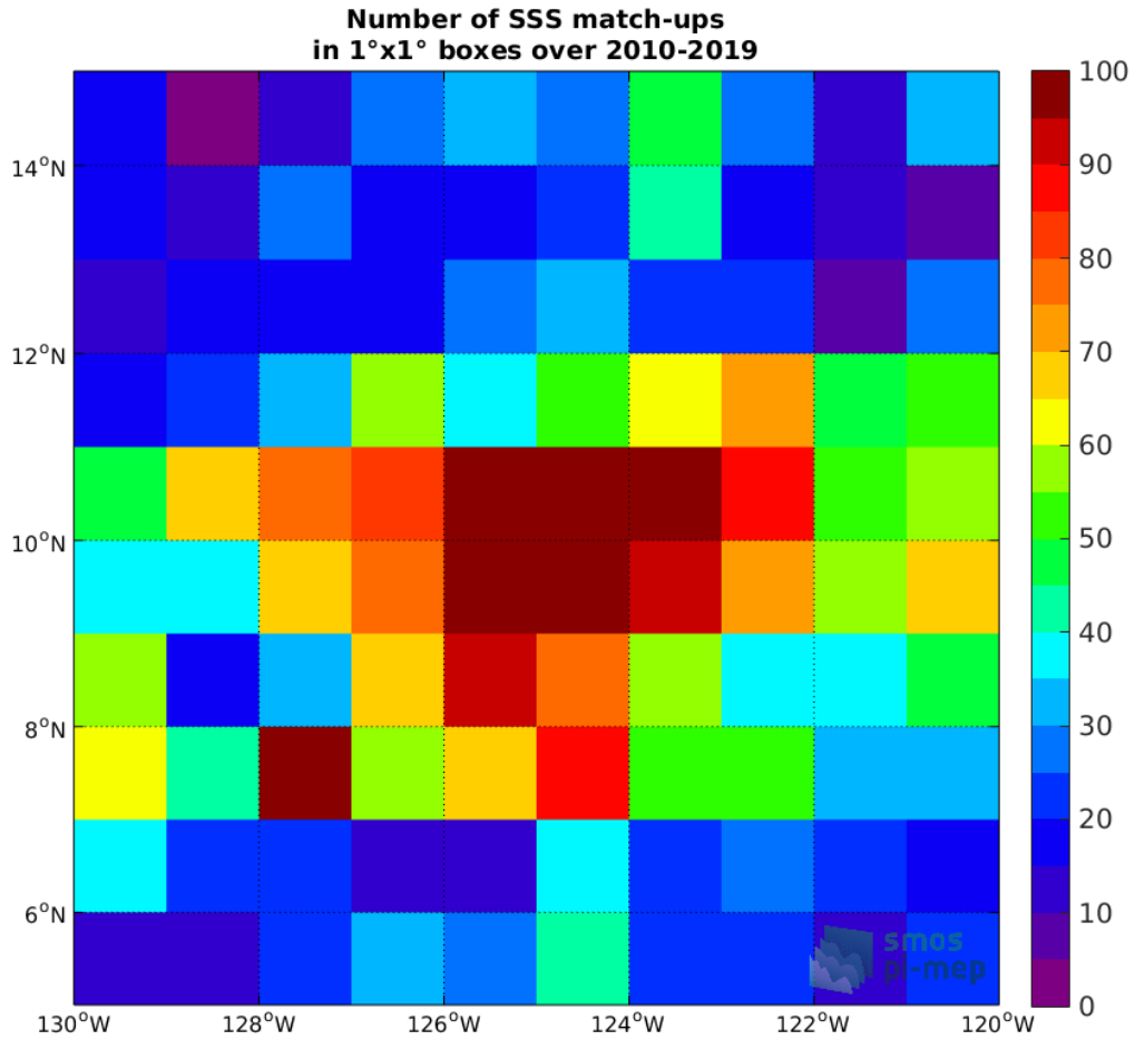
Figure 4: Number of SSS match-ups between Argo SSS and the CCI SSS L4 Merged-OI v2.31 - 7-day running (ESA) SSS product for the SPURS 2 Pi-MEP region over 1°x1° boxes and for the full satellite product period.
