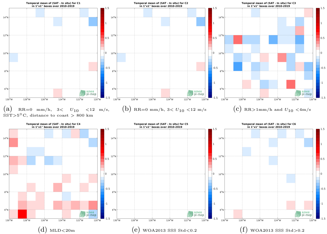
Figure 12: Temporal mean gridded over spatial boxes of size 1^\circ \times 1^\circ of \Delta SSS (CCI SSS L4 Merged-OI v2.31 - 7-day running (ESA) - Argo) for 6 different subdatasets corresponding to:RR=0 mm/h, 3 < U_{10} < 12 m/s, SST >5^\circ C, distance to coast > 800 km (a), RR=0 mm/h, 3 < U_{10} < 12 m/s (b), RR >1 mm/h and U_{10} < 4 m/s (c),MLD <20 m (d),WOA2013 SSS Std <0.2 (e),WOA2013 SSS Std >0.2 (f).
