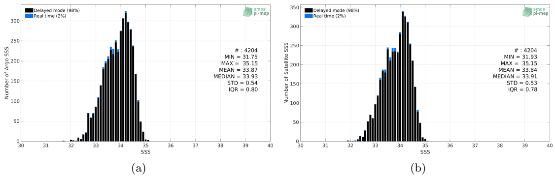
Figure 2: Histograms of SSS from Argo (a) and CCI L4 Merged-OI v2.31 - 7-day running (ESA) (b) considering all match-up pairs per bins of 0.1 over the SPURS 2 Pi-MEP region and for the full satellite product period.
