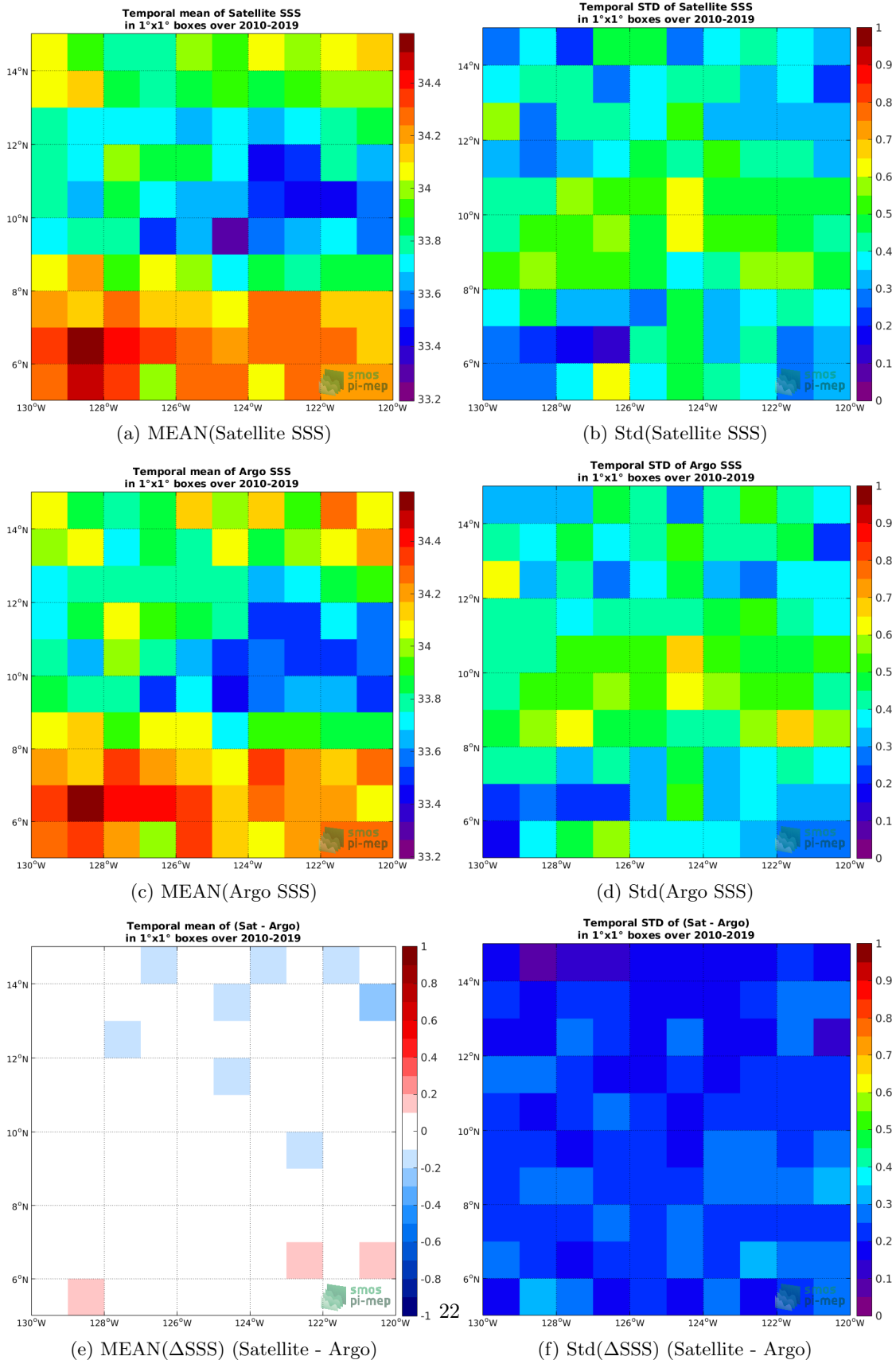
Figure 6: Temporal mean (left) and Std (right) of SSS from CCI L4 Merged-OI v2.31 - 7-day running (ESA) (top), Argo (middle), and of \Delta SSS (Satellite - Argo). Only match-up pairs are used to generate these maps.
