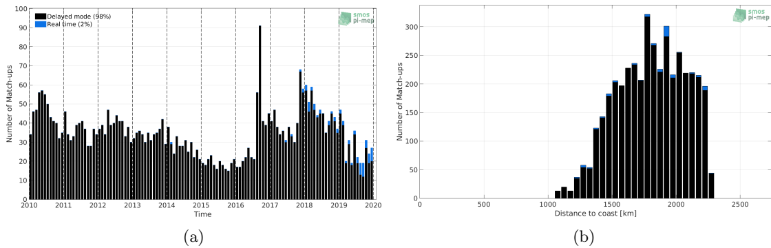
Figure 1: Number of match-ups between Argo and CCI L4 Merged-OI v2.31 - 7-day running (ESA) SSS as a function of time (a) and as function of the distance to coast (b) over the SPURS 2 Pi-MEP region and for the full satellite product period.
