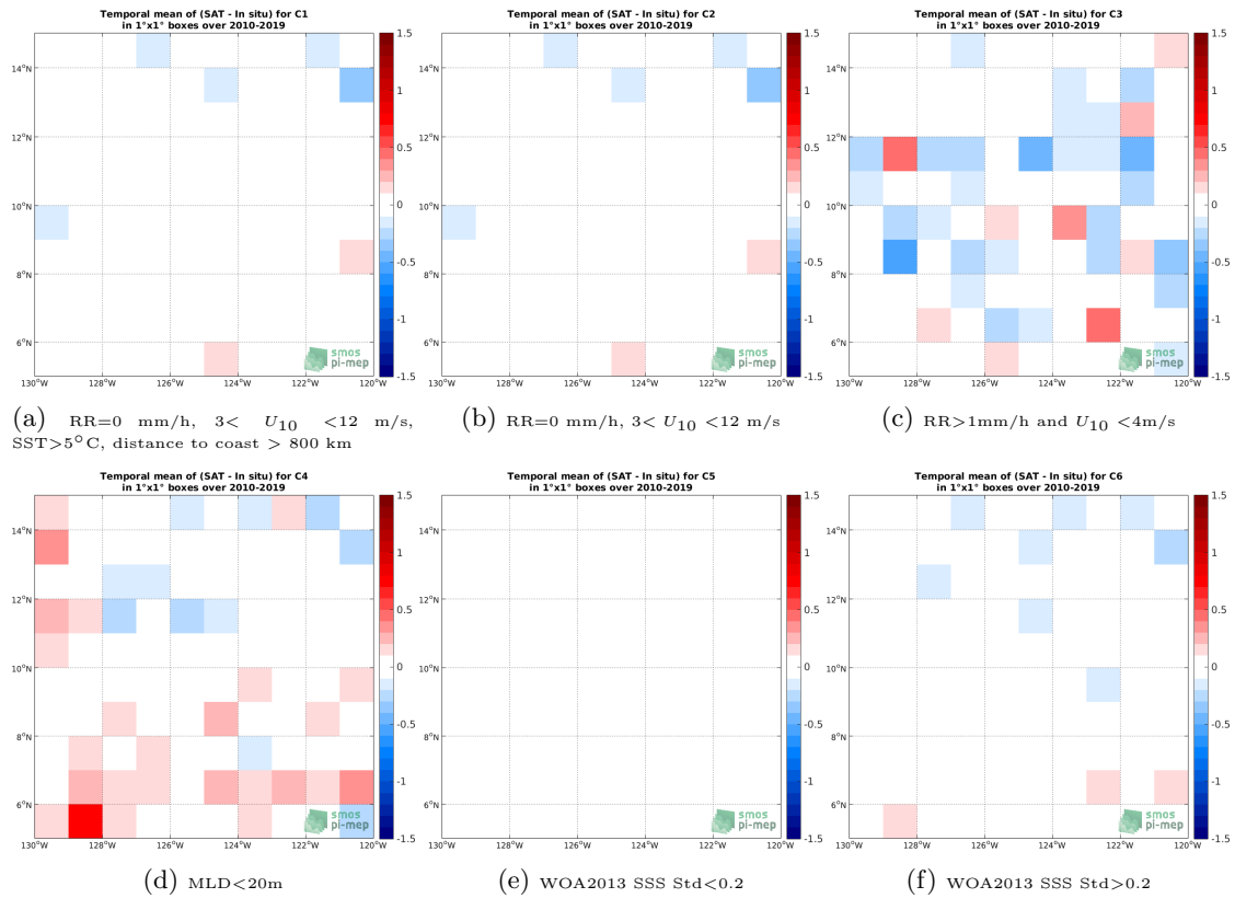
Figure 12: Temporal mean gridded over spatial boxes of size 1^\circ \times 1^\circ of \Delta SSS (CCI L4 Merged-OI v2.31 - 7-day running (ESA) - Argo) for 6 different subdatasets corresponding to:RR=0 mm/h, 3 < U_{10} < 12 m/s, SST >5^\circ C, distance to coast > 800 km (a), RR=0 mm/h, 3 < U_{10} < 12 m/s (b), RR >1 mm/h and U_{10} < 4 m/s (c),MLD <20 m (d),WOA2013 SSS Std <0.2 (e),WOA2013 SSS Std >0.2 (f).
