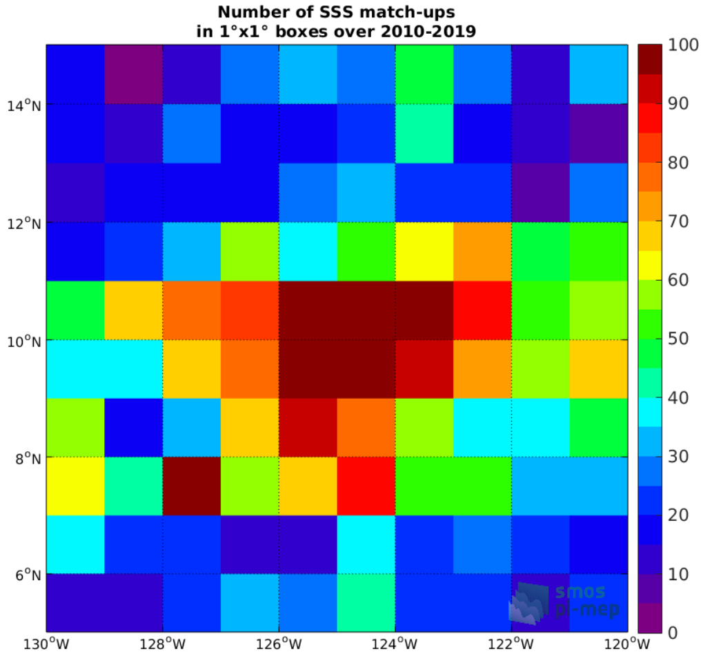
Figure 4: Number of SSS match-ups between Argo SSS and the CCI L4 Merged-OI v2.31 - 7-day running (ESA) SSS product for the SPURS 2 Pi-MEP region over 1°x1° boxes and for the full satellite product period.
