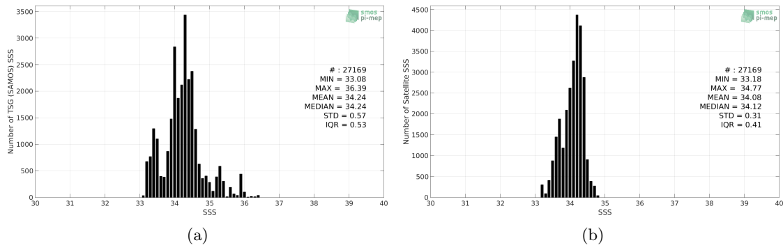
Figure 2: Histograms of SSS from TSG (SAMOS) (a) and CCI SSS L4 Merged-OI v2.31 - 30-day running (ESA) (b) considering all match-up pairs per bins of 0.1 over the SPURS 2 Pi-MEP region and for the full satellite product period.
