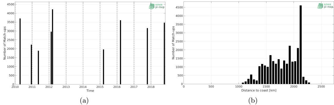
Figure 1: Number of match-ups between TSG (SAMOS) and CCI SSS L4 Merged-OI v2.31 - 30-day running (ESA) SSS as a function of time (a) and as function of the distance to coast (b) over the SPURS 2 Pi-MEP region and for the full satellite product period.
