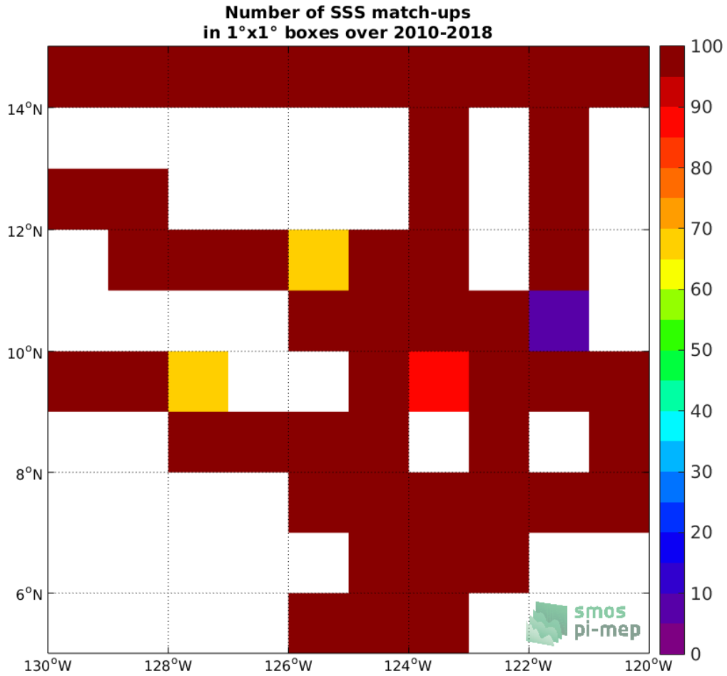
Figure 4: Number of SSS match-ups between TSG (SAMOS) SSS and the CCI SSS L4 Merged-OI v2.31 - 30-day running (ESA) SSS product for the SPURS 2 Pi-MEP region over 1°x1° boxes and for the full satellite product period.
