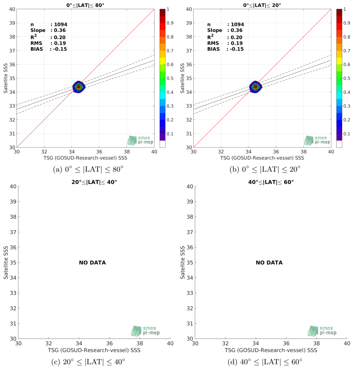
Figure 9: Contour maps of the concentration of CCI SSS L4 Merged-OI v2.31 - 30-day running (ESA) SSS ( y -axis) versus TSG (GOSUD-Research-vessel) SSS ( x -axis) at match-up pairs for different latitude bands. For each plot, the red line shows x=y . The black thin and dashed lines indicate a linear fit through the data cloud and the \pm 95\% confidence levels, respectively. The number match-up pairs n , the slope and R^2 coefficient of the linear fit, the root mean square (RMS) and the mean bias between satellite and in situ data are indicated for each latitude band in each plots.
