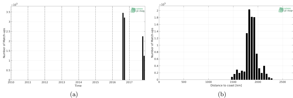
Figure 1: Number of match-ups between Salinity Snake and CCI SSS L4 Merged-OI v2.31 - 30-day running (ESA) SSS as a function of time (a) and as function of the distance to coast (b) over the SPURS 2 Pi-MEP region and for the full satellite product period.
