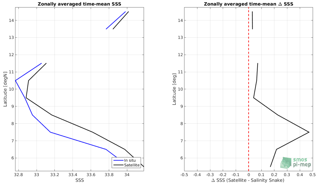
Figure 8: Left panel: Zonal mean SSS from CCI SSS L4 Merged-OI v2.31 - 30-day running (ESA) satellite product (black) and from Salinity Snake (blue). Right panel: Zonal mean of \Delta SSS (Satellite - Salinity Snake) for all the collected Pi-MEP match-up pairs estimated over the full satellite product period.
