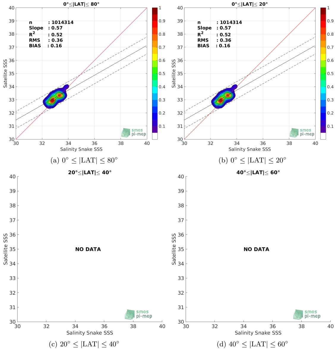
Figure 9: Contour maps of the concentration of CCI SSS L4 Merged-OI v2.31 - 30-day running (ESA) SSS (y-axis) versus Salinity Snake SSS (x-axis) at match-up pairs for different latitude bands. For each plot, the red line shows x=y . The black thin and dashed lines indicate a linear fit through the data cloud and the \pm 95\% confidence levels, respectively. The number match-up pairs n , the slope and R^2 coefficient of the linear fit, the root mean square (RMS) and the mean bias between satellite and in situ data are indicated for each latitude band in each plots.
