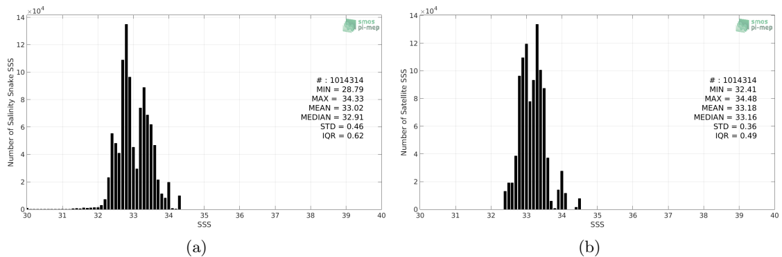
Figure 2: Histograms of SSS from Salinity Snake (a) and CCI SSS L4 Merged-OI v2.31 - 30-day running (ESA) (b) considering all match-up pairs per bins of 0.1 over the SPURS 2 Pi-MEP region and for the full satellite product period.
