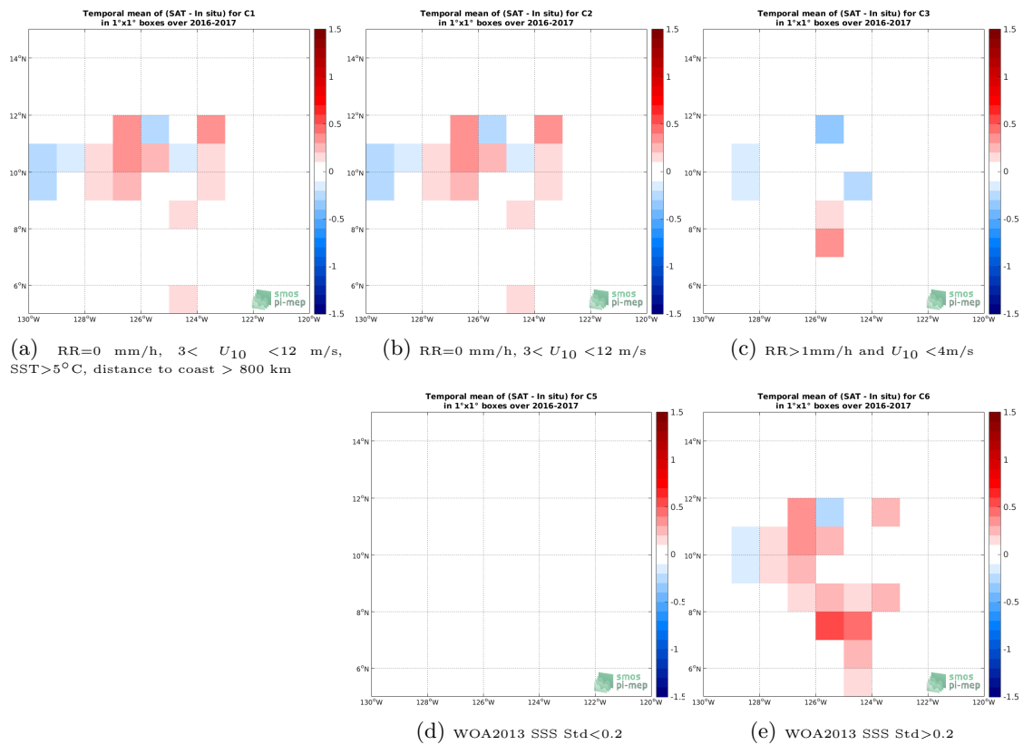
Figure 12: Temporal mean gridded over spatial boxes of size 1^\circ \times 1^\circ of \Delta SSS (CCI SSS L4 Merged-OI v2.31 - 30-day running (ESA) - Salinity Snake) for 5 different subdatasets corresponding to:RR=0 mm/h, 3 < U_{10} < 12 m/s, SST >5^\circ\text{C} , distance to coast > 800 km (a), RR=0 mm/h, 3 < U_{10} < 12 m/s (b), RR >1 mm/h and U_{10} < 4 m/s (c), WOA2013 SSS Std <0.2 (d), WOA2013 SSS Std >0.2 (e).
