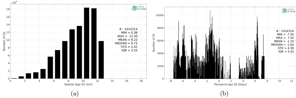
Figure 5: Histograms of the spatial (a) and temporal (b) lags between the time of the Salinity Snake measurements and the date of the corresponding CCI SSS L4 Merged-OI v2.31 - 30-day running (ESA) SSS product.
