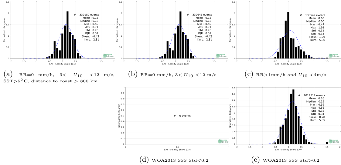
Figure 13: Normalized histogram of \Delta SSS (CCI SSS L4 Merged-OI v2.31 - 30-day running (ESA) - Salinity Snake) for 5 different subdatasets corresponding to: RR=0 mm/h, 3 < U_{10} < 12 m/s, SST > 5°C, distance to coast > 800 km (a), RR=0 mm/h, 3 < U_{10} < 12 m/s (b), RR > 1mm/h and U_{10} < 4 m/s (c), WOA2013 SSS Std < 0.2 (d), WOA2013 SSS Std > 0.2 (e).
