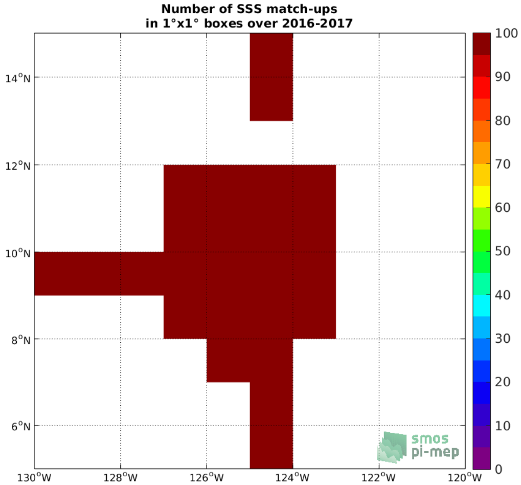
Figure 4: Number of SSS match-ups between Salinity Snake SSS and the CCI SSS L4 Merged-OI v2.31 - 30-day running (ESA) SSS product for the SPURS 2 Pi-MEP region over 1°x1° boxes and for the full satellite product period.
