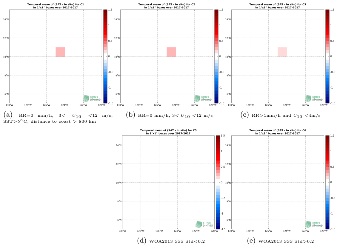
Figure 12: Temporal mean gridded over spatial boxes of size 1^\circ \times 1^\circ of \Delta\text{SSS} (CCI SSS L4 Merged-OI v2.31 - 30-day running (ESA) - Saildrone) for 5 different subdatasets corresponding to:RR=0 mm/h, 3 < U_{10} < 12 m/s, SST >5^\circ\text{C} , distance to coast > 800 km (a), RR=0 mm/h, 3 < U_{10} < 12 m/s (b), RR >1 mm/h and U_{10} < 4 m/s (c), WOA2013 SSS Std <0.2 (d), WOA2013 SSS Std >0.2 (e).
