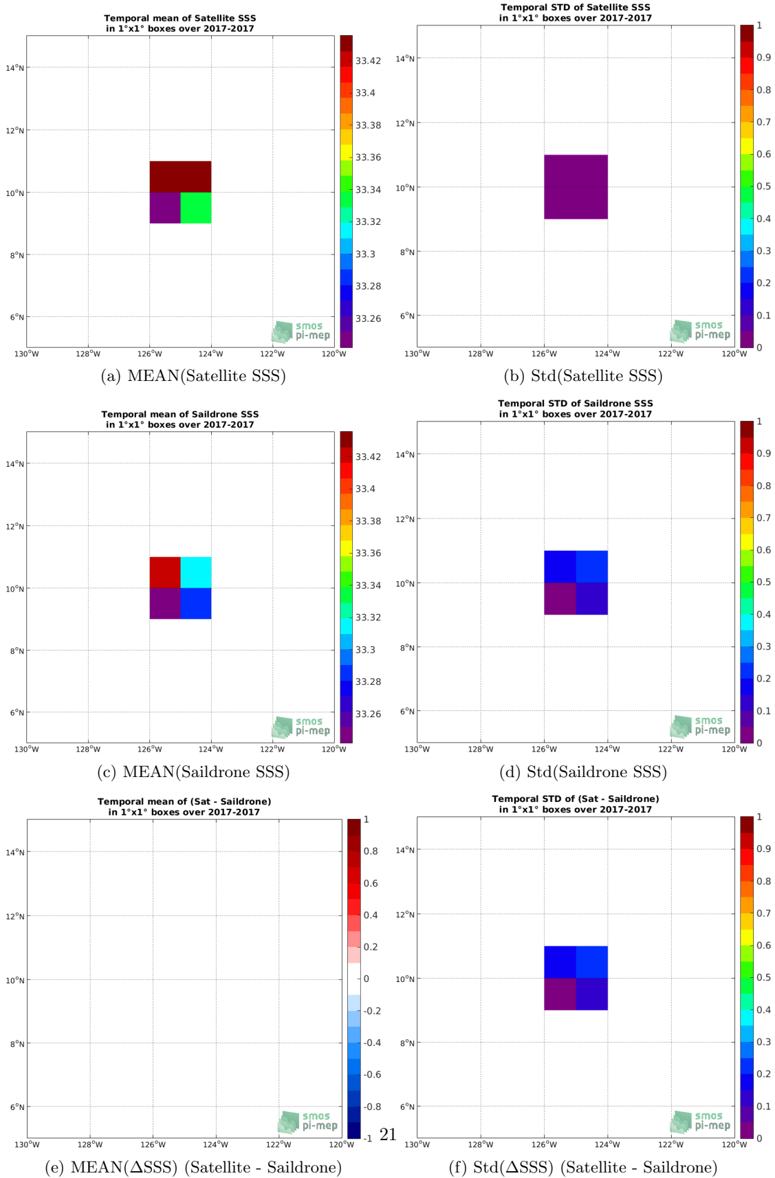
Figure 6: Temporal mean (left) and Std (right) of SSS from CCI SSS L4 Merged-OI v2.31 - 30-day running (ESA) (top), Saildrone (middle), and of \Delta SSS (Satellite - Saildrone). Only match-up pairs are used to generate these maps.
