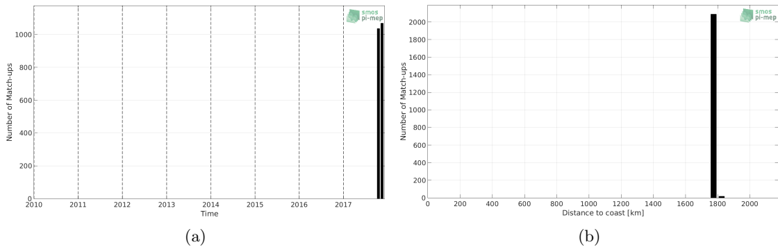
Figure 1: Number of match-ups between Saldrone and CCI SSS L4 Merged-OI v2.31 - 30-day running (ESA) SSS as a function of time (a) and as function of the distance to coast (b) over the SPURS 2 Pi-MEP region and for the full satellite product period.
