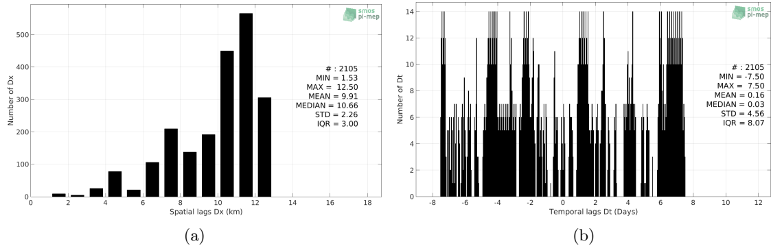
Figure 5: Histograms of the spatial (a) and temporal (b) lags between the time of the Saildrone measurements and the date of the corresponding CCI SSS L4 Merged-OI v2.31 - 30-day running (ESA) SSS product.
