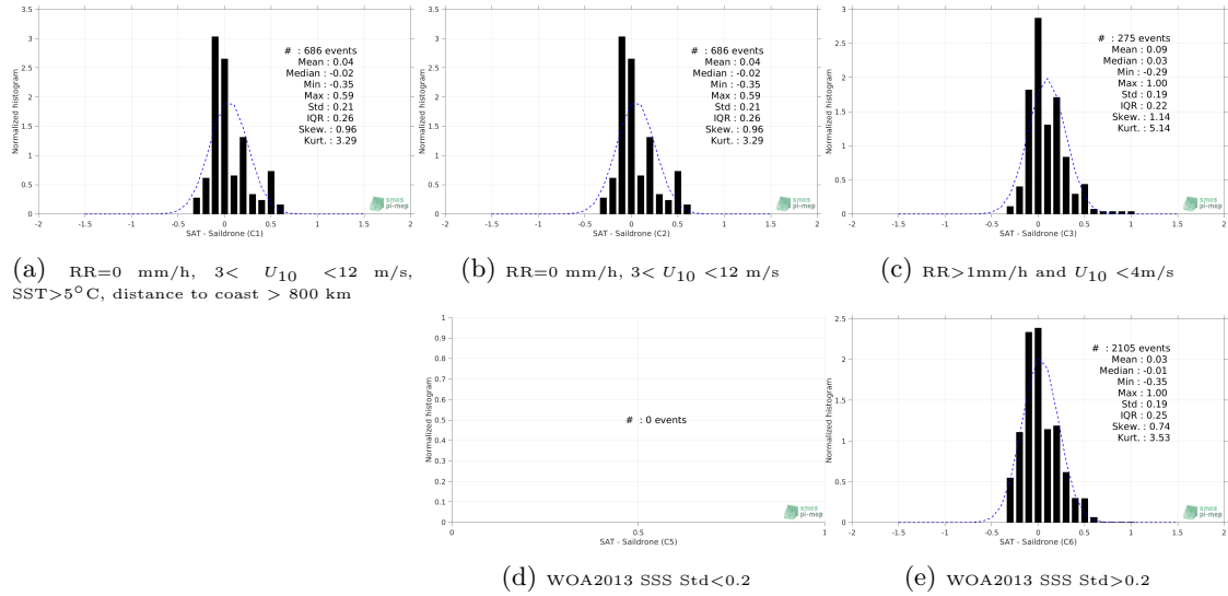
Figure 13: Normalized histogram of \Delta SSS (CCI SSS L4 Merged-OI v2.31 - 30-day running (ESA) - Saildrone) for 5 different subdatasets corresponding to: RR=0 mm/h, 3 < U_{10} < 12 m/s, SST>5°C, distance to coast > 800 km (a), RR=0 mm/h, 3 < U_{10} < 12 m/s (b), RR>1mm/h and U_{10} < 4 m/s (c), WOA2013 SSS Std<0.2 (d), WOA2013 SSS Std>0.2 (e).
