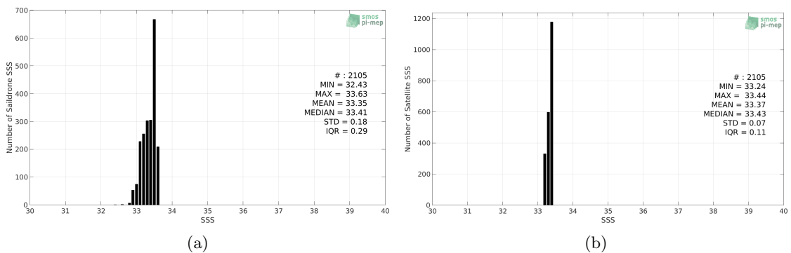
Figure 2: Histograms of SSS from Saldrone (a) and CCI SSS L4 Merged-OI v2.31 - 30-day running (ESA) (b) considering all match-up pairs per bins of 0.1 over the SPURS 2 Pi-MEP region and for the full satellite product period.
