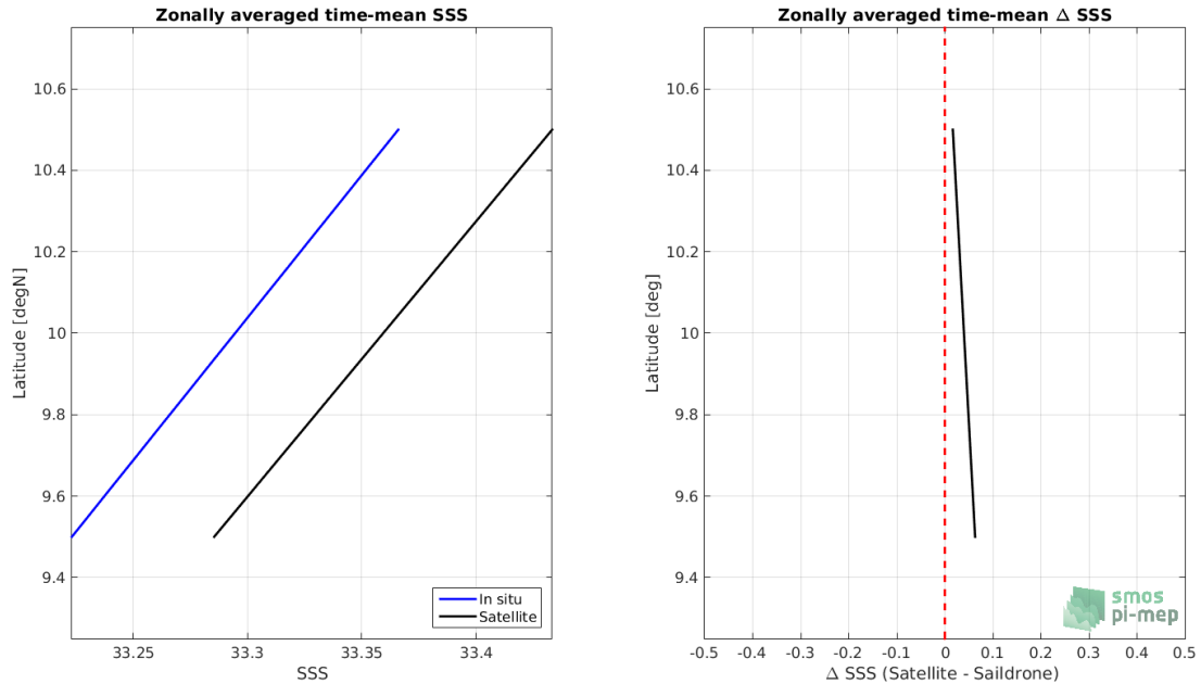
Figure 8: Left panel: Zonal mean SSS from CCI SSS L4 Merged-OI v2.31 - 30-day running (ESA) satellite product (black) and from Sairdrone (blue). Right panel: Zonal mean of \Delta SSS (Satellite - Sairdrone) for all the collected Pi-MEP match-up pairs estimated over the full satellite product period.
