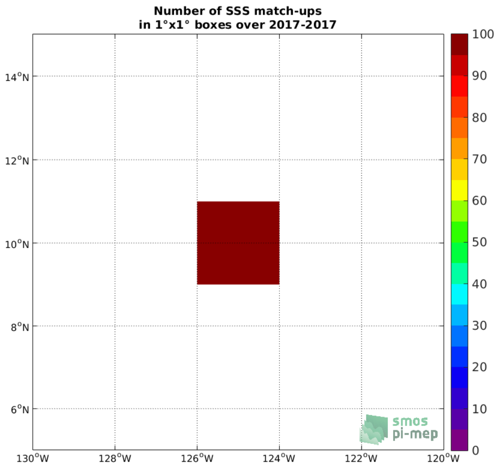
Figure 4: Number of SSS match-ups between Saildrone SSS and the CCI SSS L4 Merged-OI v2.31 - 30-day running (ESA) SSS product for the SPURS 2 Pi-MEP region over 1°x1° boxes and for the full satellite product period.
