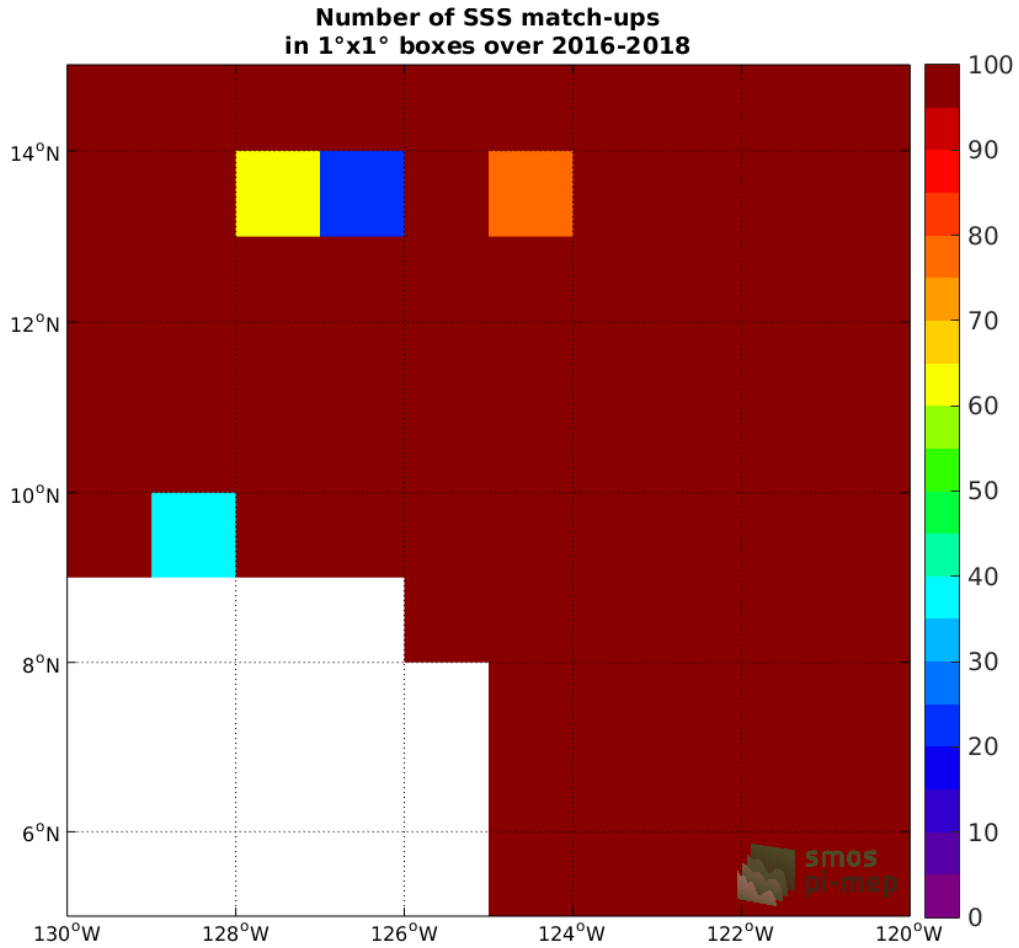
Figure 3: Number of SSS match-ups between Surface drifters SSS and the CCI SSS L4 Merged-OI v2.31 - 30-day running (ESA) SSS product for the SPURS 2 Pi-MEP region over 1°x1° boxes and for the full satellite product period.
