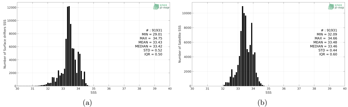
Figure 2: Histograms of SSS from Surface drifters (a) and CCI SSS L4 Merged-OI v2.31 - 30-day running (ESA) (b) considering all match-up pairs per bins of 0.1 over the SPURS 2 Pi-MEP region and for the full satellite product period.
