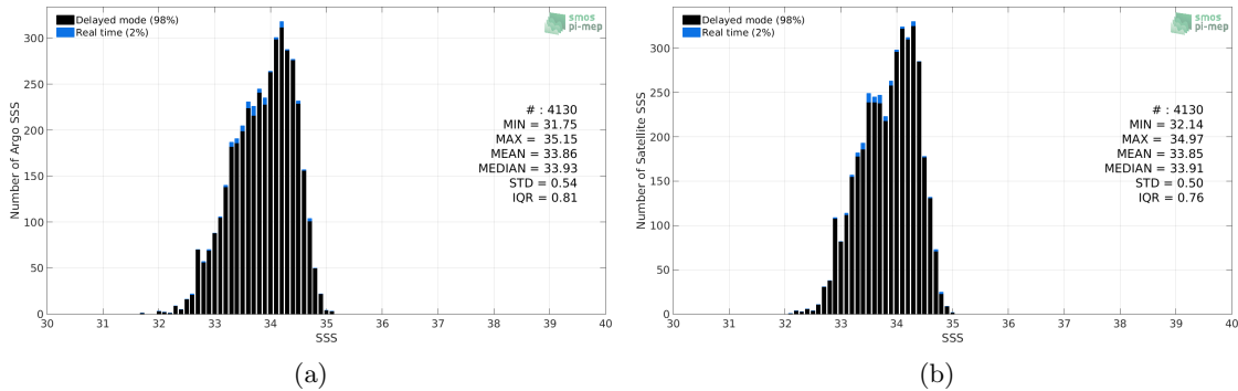
Figure 2: Histograms of SSS from Argo (a) and CCI SSS L4 Merged-OI v2.31 - 30-day running (ESA) (b) considering all match-up pairs per bins of 0.1 over the SPURS 2 Pi-MEP region and for the full satellite product period.
