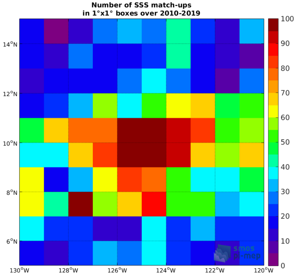
Figure 4: Number of SSS match-ups between Argo SSS and the CCI SSS L4 Merged-OI v2.31 - 30-day running (ESA) SSS product for the SPURS 2 Pi-MEP region over 1°x1° boxes and for the full satellite product period.
