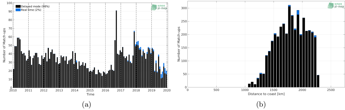
Figure 1: Number of match-ups between Argo and CCI SSS L4 Merged-OI v2.31 - 30-day running (ESA) SSS as a function of time (a) and as function of the distance to coast (b) over the SPURS 2 Pi-MEP region and for the full satellite product period.
