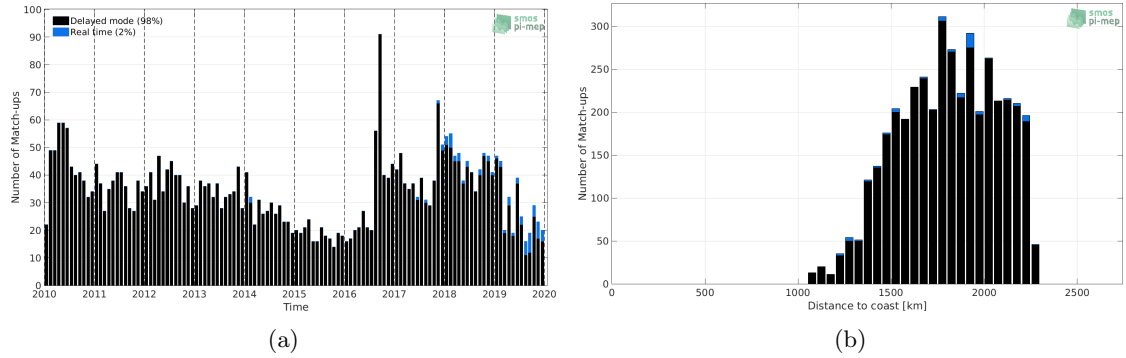
Figure 1: Number of match-ups between Argo and CCI L4 Merged-OI v2.31 - 30-day running (ESA) SSS as a function of time (a) and as function of the distance to coast (b) over the SPURS 2 Pi-MEP region and for the full satellite product period.
