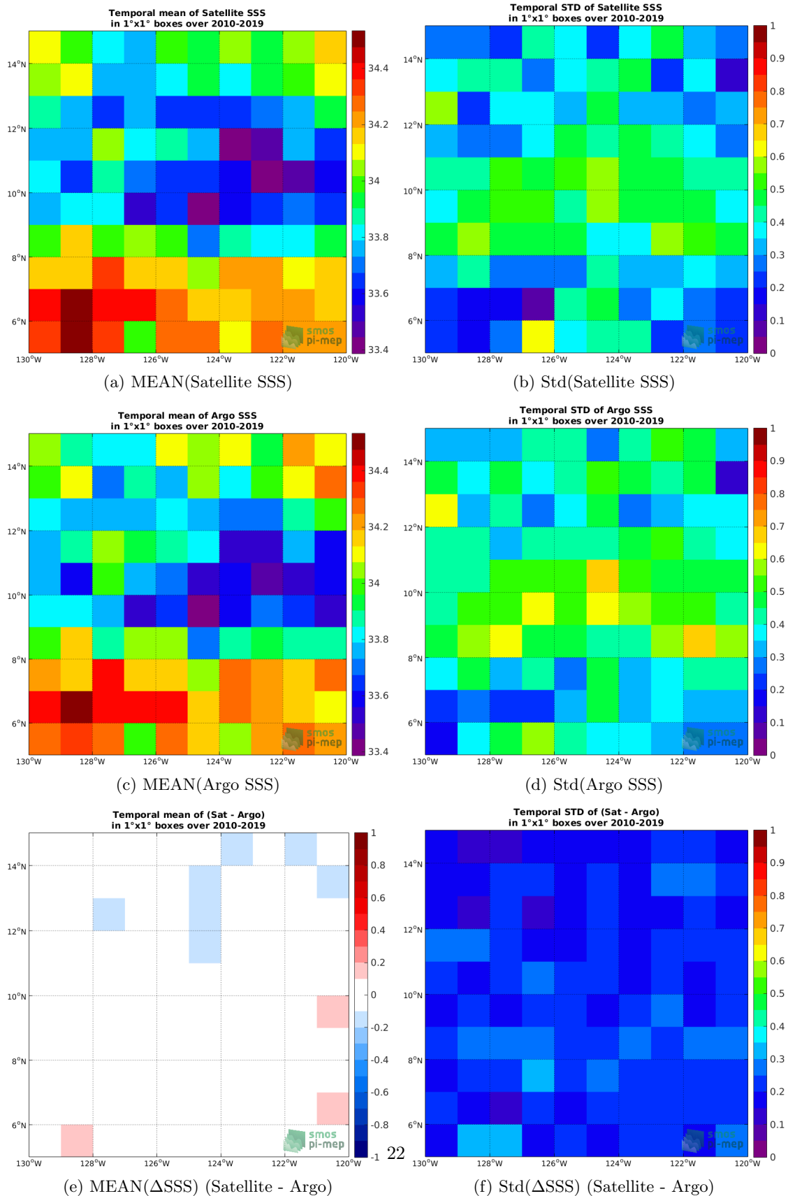
Figure 6: Temporal mean (left) and Std (right) of SSS from CCI L4 Merged-OI v2.31 - 30-day running (ESA) (top), Argo (middle), and of \Delta SSS (Satellite - Argo). Only match-up pairs are used to generate these maps.
