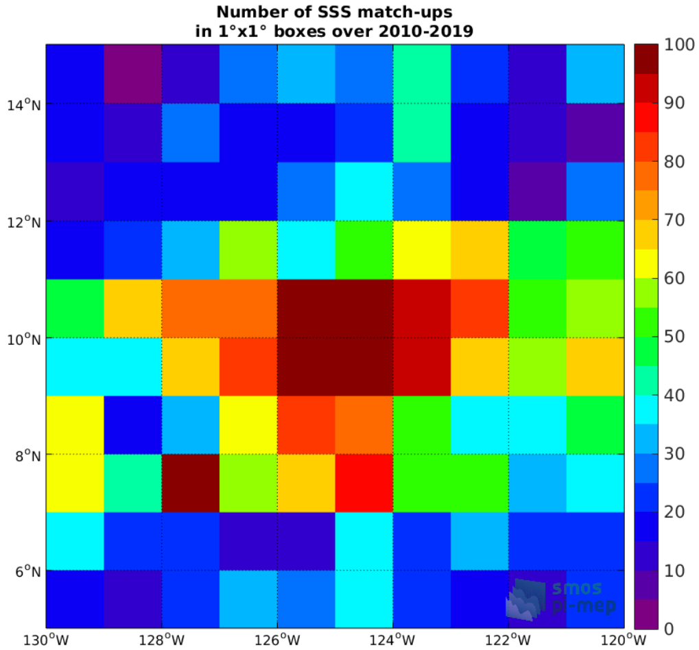
Figure 4: Number of SSS match-ups between Argo SSS and the CCI L4 Merged-OI v2.31 - 30-day running (ESA) SSS product for the SPURS 2 Pi-MEP region over 1°x1° boxes and for the full satellite product period.
