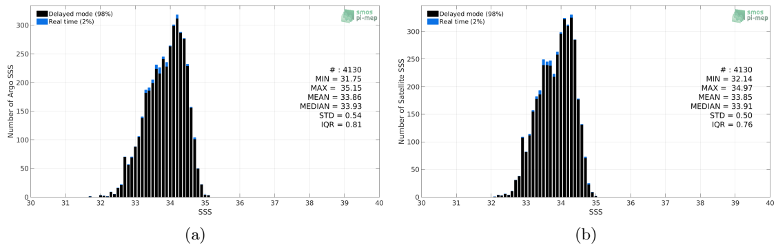
Figure 2: Histograms of SSS from Argo (a) and CCI L4 Merged-OI v2.31 - 30-day running (ESA) (b) considering all match-up pairs per bins of 0.1 over the SPURS 2 Pi-MEP region and for the full satellite product period.
