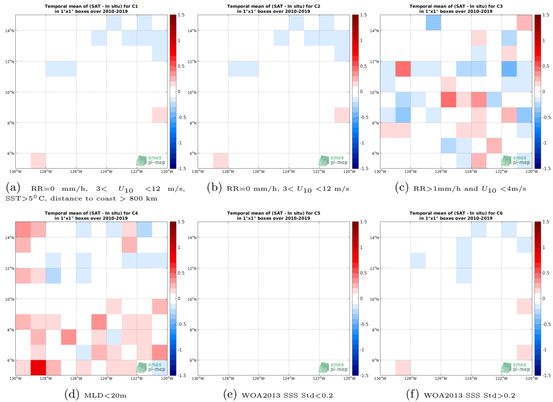
Figure 12: Temporal mean gridded over spatial boxes of size 1^\circ \times 1^\circ of \Delta SSS (CCI L4 Merged-OI v2.31 - 30-day running (ESA) - Argo) for 6 different subdatasets corresponding to:RR=0 mm/h, 3 < U_{10} < 12 m/s, SST >5^\circ C, distance to coast > 800 km (a), RR=0 mm/h, 3 < U_{10} < 12 m/s (b), RR >1 mm/h and U_{10} < 4 m/s (c),MLD <20 m (d),WOA2013 SSS Std <0.2 (e),WOA2013 SSS Std >0.2 (f).
