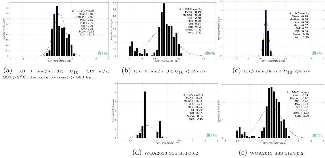
Figure 13: Normalized histogram of \Delta SSS (CCI L4 Merged-OI v1.8 - 30-day running (ESA) - TSG-SAMOS) for 5 different subdatasets corresponding to: RR=0 mm/h, 3 < U_{10} < 12 m/s, SST>5°C, distance to coast > 800 km (a), RR=0 mm/h, 3 < U_{10} < 12 m/s (b), RR>1mm/h and U_{10} < 4 m/s (c), WOA2013 SSS Std<0.2 (d), WOA2013 SSS Std>0.2 (e).
