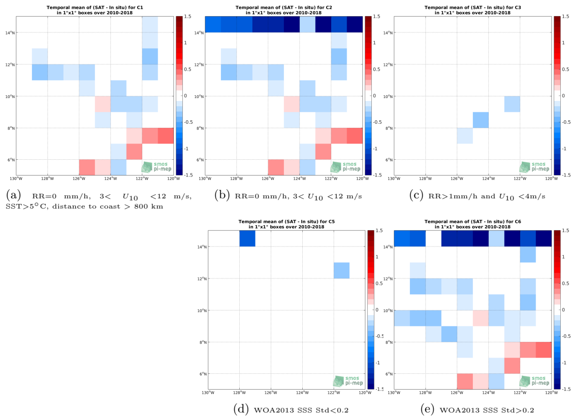
Figure 12: Temporal mean gridded over spatial boxes of size 1^\circ \times 1^\circ of \Delta SSS (CCI L4 Merged-OI v1.8 - 30-day running (ESA) - TSG-SAMOS) for 5 different subdatasets corresponding to:RR=0 mm/h, 3 < U_{10} < 12 m/s, SST > 5^\circ\text{C} , distance to coast > 800 km (a), RR=0 mm/h, 3 < U_{10} < 12 m/s (b), RR > 1 mm/h and U_{10} < 4 m/s (c), WOA2013 SSS Std < 0.2 (d), WOA2013 SSS Std > 0.2 (e).
