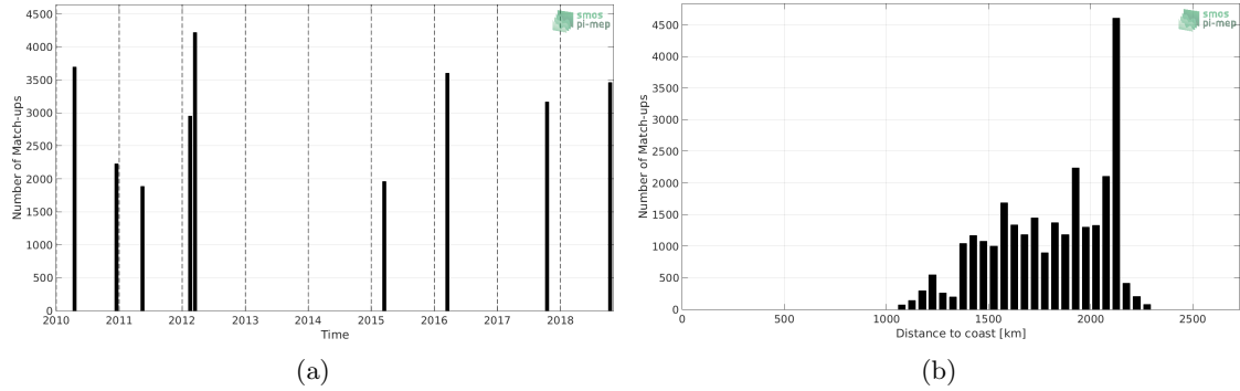
Figure 1: Number of match-ups between TSG-SAMOS and CCI L4 Merged-OI v1.8 - 30-day running (ESA) SSS as a function of time (a) and as function of the distance to coast (b) over the SPURS 2 Pi-MEP region and for the full satellite product period.
