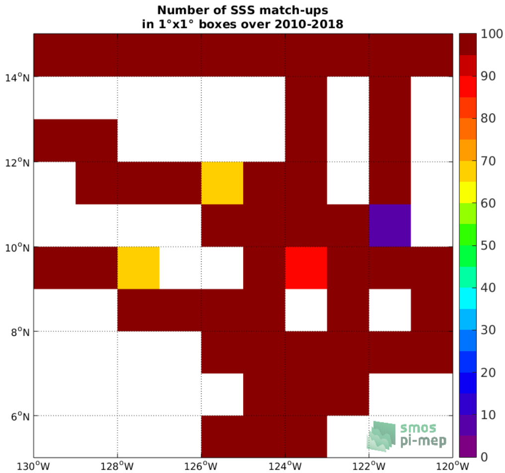
Figure 4: Number of SSS match-ups between TSG-SAMOS SSS and the CCI L4 Merged-OI v1.8 - 30-day running (ESA) SSS product for the SPURS 2 Pi-MEP region over 1°x1° boxes and for the full satellite product period.
