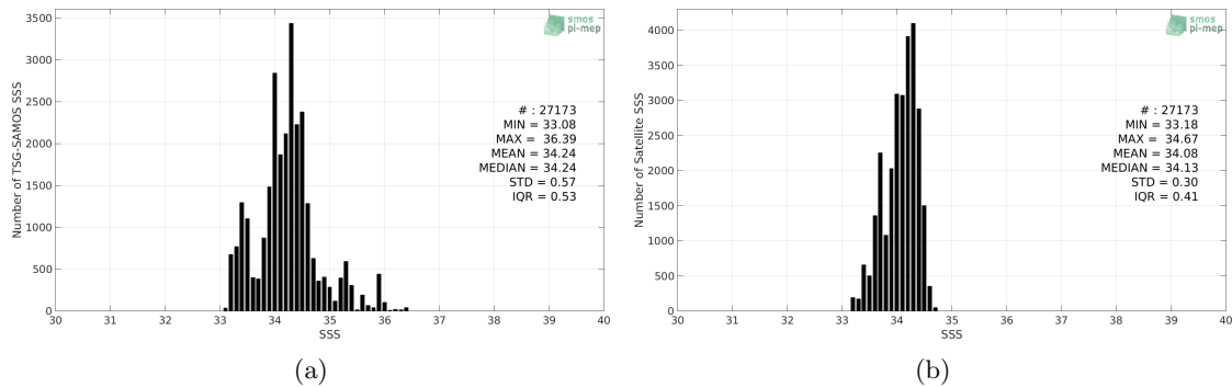
Figure 2: Histograms of SSS from TSG-SAMOS (a) and CCI-L4-ESA-MERGED-OI-V1.8-30DAY-RUNNING (b) considering all match-up pairs per bins of 0.1 over the SPURS 2 Pi-MEP region and for the full satellite product period.
