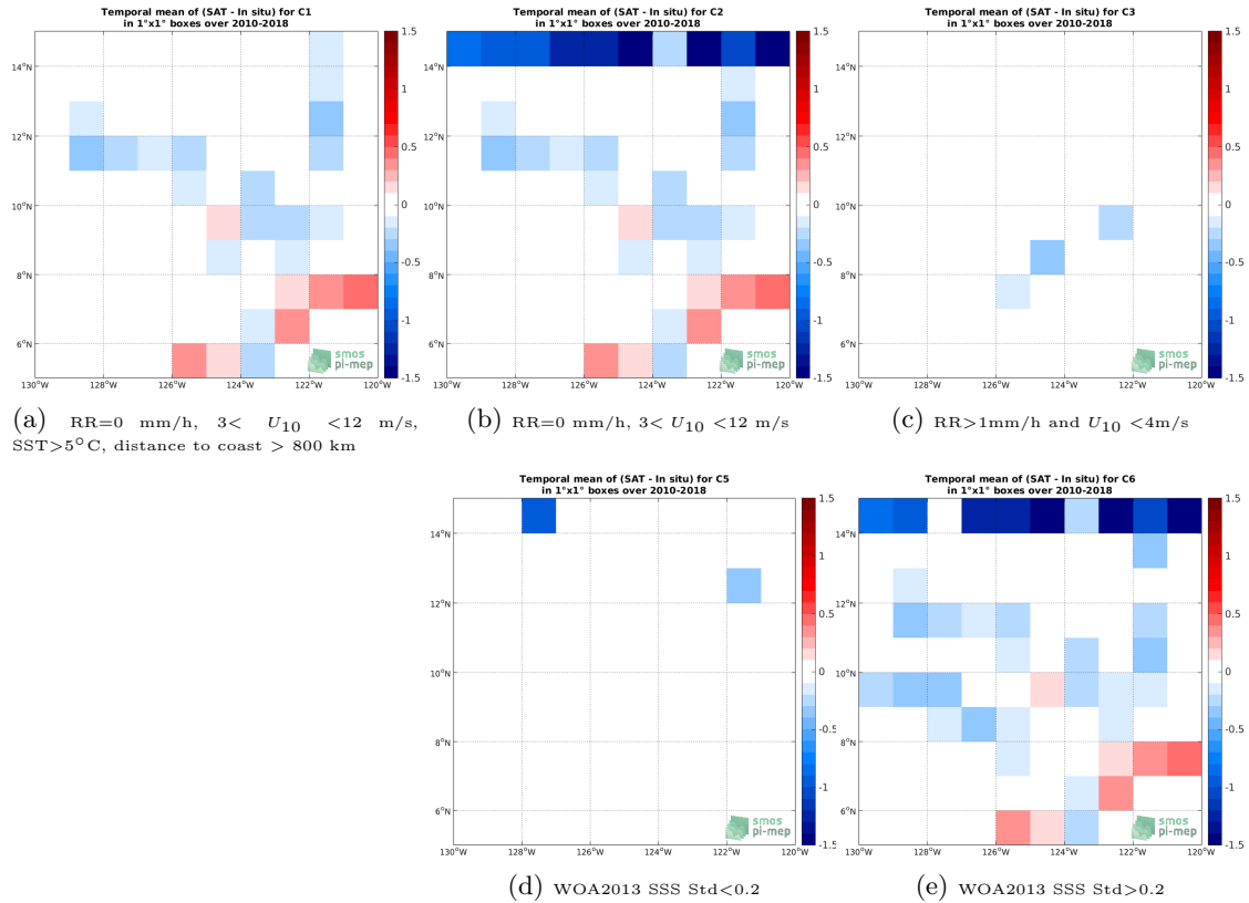
Figure 12: Temporal mean gridded over spatial boxes of size 1^\circ \times 1^\circ of \Delta SSS (CCI-L4-ESA-MERGED-OI-V1.8-30DAY-RUNNING - TSG-SAMOS) for 5 different subdatasets corresponding to:RR=0 mm/h, 3 < U_{10} < 12 m/s, SST >5^\circ\text{C} , distance to coast > 800 km (a), RR=0 mm/h, 3 < U_{10} < 12 m/s (b), RR >1 mm/h and U_{10} < 4 m/s (c), WOA2013 SSS Std <0.2 (d), WOA2013 SSS Std >0.2 (e).
