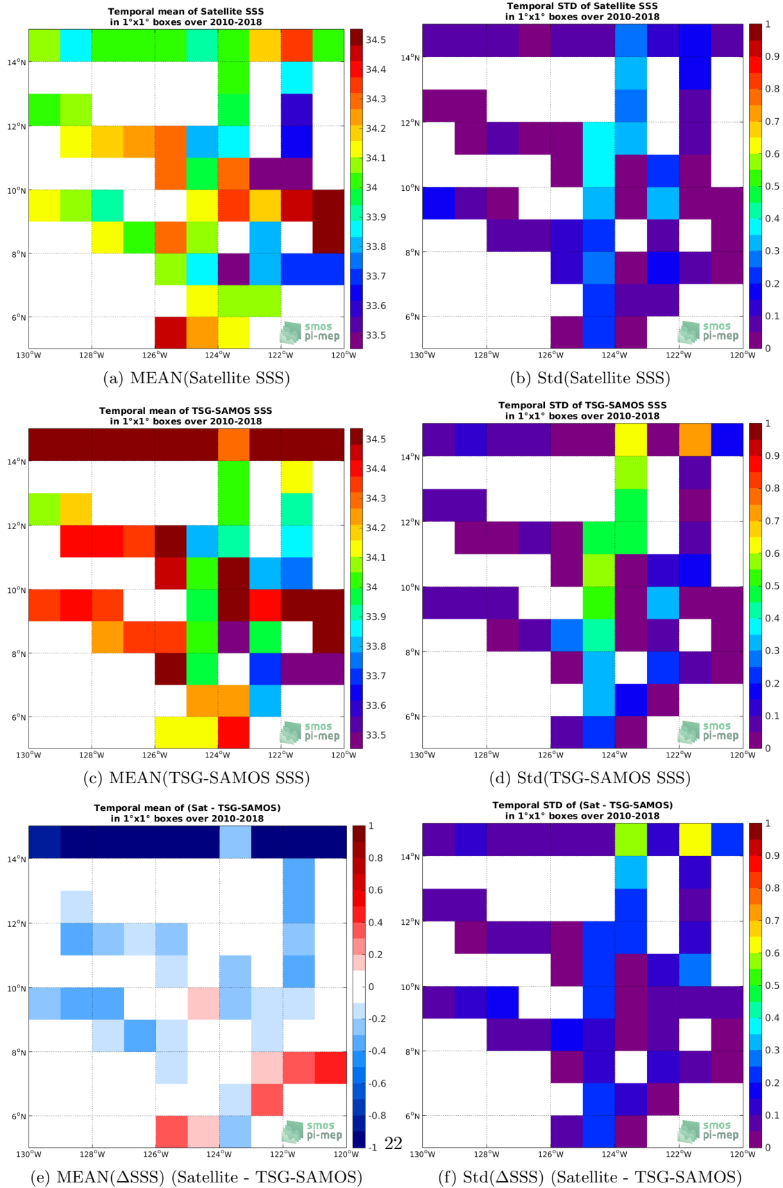
Figure 6: Temporal mean (left) and Std (right) of SSS from CCI-L4-ESA-MERGED-OI-V1.8-30DAY-RUNNING (top), TSG-SAMOS (middle), and of \Delta SSS (Satellite - TSG-SAMOS). Only match-up pairs are used to generate these maps.
