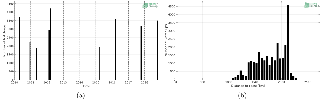
Figure 1: Number of match-ups between TSG-SAMOS and CCI-L4-ESA-MERGED-OI-V1.8-30DAY-RUNNING SSS as a function of time (a) and as function of the distance to coast (b) over the SPURS 2 Pi-MEP region and for the full satellite product period.
