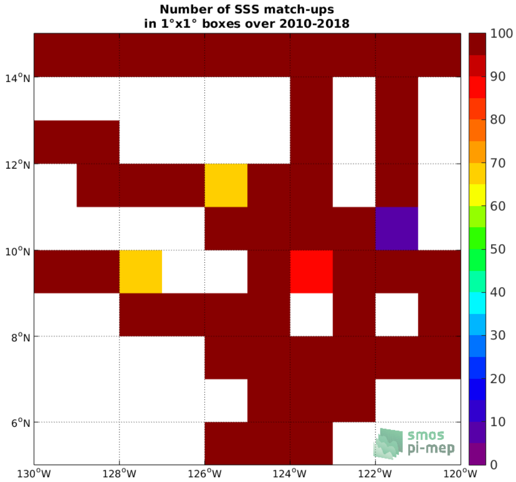
Figure 4: Number of SSS match-ups between TSG-SAMOS SSS and the CCI-L4-ESA-MERGED-OI-V1.8-30DAY-RUNNING SSS product for the SPURS 2 Pi-MEP region over 1°x1° boxes and for the full satellite product period.
