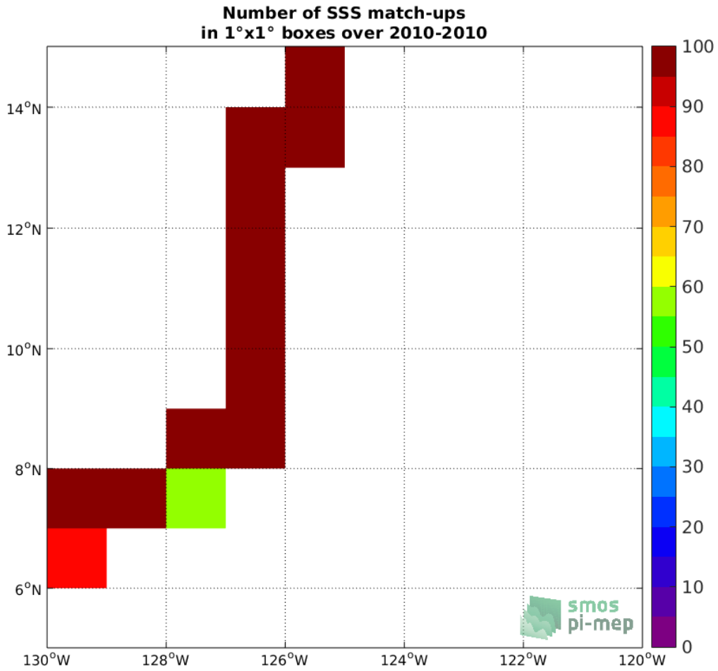
Figure 4: Number of SSS match-ups between TSG-GOSUD-Sailing-ship SSS and the CCI L4 Merged-OI v1.8 - 30-day running (ESA) SSS product for the SPURS 2 Pi-MEP region over 1°x1° boxes and for the full satellite product period.
