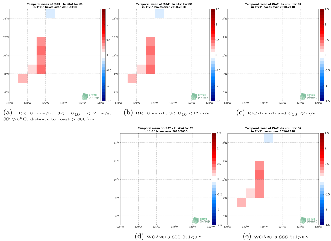
Figure 12: Temporal mean gridded over spatial boxes of size 1^\circ \times 1^\circ of \Delta SSS (CCI L4 Merged-OI v1.8 - 30-day running (ESA) - TSG-GOSUD-Sailing-ship) for 5 different subdatasets corresponding to:RR=0 mm/h, 3 < U_{10} < 12 m/s, SST>5°C, distance to coast > 800 km (a), RR=0 mm/h, 3 < U_{10} < 12 m/s (b), RR>1mm/h and U_{10} < 4 m/s (c), WOA2013 SSS Std<0.2 (d), WOA2013 SSS Std>0.2 (e).
