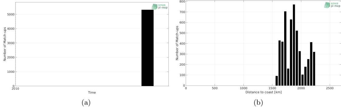
Figure 1: Number of match-ups between TSG-GOSUD-Sailing-ship and CCI L4 Merged-OI v1.8 - 30-day running (ESA) SSS as a function of time (a) and as function of the distance to coast (b) over the SPURS 2 Pi-MEP region and for the full satellite product period.
