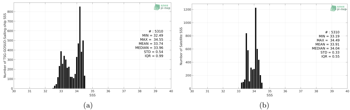
Figure 2: Histograms of SSS from TSG-GOSUD-Sailing-ship (a) and CCI L4 Merged-OI v1.8 - 30-day running (ESA) (b) considering all match-up pairs per bins of 0.1 over the SPURS 2 Pi-MEP region and for the full satellite product period.
