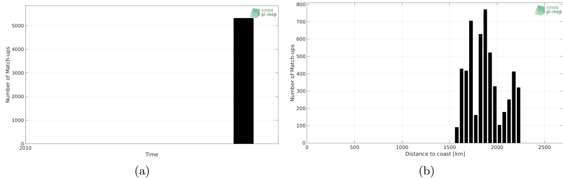
Figure 1: Number of match-ups between TSG-GOSUD-Sailing-ship and CCI-L4-ESA-MERGED-OI-V1.8-30DAY-RUNNING SSS as a function of time (a) and as function of the distance to coast (b) over the SPURS 2 Pi-MEP region and for the full satellite product period.
