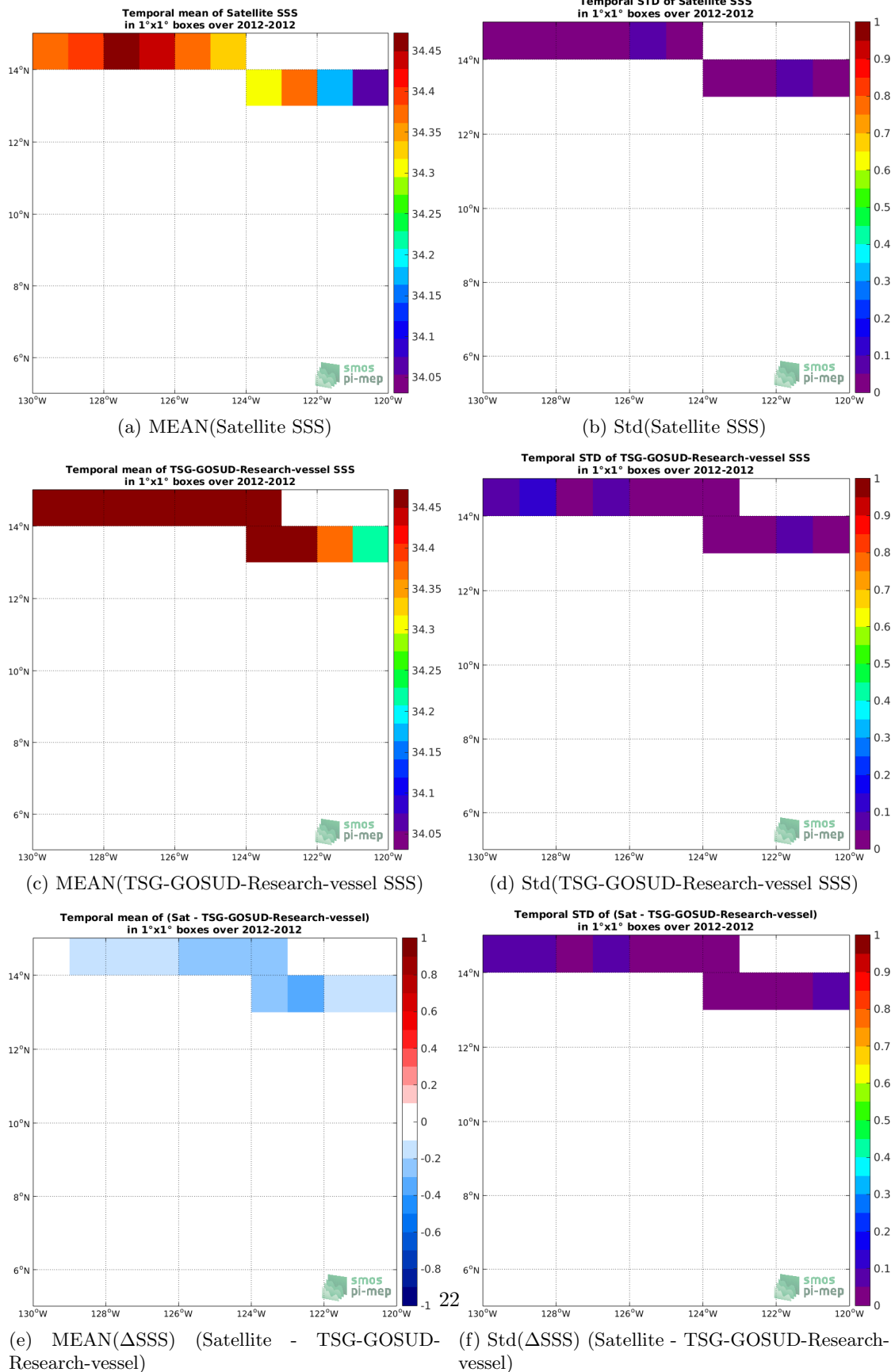
Figure 6: Temporal mean (left) and Std (right) of SSS from CCI L4 Merged-OI v1.8 - 30-day running (ESA) (top), TSG-GOSUD-Research-vessel (middle), and of \Delta SSS (Satellite - TSG-GOSUD-Research-vessel). Only match-up pairs are used to generate these maps.
