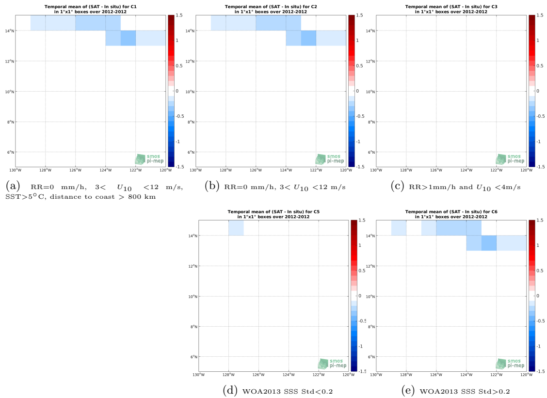
Figure 12: Temporal mean gridded over spatial boxes of size 1^\circ \times 1^\circ of \Delta SSS (CCI L4 Merged-OI v1.8 - 30-day running (ESA) - TSG-GOSUD-Research-vessel) for 5 different subdatasets corresponding to: RR=0 mm/h, 3 < U_{10} < 12 m/s, SST>5°C, distance to coast > 800 km (a), RR=0 mm/h, 3 < U_{10} < 12 m/s (b), RR>1mm/h and U_{10} < 4 m/s (c), WOA2013 SSS Std<0.2 (d), WOA2013 SSS Std>0.2 (e).
